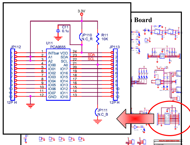
Figure 18. PCA9555 Schematic
