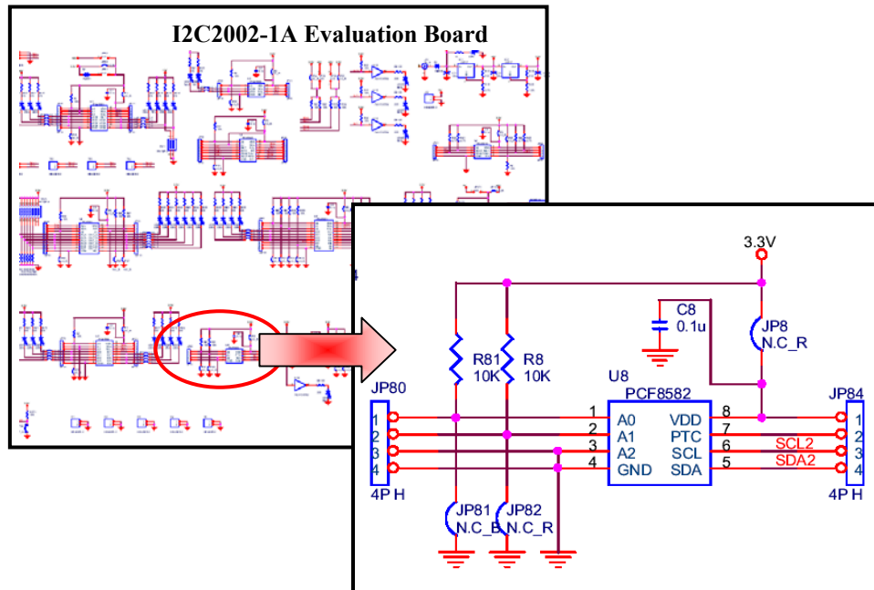
Figure 23. PCF8582C-2 Schematic
