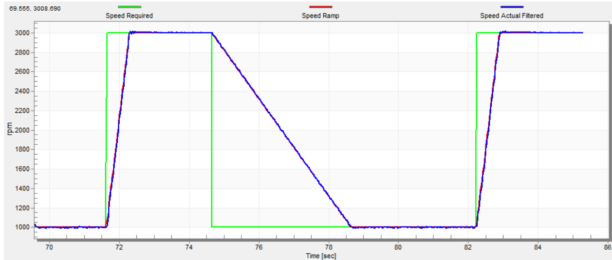
Figure 30. Speed profile
