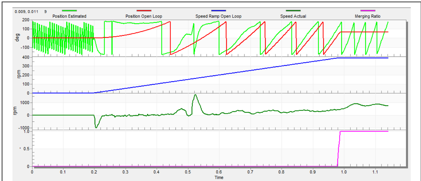
Figure 31. Motor startup
