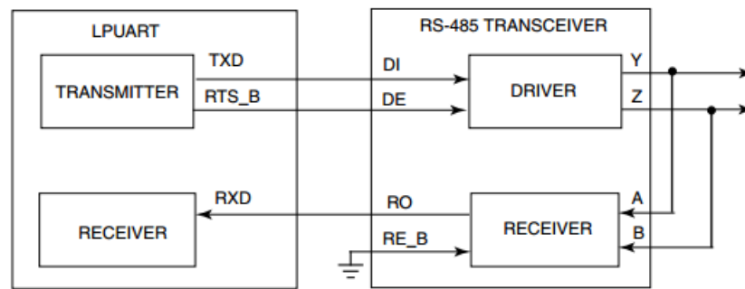
Figure 3. Transceiver driver enable using RTS_B
