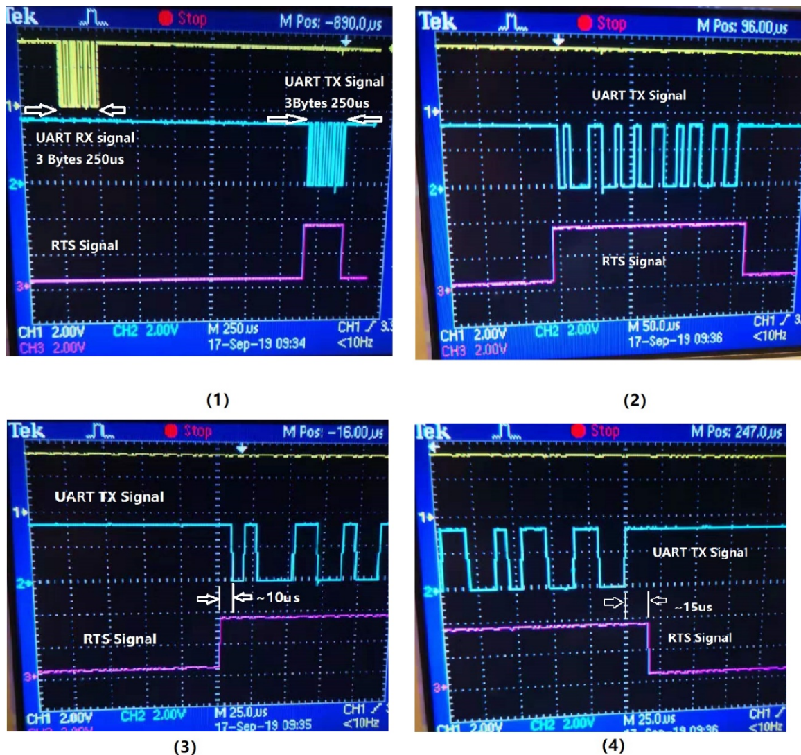
Figure 15. Timing Wave using RTS control
