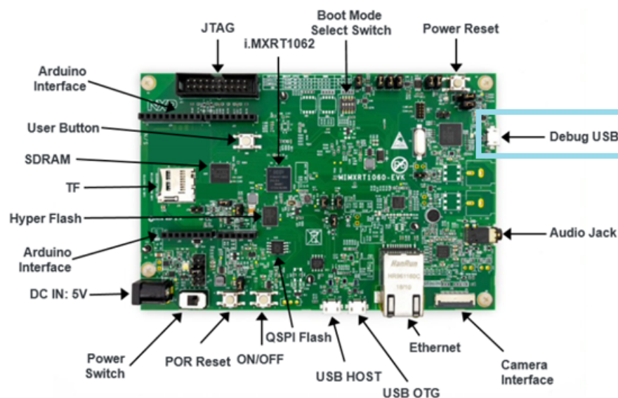
Figure 2. Overview of the MIMXRT1060 EVK board (Front side)
