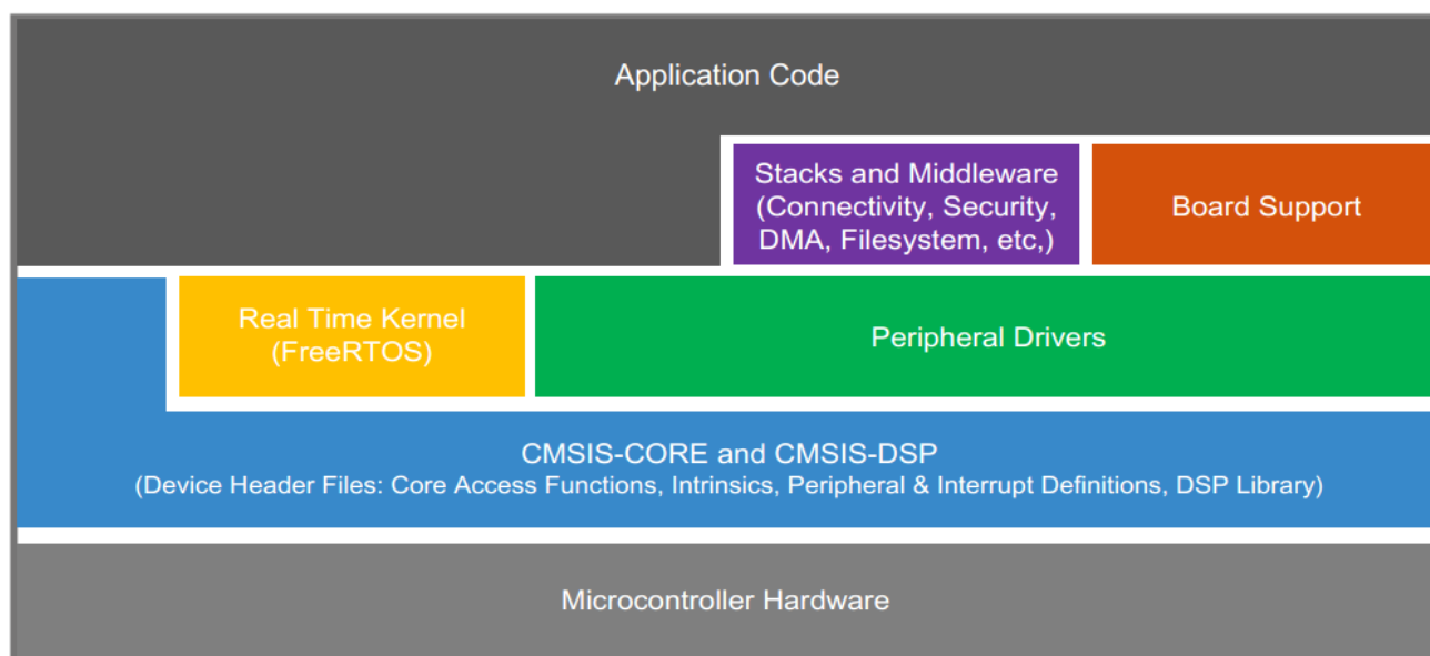
Figure 8. MCUXpresso SDK layers
