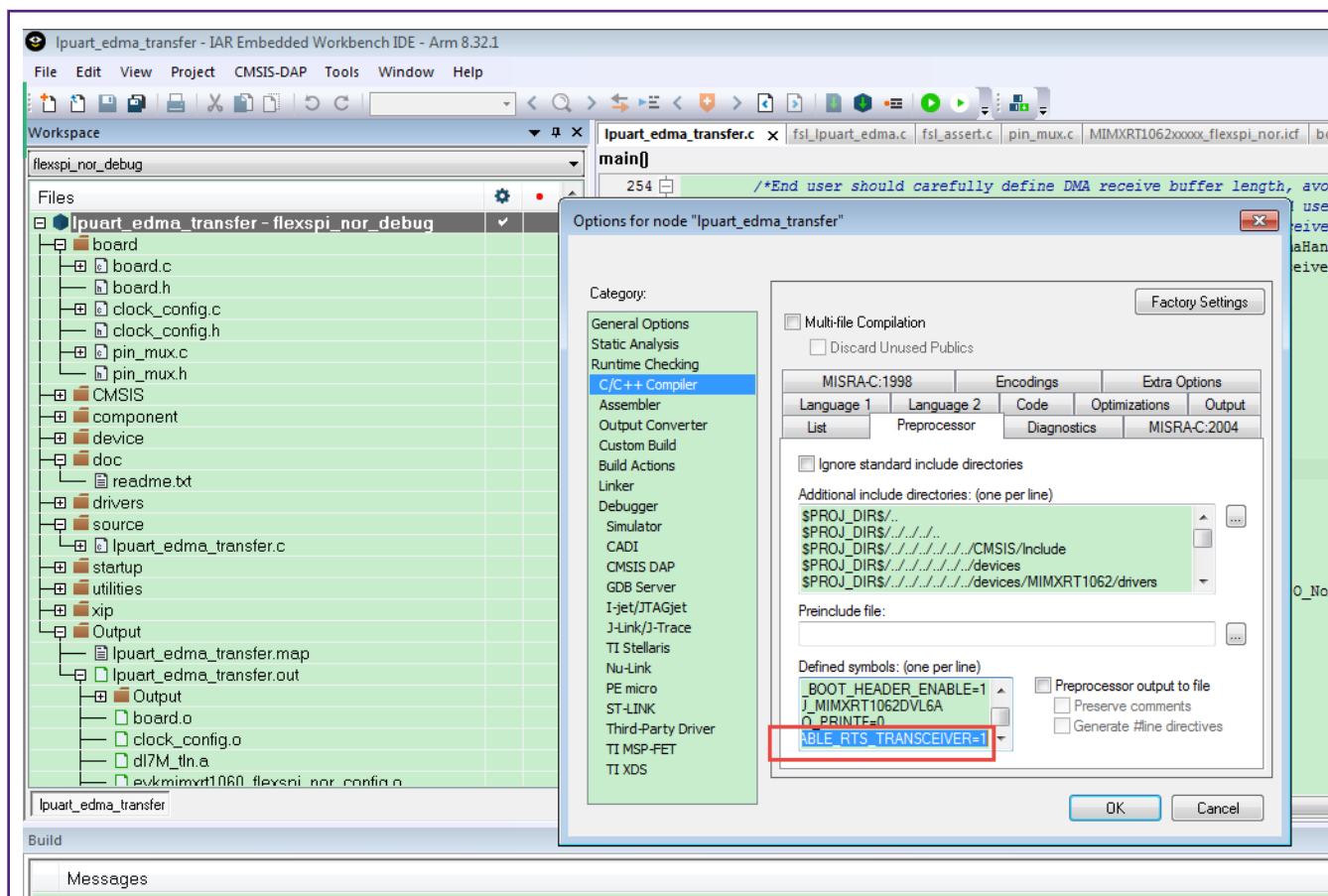
Figure 13. Macro Definition in software package
