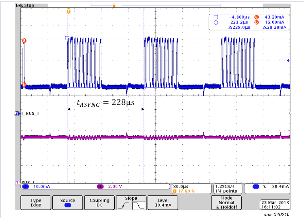
Figure 14. PSI5 response time using asynchronous mode
