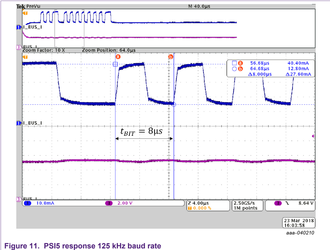
Figure 11. PSI5 response 125 kHz baud rate
