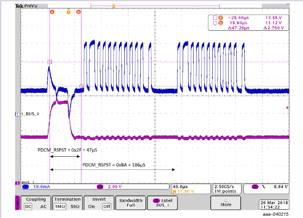
Figure 13. PSI5 PDCM start time response
