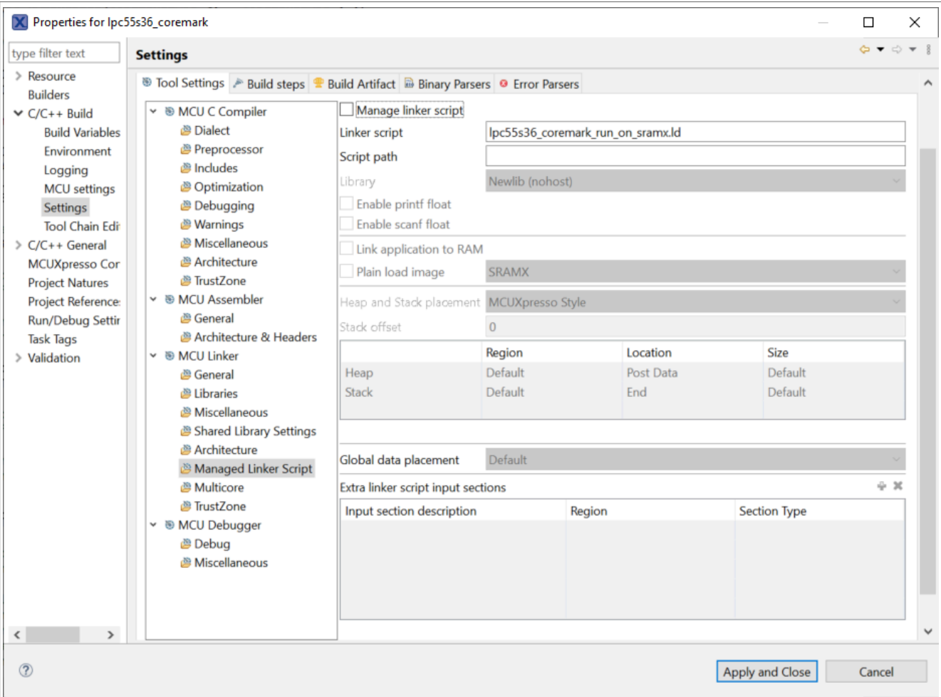
Figure 14. MCUXpresso allocate code to SRAM area
