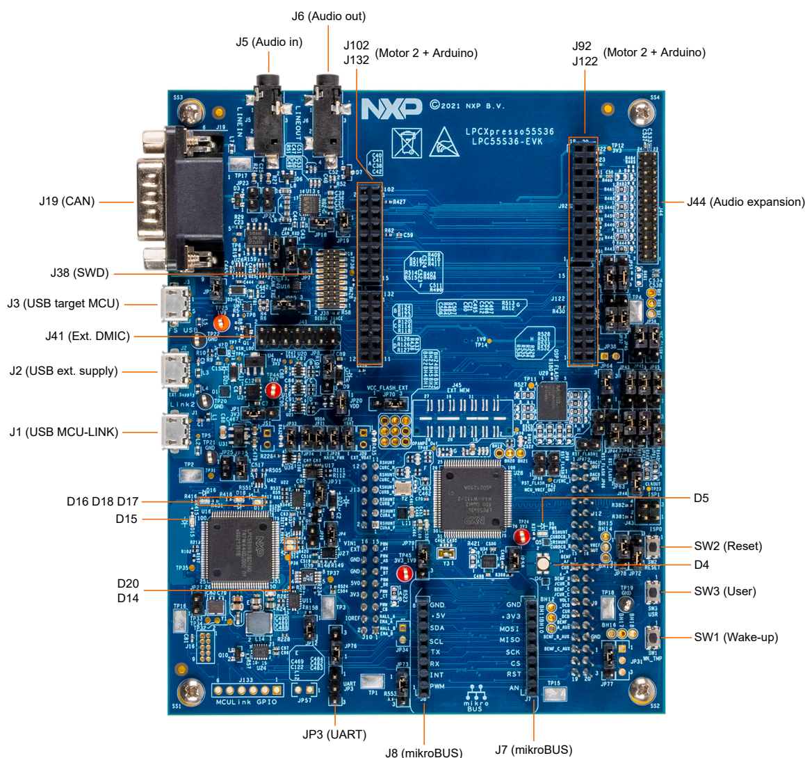
Figure 19. LPCXpresso55S36 development board
