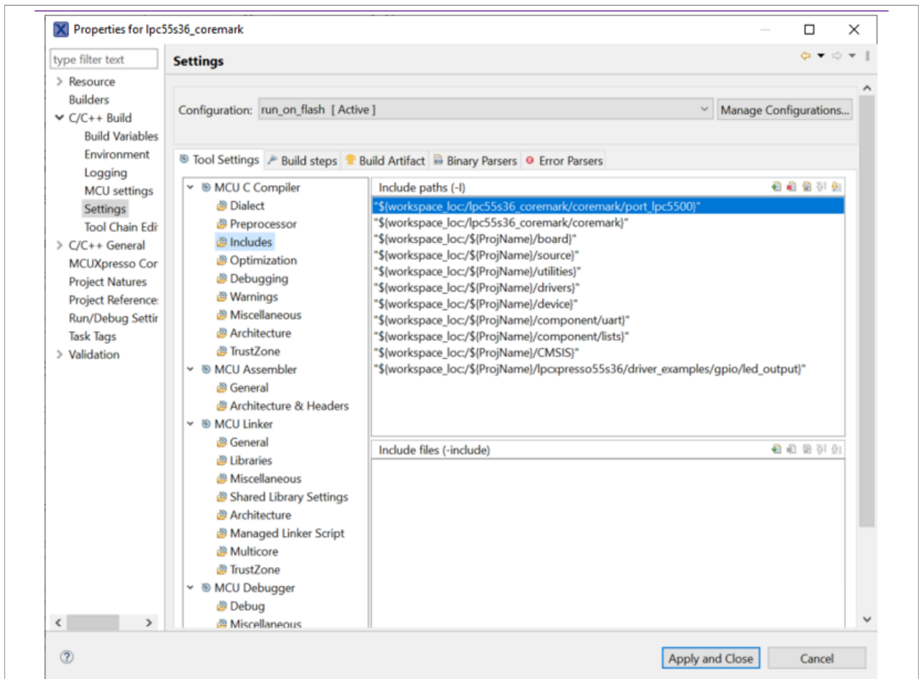
Figure 11. MCUXpresso compiler include paths
