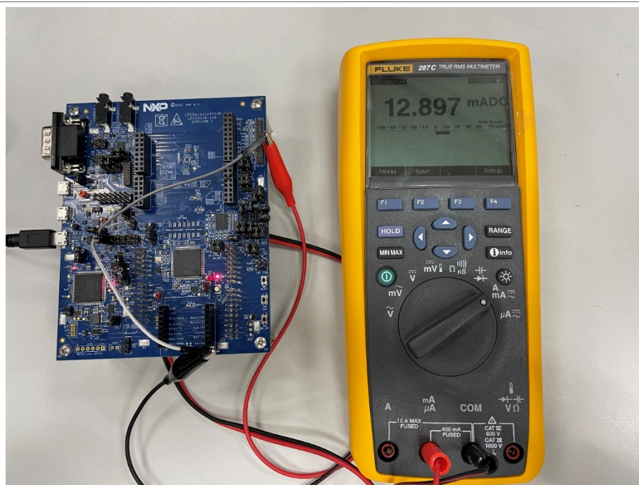
Figure 20. \mu\text{A}/\text{MHz} measurement setup
