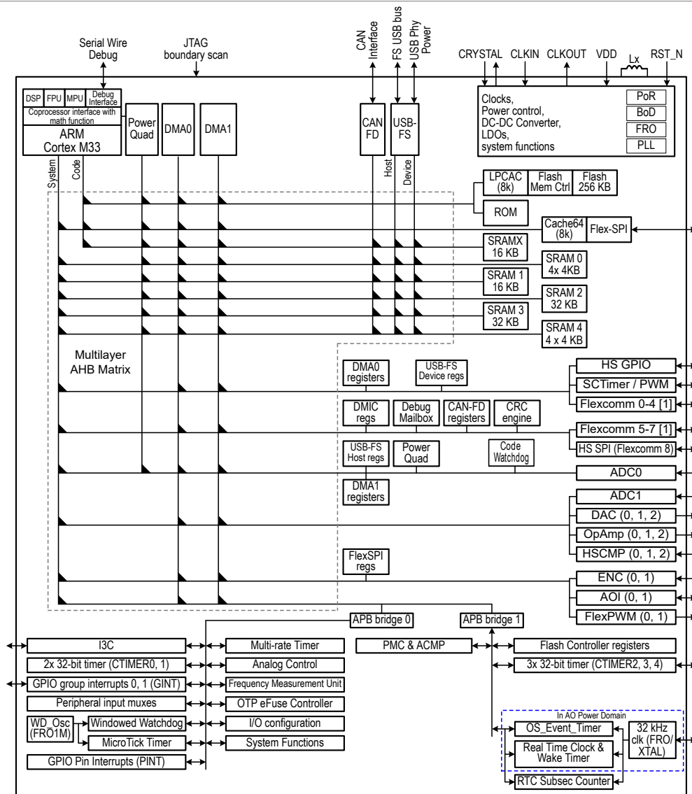
Figure 15. LPC553x/LPC55S3x AHB matrix
