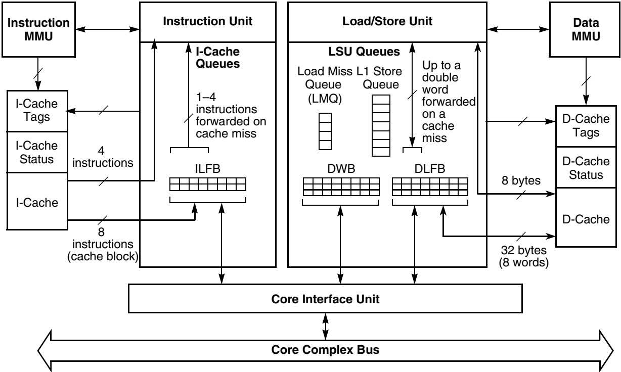
Figure 12-2. Cache/Core Interface Unit Integration
