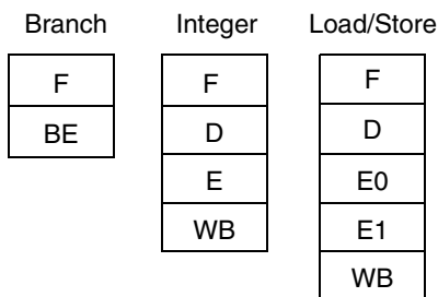
Figure 1-1. MPC 603e and MPC755 Pipeline Diagram
