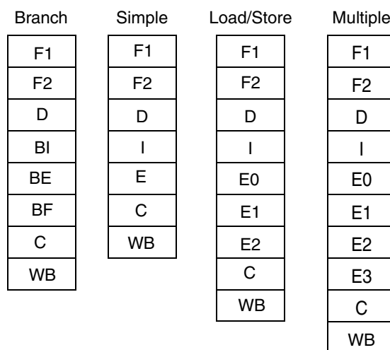
Figure 1-3. e500 Core Pipeline Diagram
