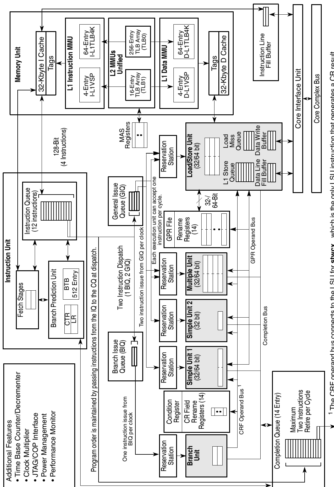
Figure 2-1. Functional Block Diagram
