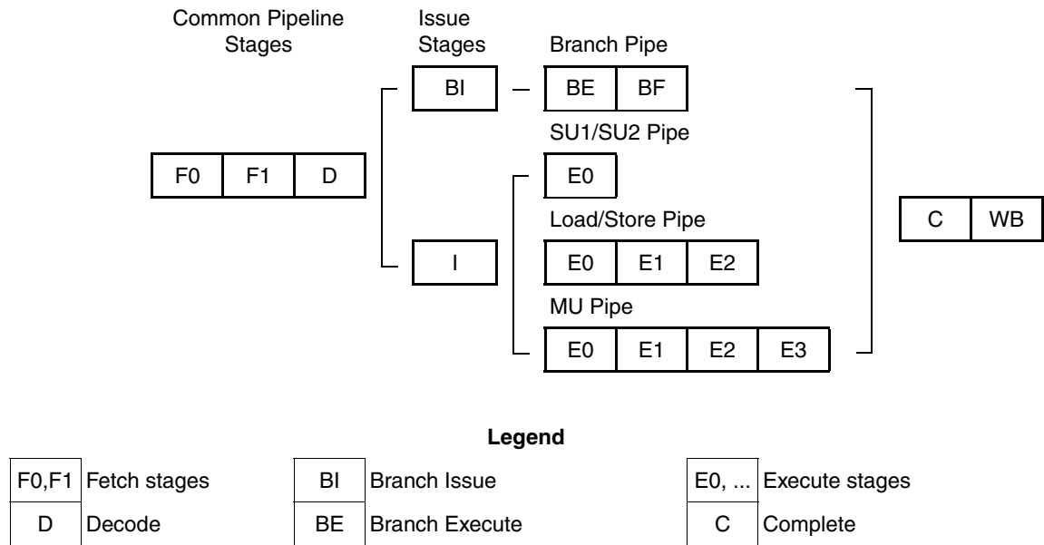
Figure 3-1. Pipeline Diagram of the e500 Core
