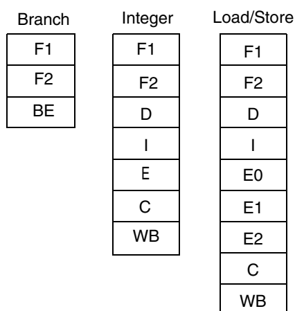
Figure 1-2. MPC745x Pipeline Diagram
