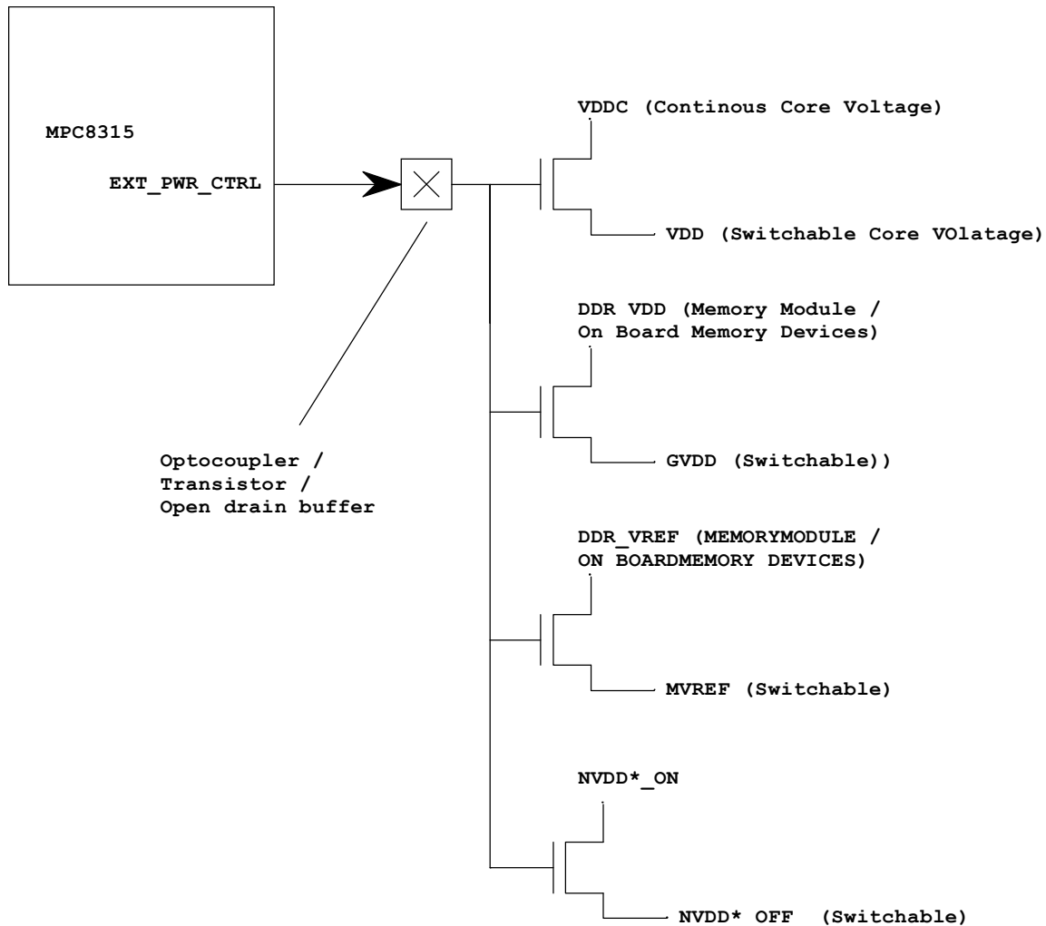
Figure 27. I/O Switching
