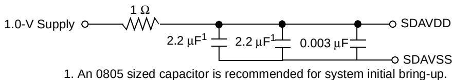
Figure 3. SerDes PLL Power Supply Filter Circuit
