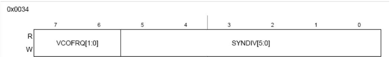
Figure 5. SYN/CPMUSYN Register
