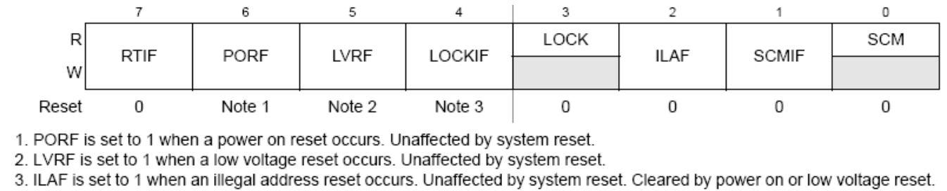
Figure 10. CRG Flags Register (CRGFLG)
