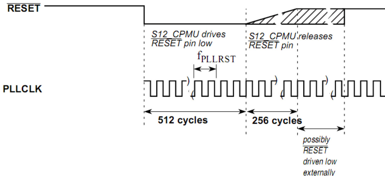
Figure 4. Reset Timing on the S12P
