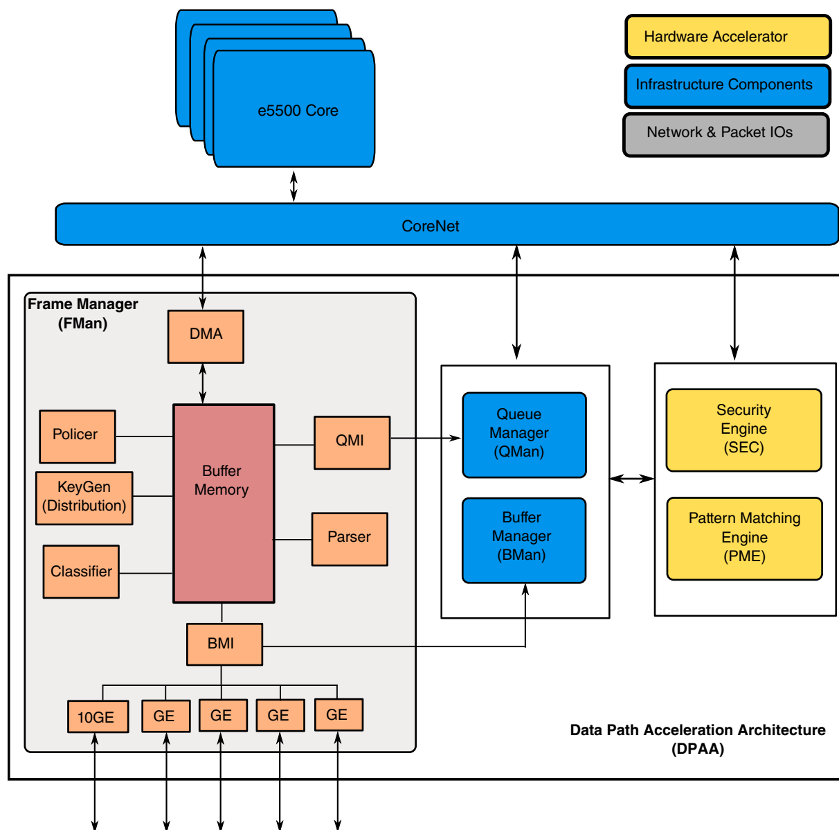
Figure 1. DPAA block diagram
