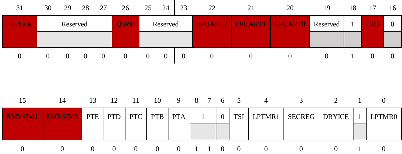
Figure 5. System Clock Gating Control Register 5 (SIM_SCGC5)
