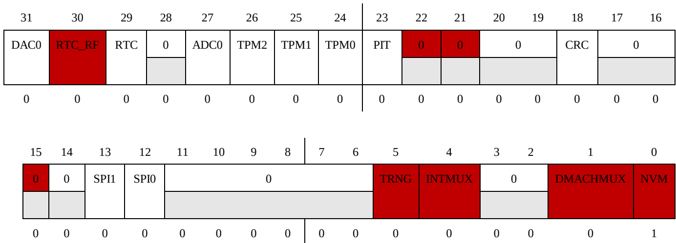
Figure 4. System Clock Gating Control Register 6 (SIM_SCGC6)
