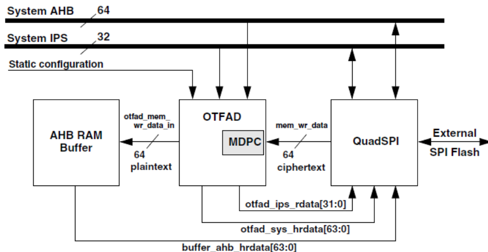
Figure 16. K80 150 MHz OTFAD and QuadSPI connection topology
