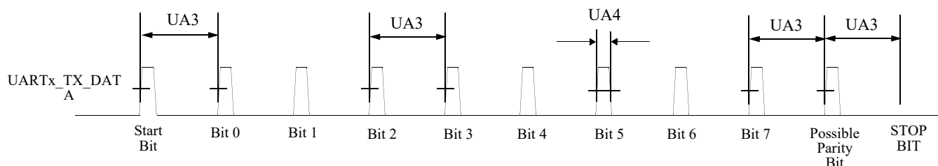
Figure 76. UART IrDA Mode Transmit Timing Diagram
