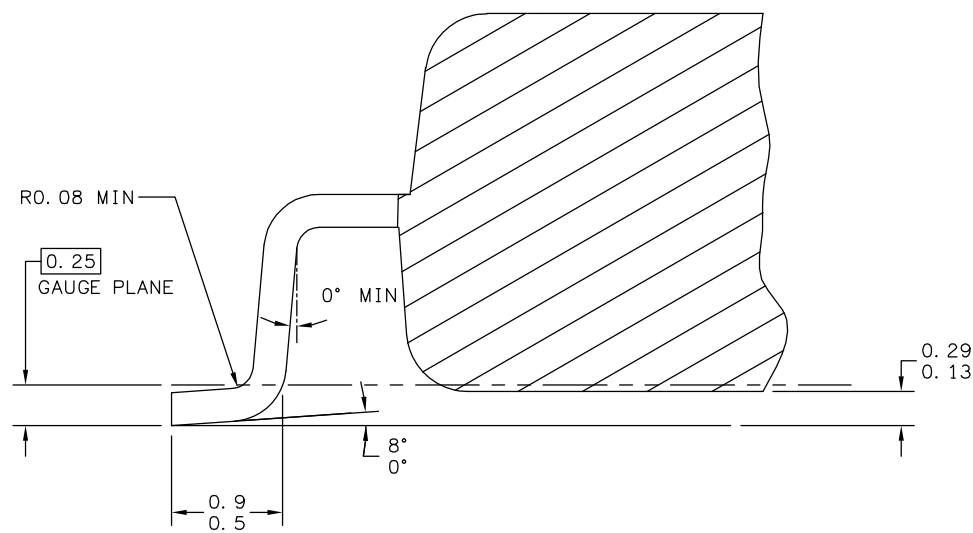
SECTION B-B
