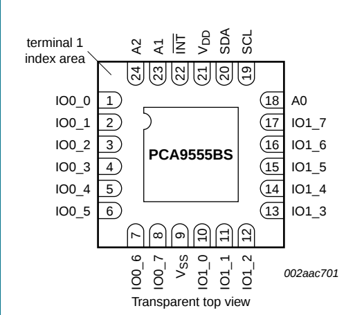
Fig 5. Pin configuration for HVQFN24
