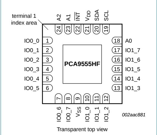
Fig 6. Pin configuration for HWQFN24
