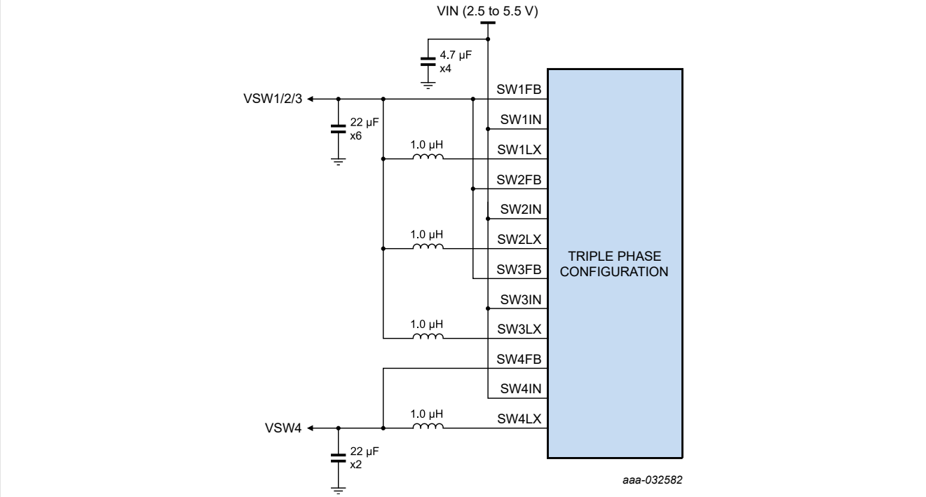
Figure 26. Triple phase configuration
