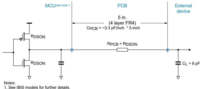
Figure 35. Reference Load Diagram
