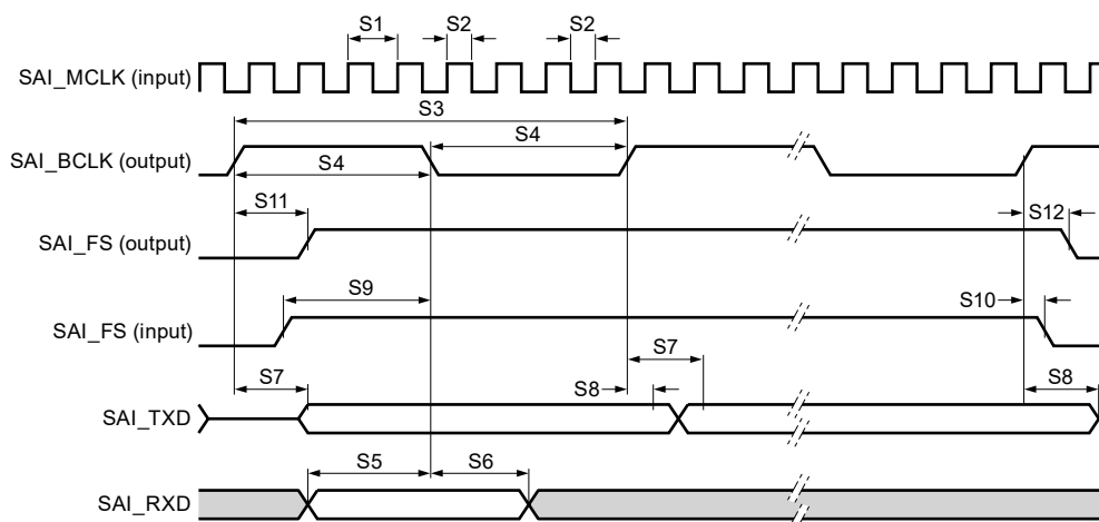
Figure 51. SAI controller mode
