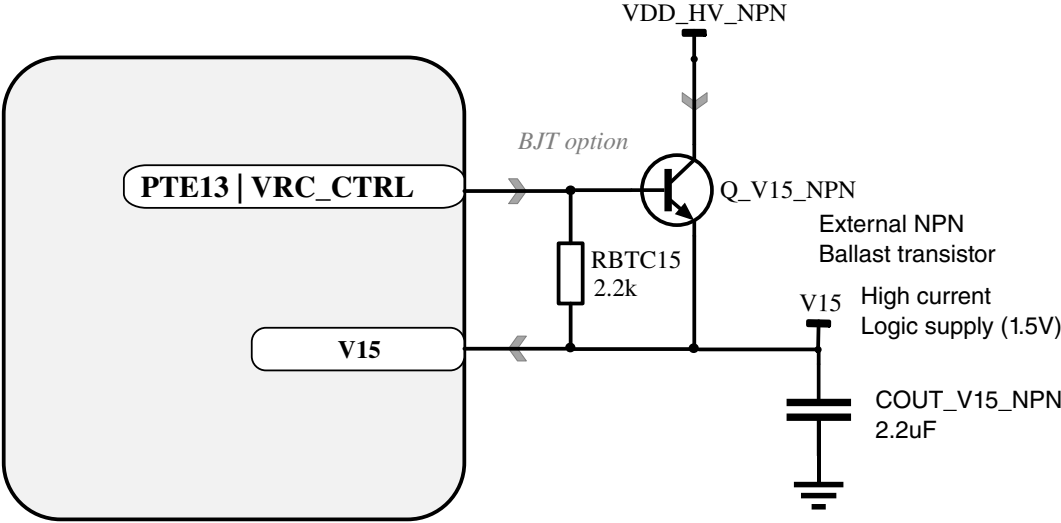
Figure 32. Ballast circuit
