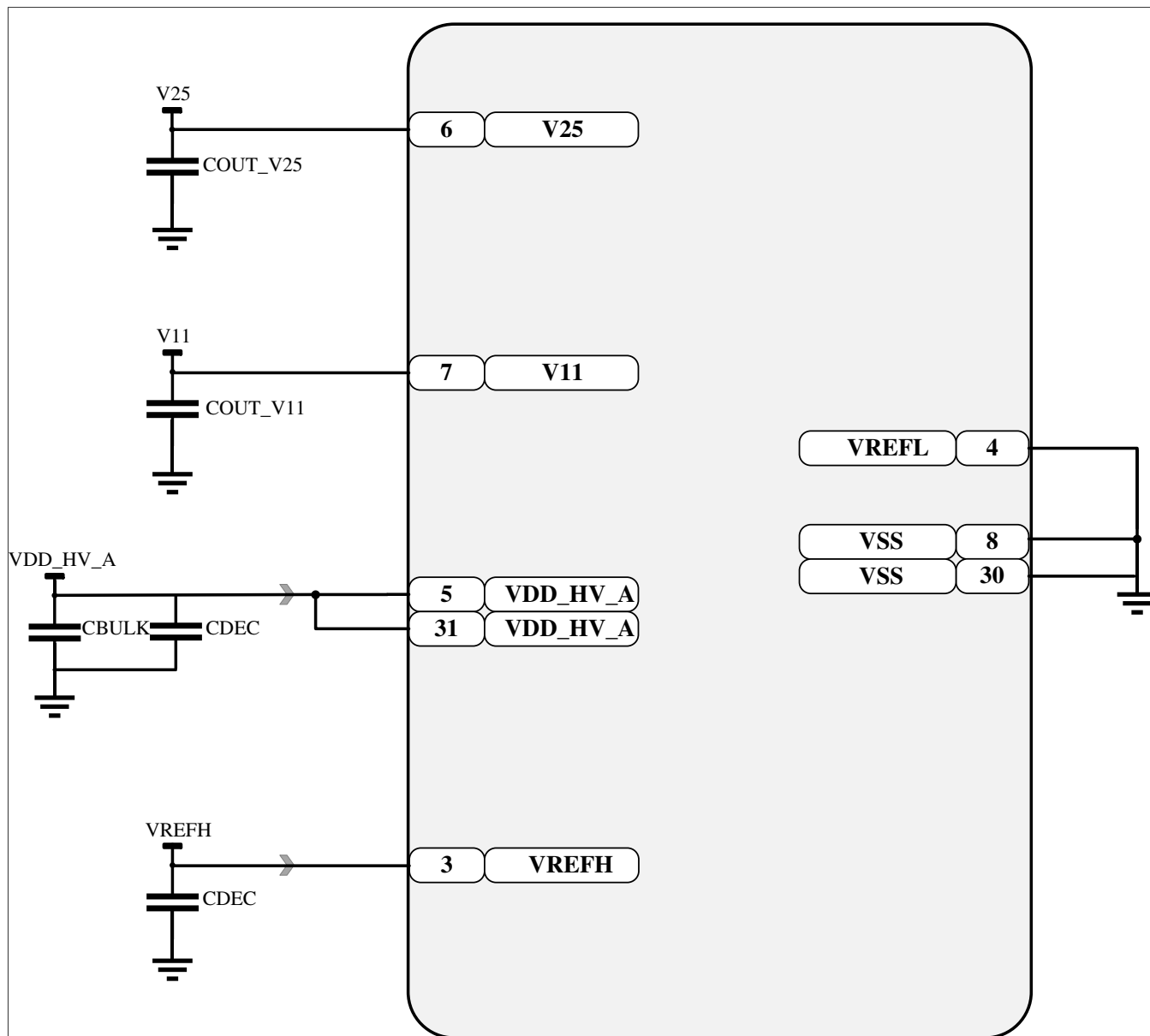
Figure 17. 48-pin LQFP decoupling capacitor pinout diagram (S32K311, S32K310)
