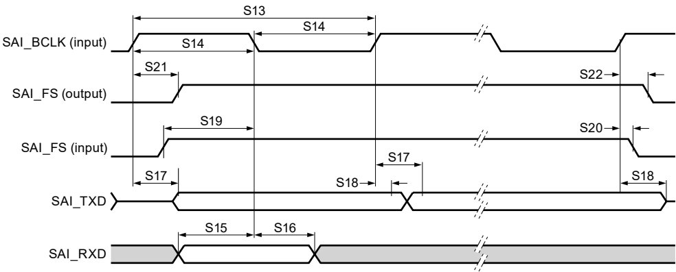
Figure 50. SAI target mode
