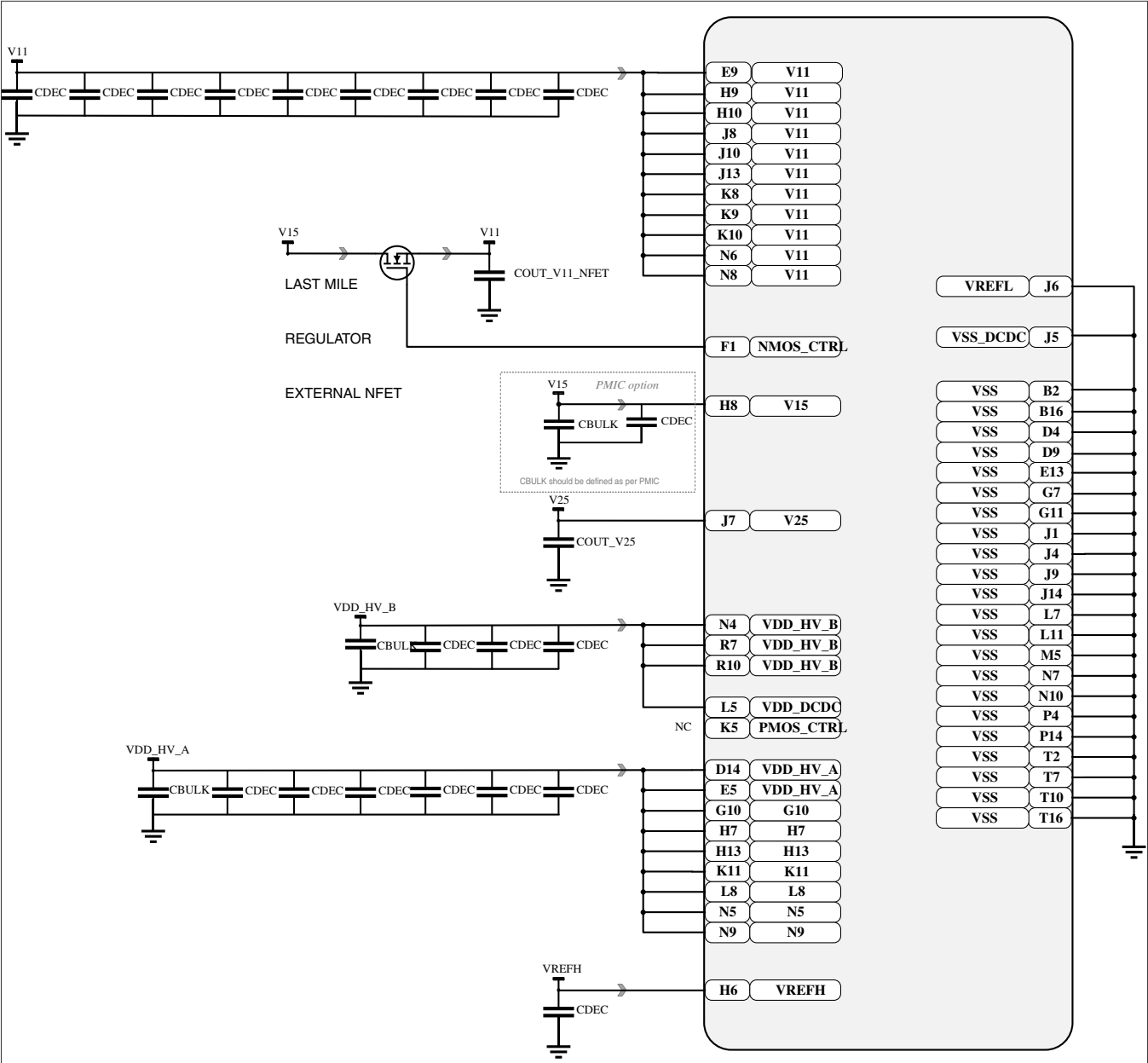
Figure 27. 289BGA package decoupling capacitor pinout diagram, (S32K388)
