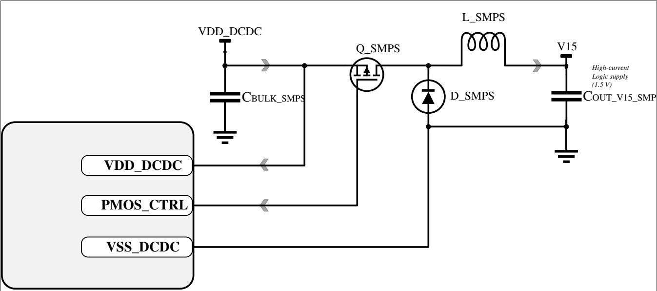
Figure 31. SMPS circuit
