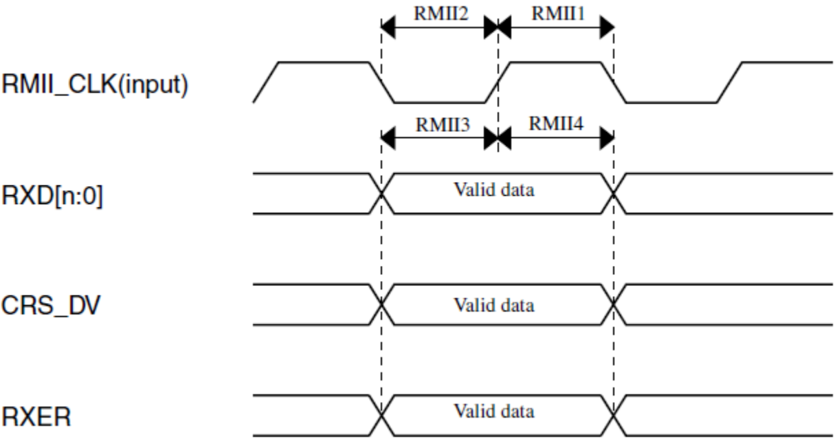
Figure 56. RMI receive diagram
