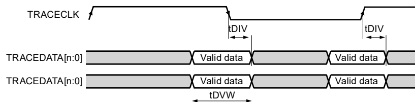
Figure 65. Trace CLKOUT specifications
