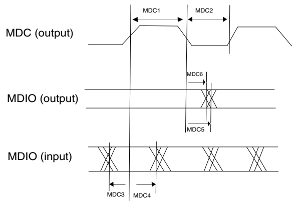
Figure 60. MII/RMII serial management channel timing
