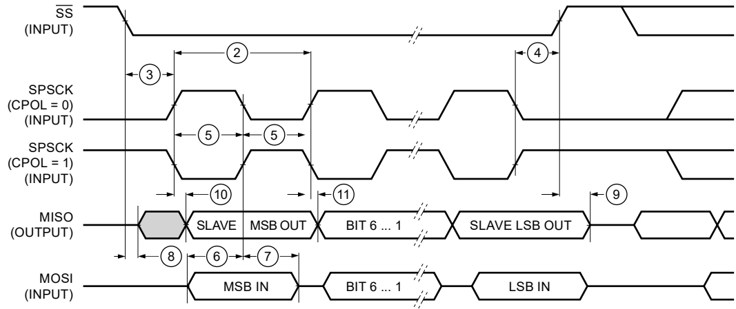
Figure 45. LPSPI Peripheral Mode Timing (CPHA=1)
