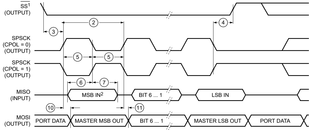
Figure 48. LPSPi Controller Mode Timing (CPHA=1)
