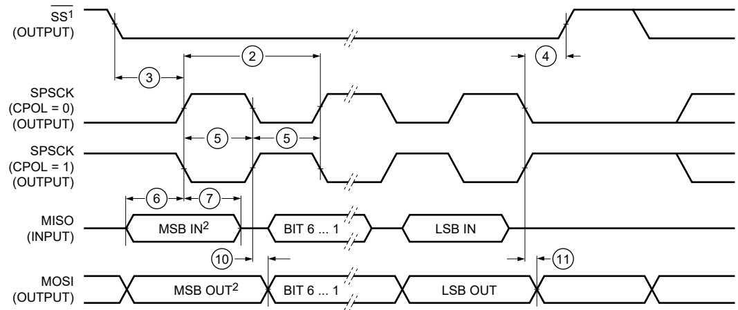
Figure 47. LPSPI Controller Mode Timing (CPHA=0)
