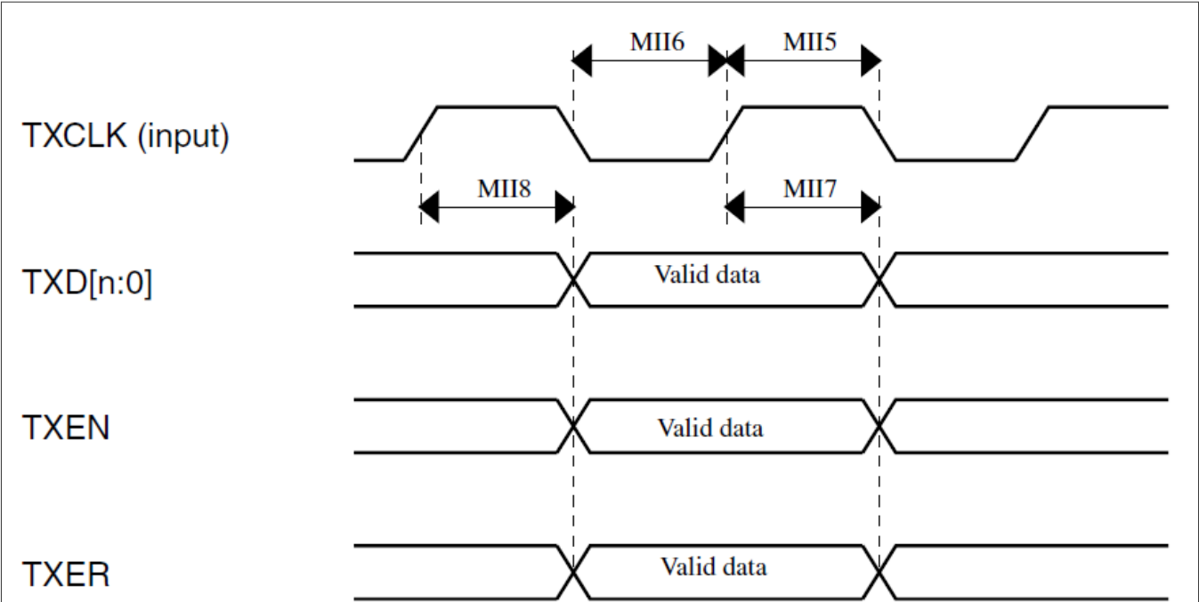
Figure 53. MII transmit diagram
