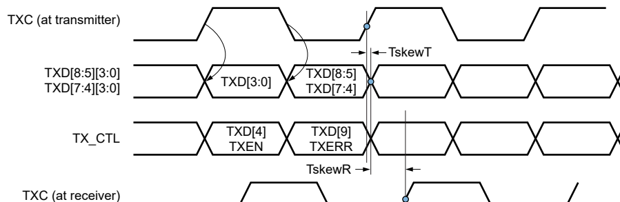
Figure 59. RGMII Transmit Timing
