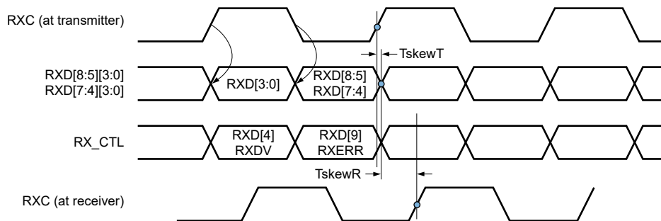
Figure 58. RGMII Receive Timing
