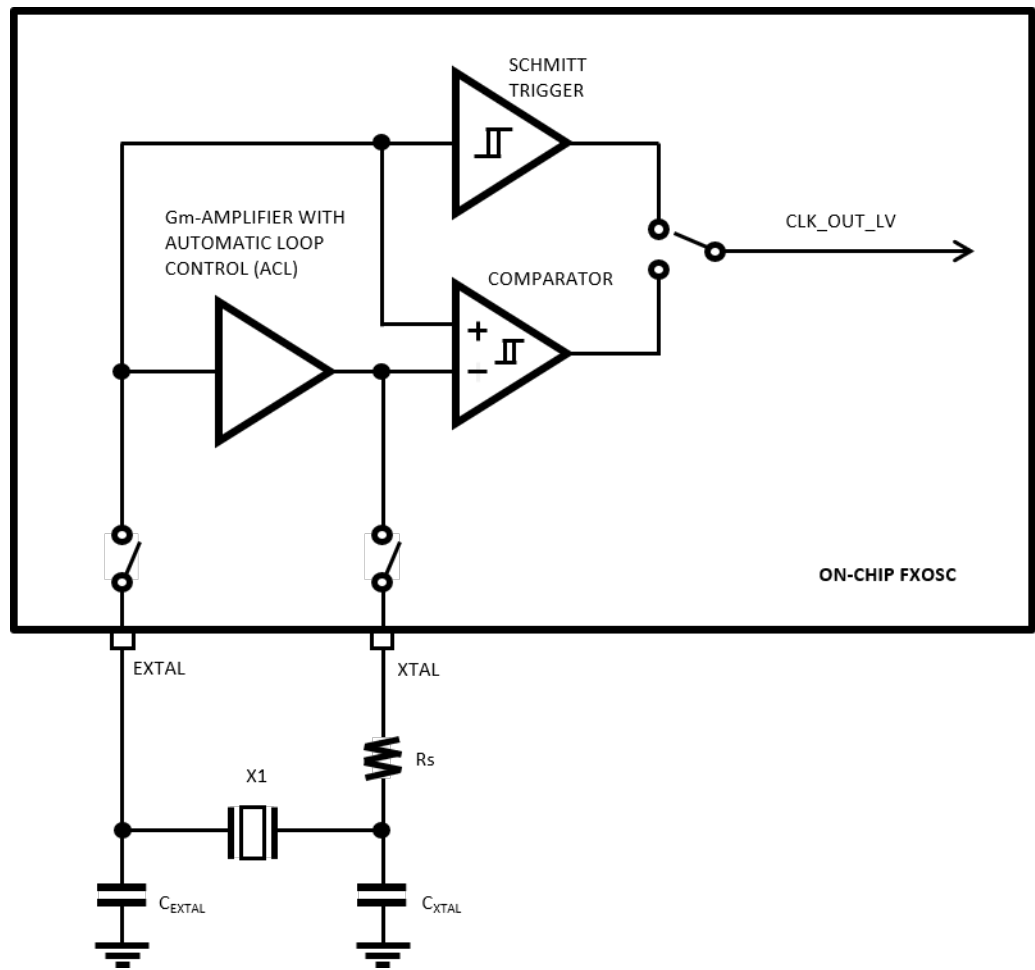
Figure 44. Block diagram
