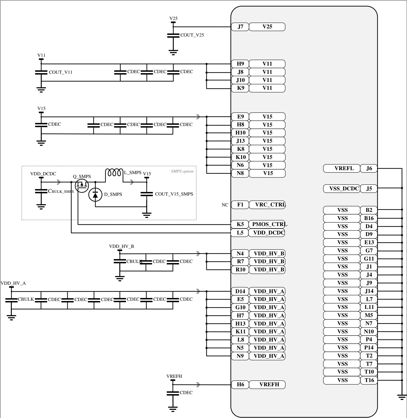
Figure 26. 289BGA package decoupling capacitor pinout diagram, SMPS (S32K358, S32K348, S32K338 and S32K328)
