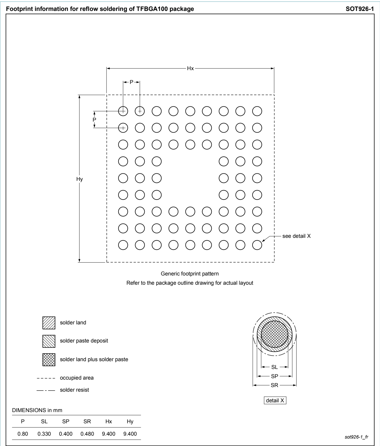
Fig. 2. Reflow soldering footprint for TFBGA100 (SOT926-1)
