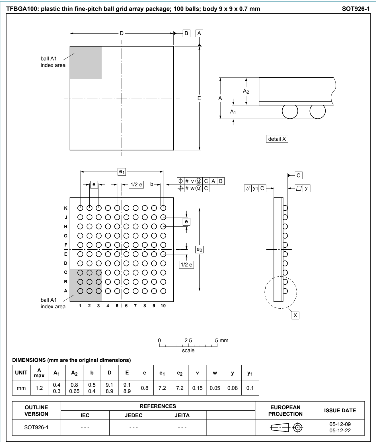
Fig. 1. Package outline TFBGA100 (SOT926-1)
