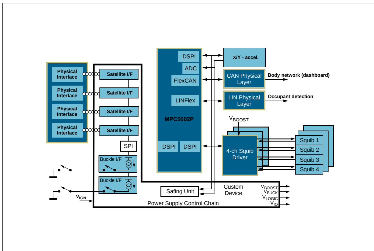
Figure 3. Airbag application
