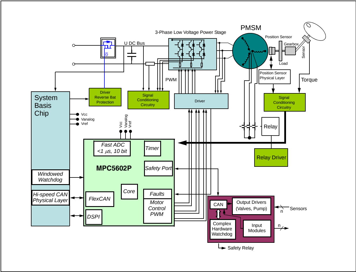
Figure 2. Electric power steering application
