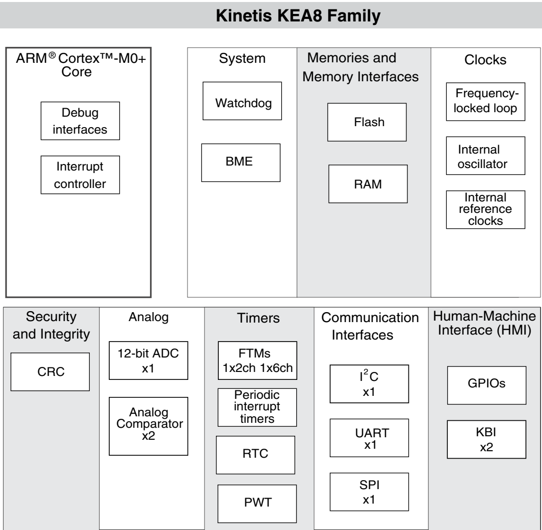
Figure 1. KEA8 family block diagram
