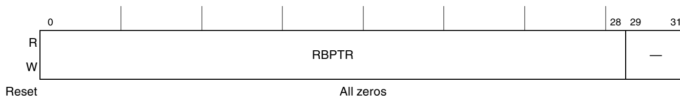
Figure 15-33. RBPTR Register Definition
