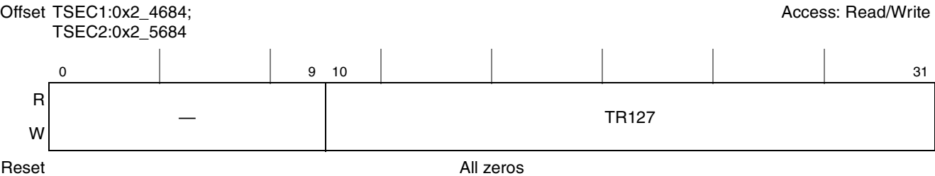
Figure 15-50. Transmit and Receive 65- to 127-Byte Frame Register Definition
