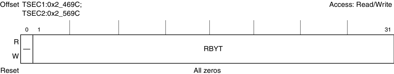
Figure 15-56. Receive Byte Counter Register Definition
