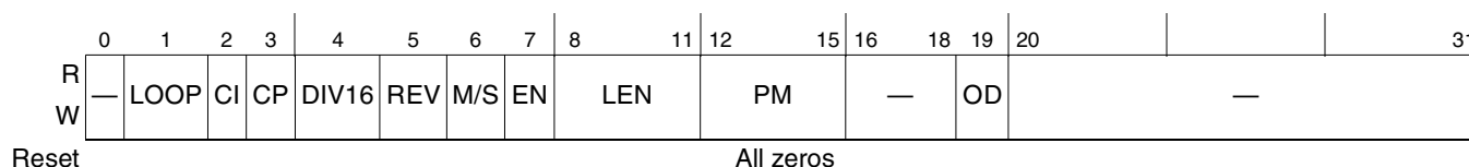
Figure 19-4. SPMODE-SPI Mode Register
