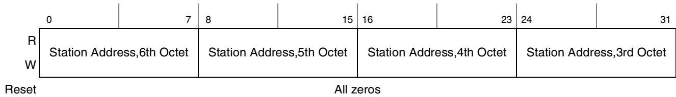
Figure 15-47. MACSTNADDR1 Register Definition
