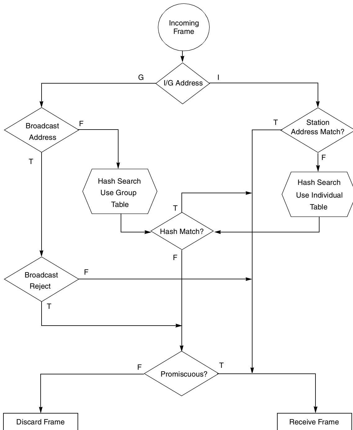
Figure 15-114. Ethernet Address Recognition Flowchart
