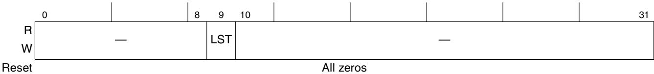
Figure 19-9. SPI Command Register (SPCOM)
