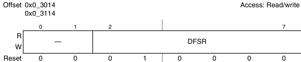
Figure 17-7. I 2 Cn Digital Filter Sampling Rate Register (I2CnDFSRR)
