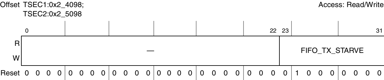
Figure 15-16. FIFO_TX_STARVE Register Definition
