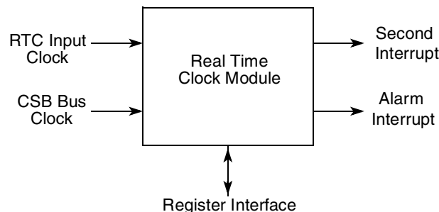
Figure 5-24. Real Time Clock Module High Level Block Diagram
