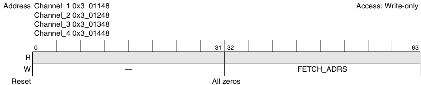
Figure 14-64. Fetch FIFO
