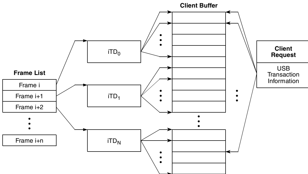
Figure 16-50. Example Association of iTDs to Client Request Buffer
