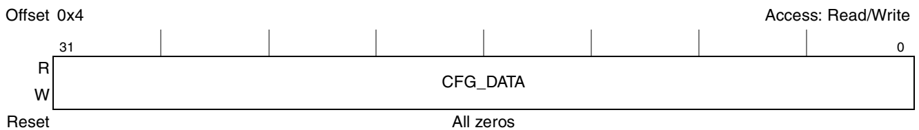
Figure 13-4. PCI_CONFIG_DATA
