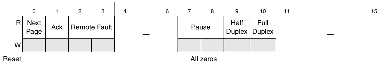
Figure 15-102. AN Link Partner Base Page Ability Register Definition
