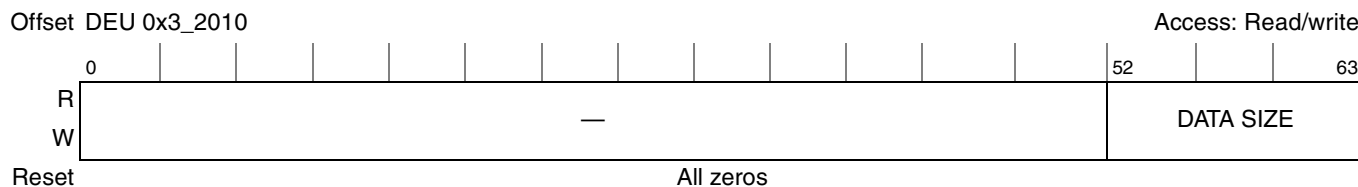
Figure 14-19. DEU Data Size Register (DEUDSR)
