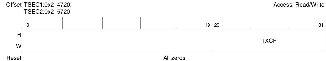
Figure 15-88. Transmit Control Frame Counter Register Definition
