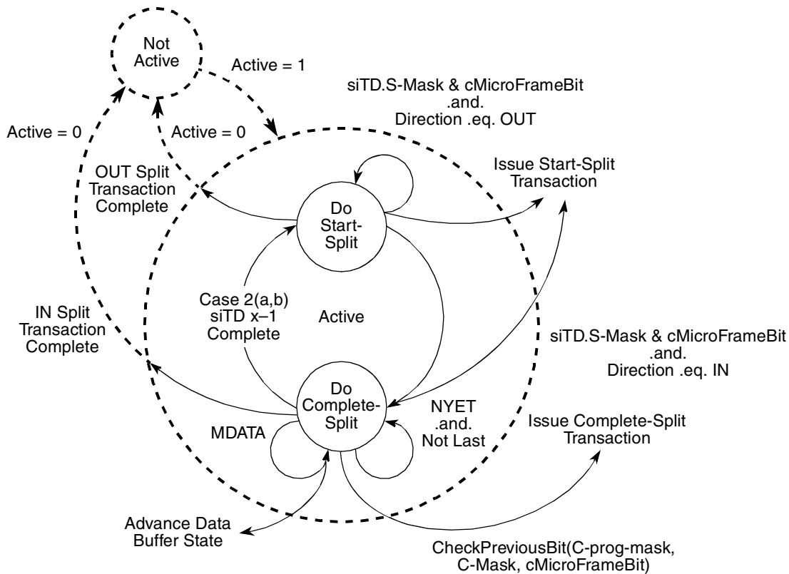
Figure 16-61. Split Transaction State Machine for Isochronous
