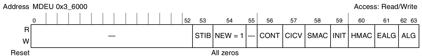
Figure 14-34. MDEU Mode Register (MDEUMR) in ‘New’ Configuration
