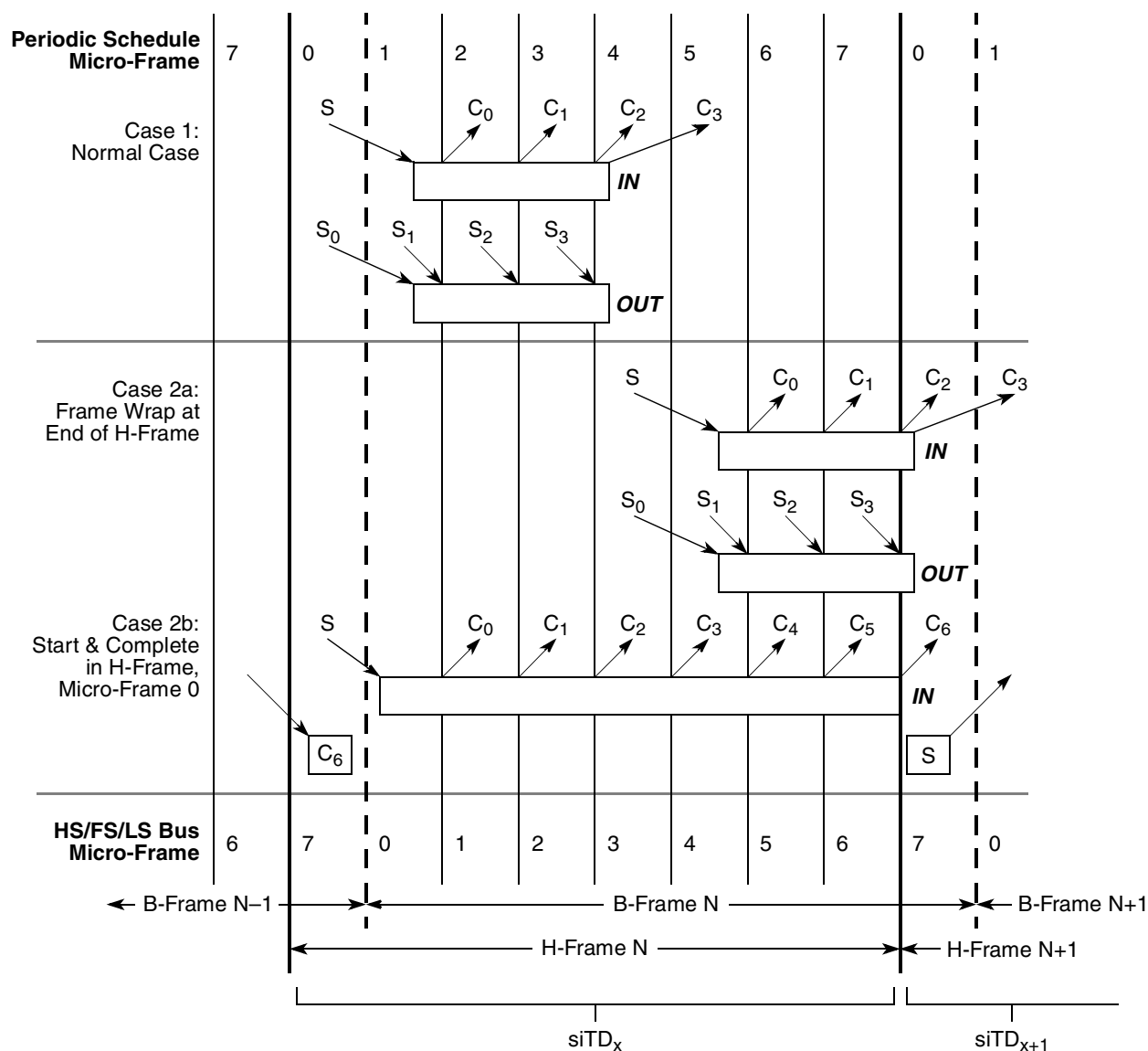
Figure 16-59. Split Transaction, Isochronous Scheduling Boundary Conditions
