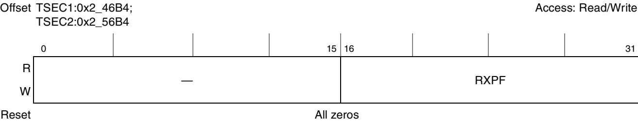
Figure 15-62. Receive Pause Frame Packet Counter Register Definition
