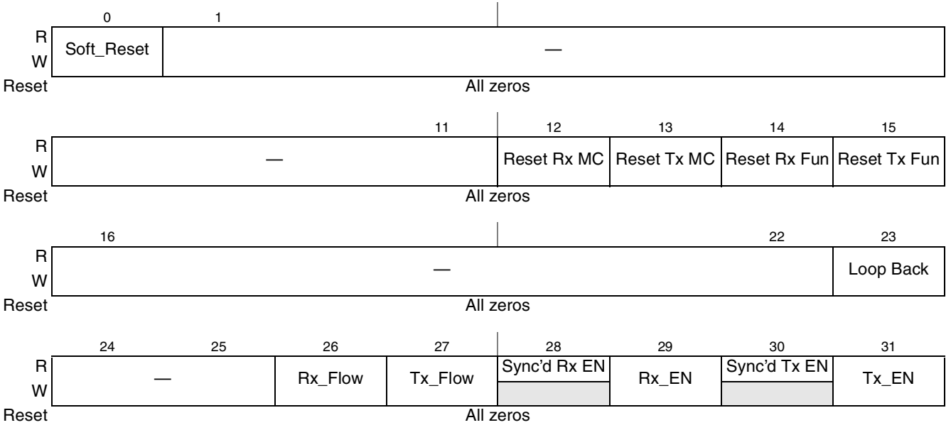
Figure 15-35. MACCFG1 Register Definition
