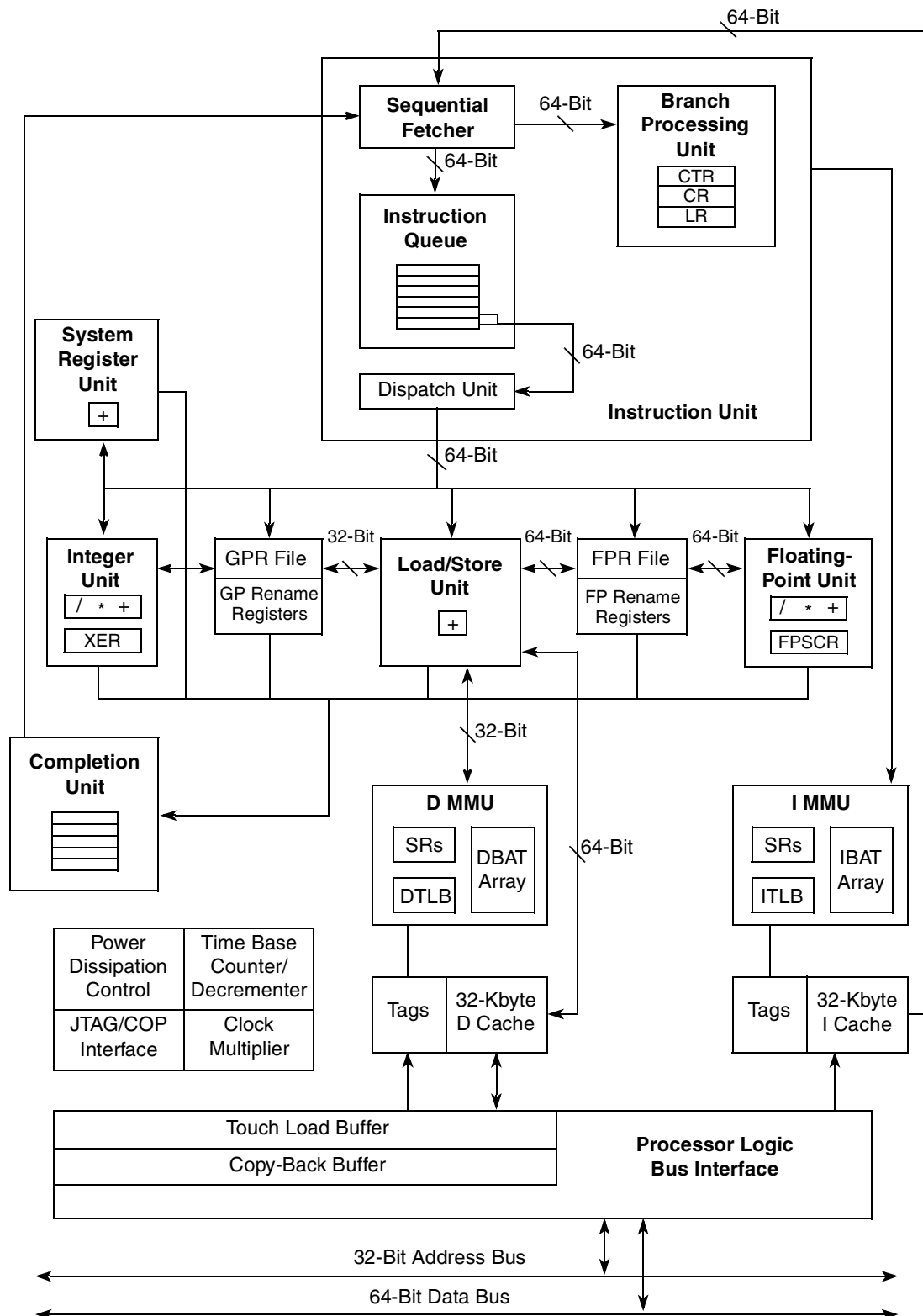
Figure 1-2. MPC8349EA Integrated e300c1 Core Block Diagram
