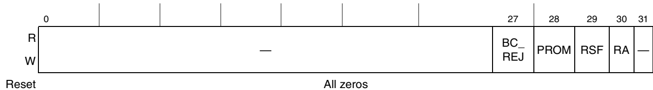
Figure 15-27. RCTRL Register Definition
