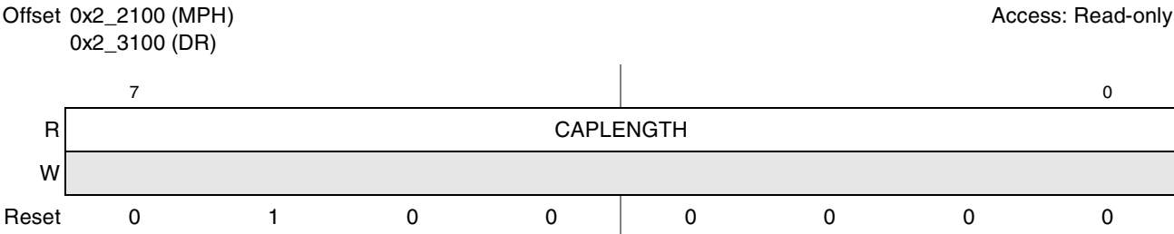
Figure 16-2. Capability Registers Length (CAPLENGTH)
