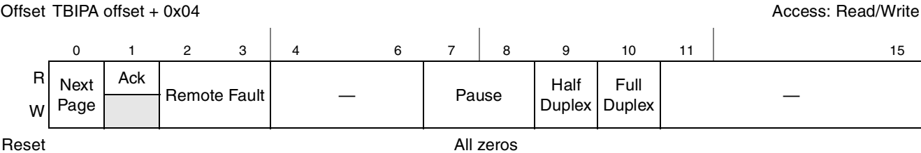
Figure 15-101. AN Advertisement Register Definition
