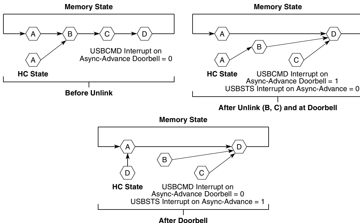
Figure 16-51. Generic Queue Head Unlink Scenario
