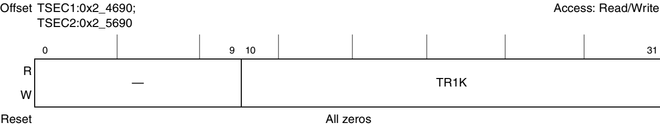
Figure 15-53. Transmit and Received 512- to 1023-Byte Frame Register Definition
