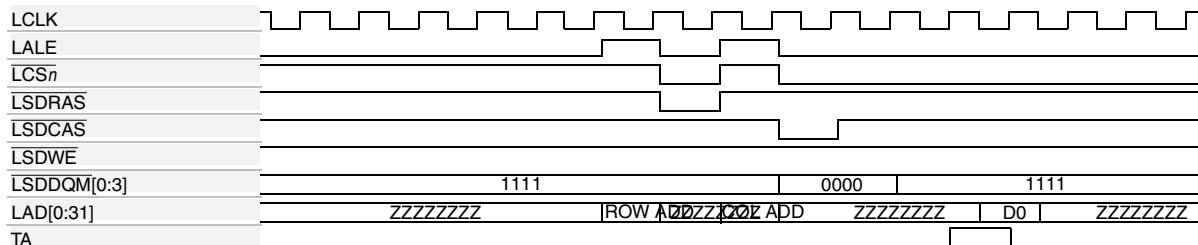
Figure 10-41. SDRAM Single-Beat Read, Page Closed, CL = 3
