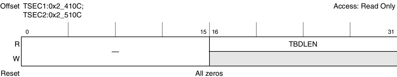
Figure 15-20. TBDLEN Register Definition
