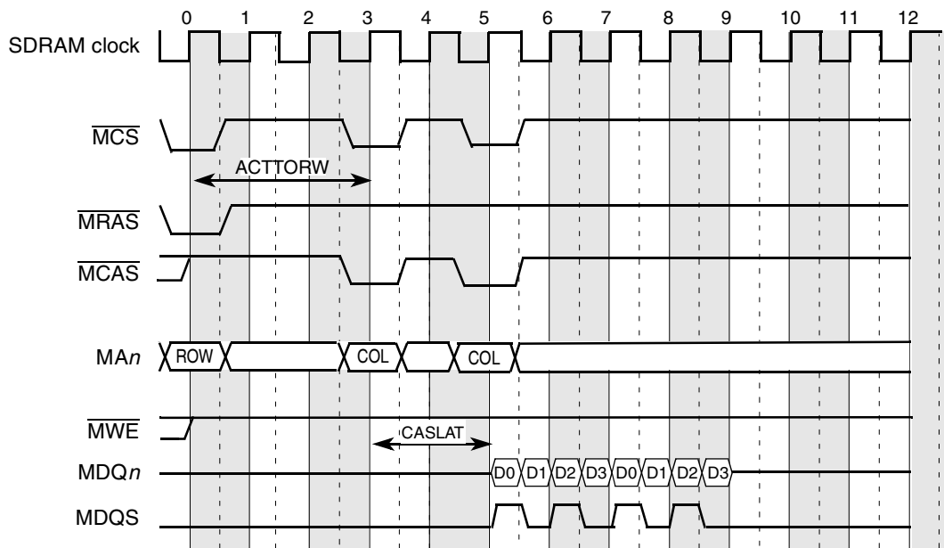
Figure 9-35. DDR SDRAM Burst Read Timing—ACTTORW = 3, MCAS Latency = 2
