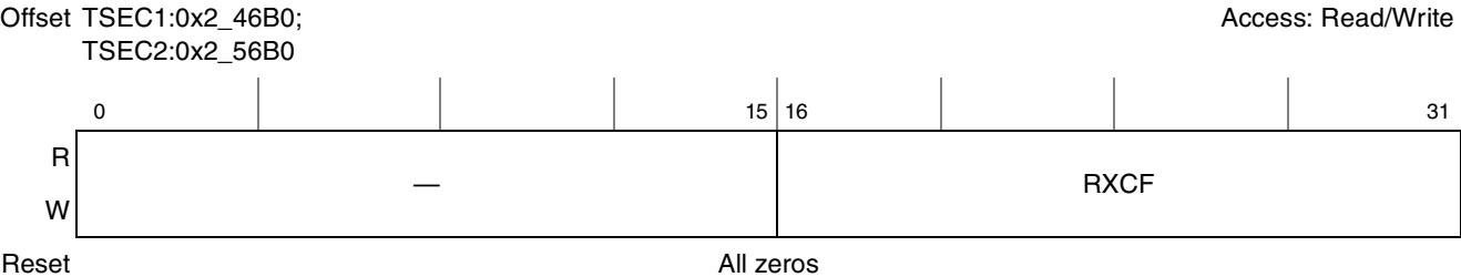
Figure 15-61. Receive Control Frame Packet Counter Register Definition
