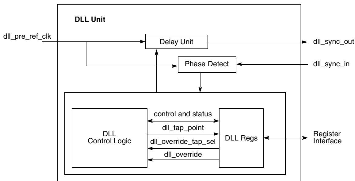
Figure 22-1. DLL Block Diagram
