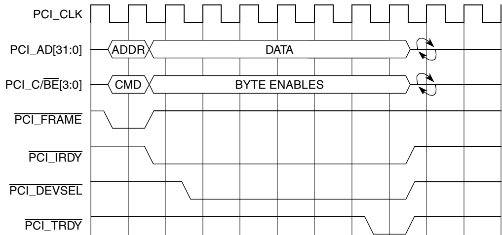
Figure 13-49. Single Beat Write Example
