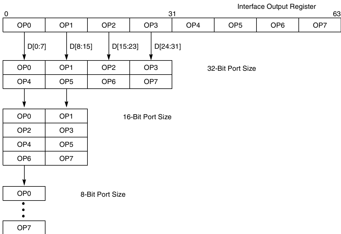
Figure 10-73. Interface to Different Port-Size Devices
