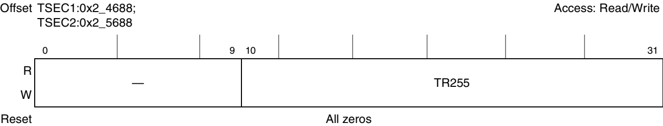
Figure 15-51. Transmit and Received 128- to 255-Byte Frame Register Definition
