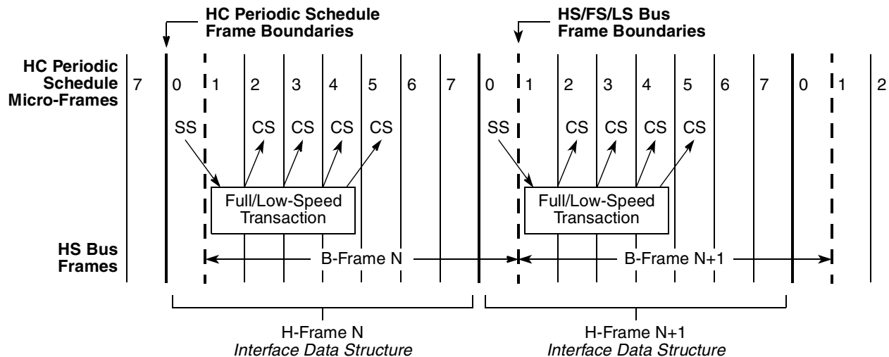
Figure 16-48. Relationship of Periodic Schedule Frame Boundaries to Bus Frame Boundaries
