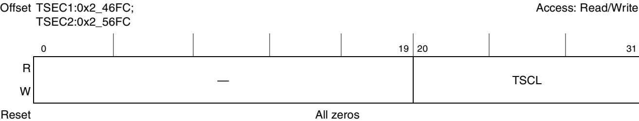
Figure 15-80. Transmit Single Collision Packet Counter Register Definition
