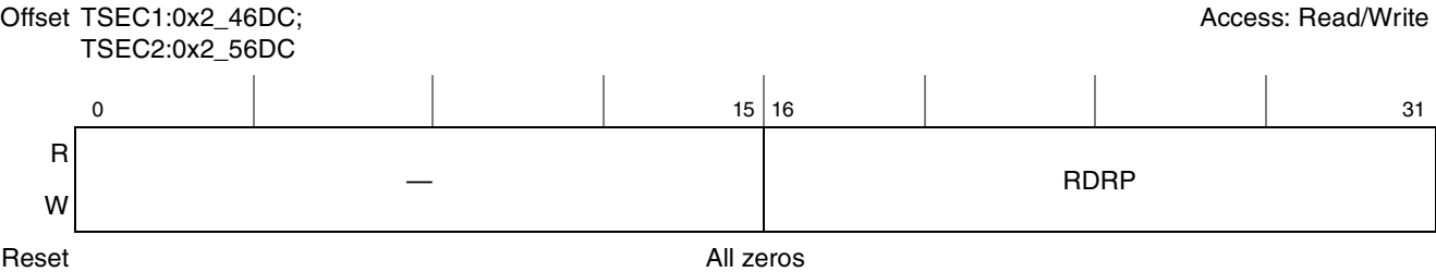
Figure 15-72. Receive Dropped Packet Counter Register Definition
