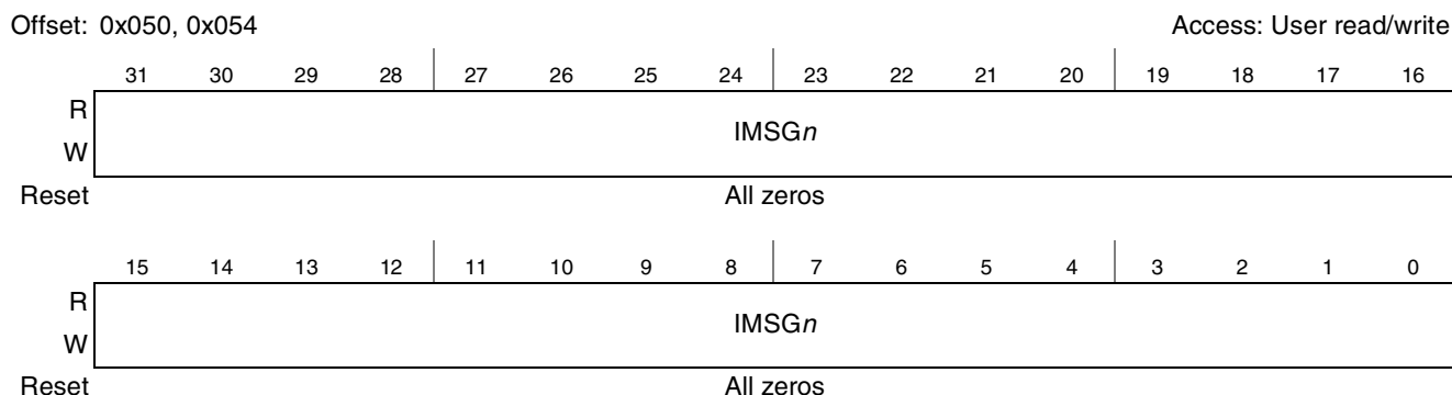
Figure 12-4. Inbound Message Registers (IMR0, IMR1)
