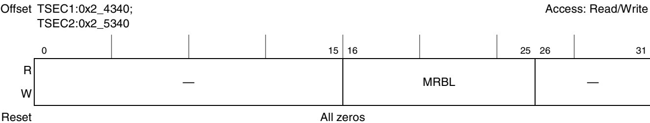
Figure 15-32. MRBL Register Definition
