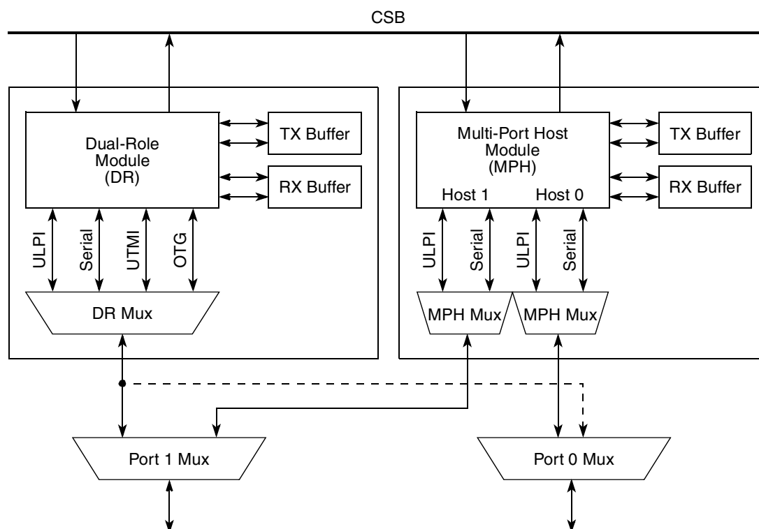
Figure 1-4. USB Controllers Port Configuration
