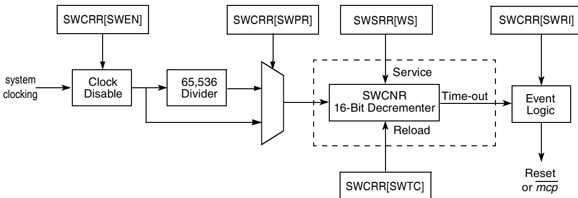
Figure 5-23. Software Watchdog Timer Functional Block Diagram
