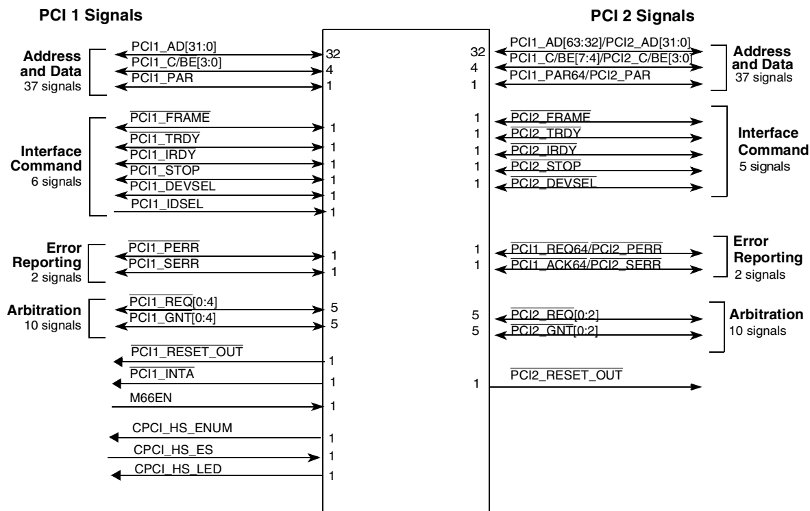
Figure 13-2. PCI Interface External Signals
