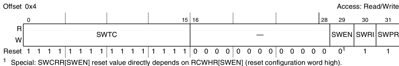
Figure 5-19. System Watchdog Control Register (SWCRR)
