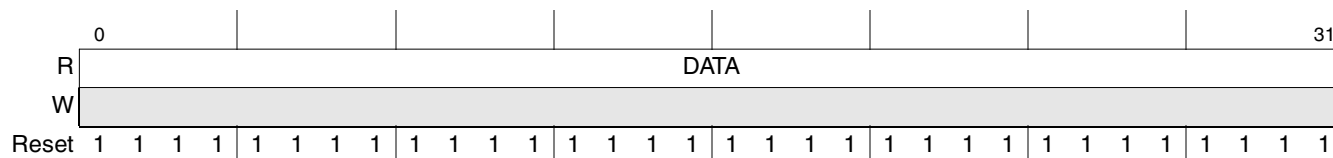
Figure 19-11. SPI Receive Data Hold Register
