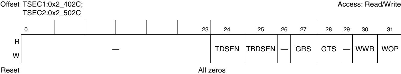
Figure 15-12. DMACTRL Register Definition
