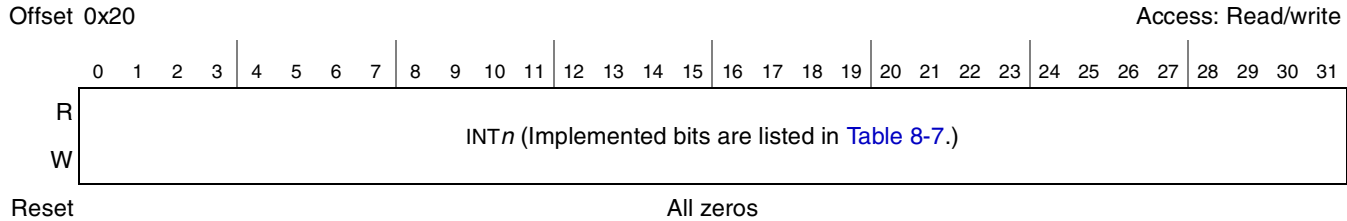
Figure 8-8. System Internal Interrupt Mask Register (SIMSR_H)
