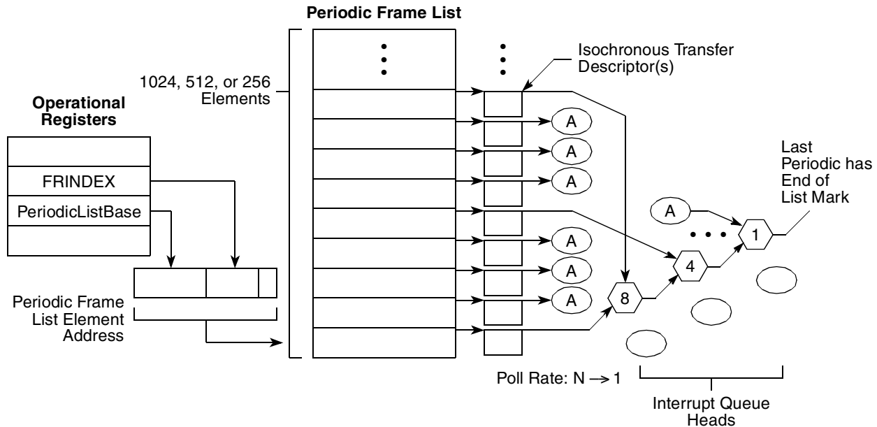
Figure 16-37. Periodic Schedule Organization
