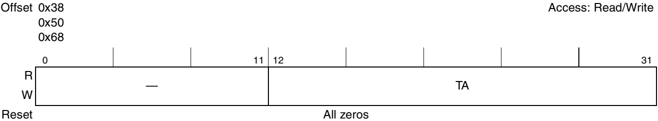
Figure 13-16. PCI Inbound Translation Address Registers (PITAR n )
