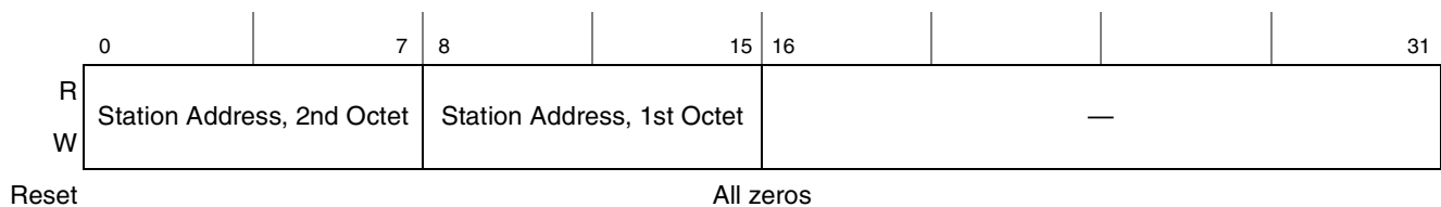
Figure 15-48. MACSTNADDR2 Register Definition
