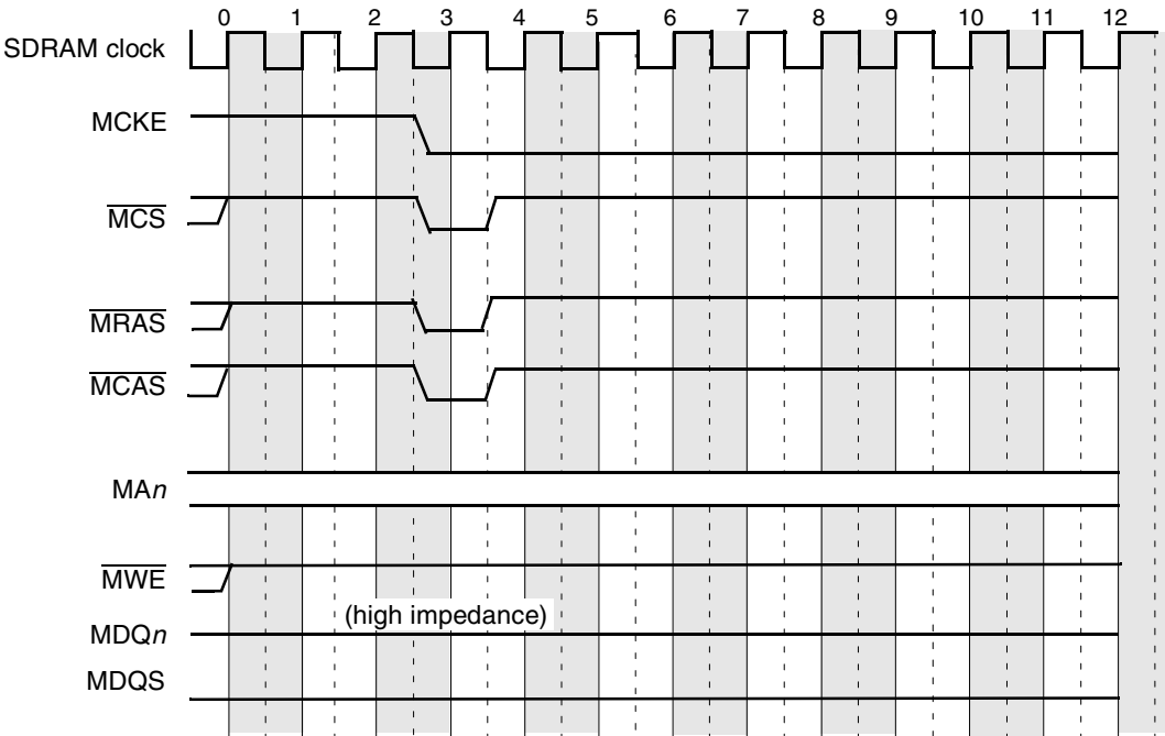
Figure 9-44. DDR SDRAM Self-Refresh Entry Timing
