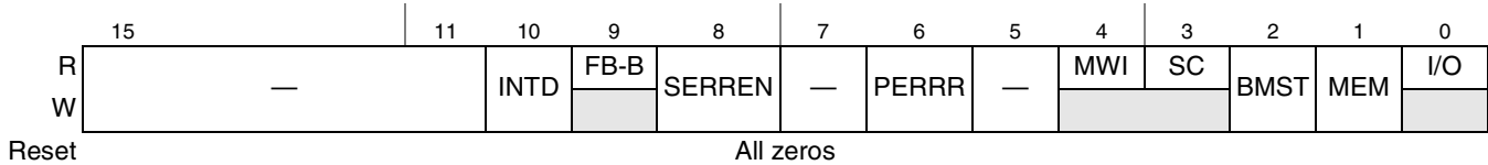
Figure 13-22. PCI Command Configuration Register
