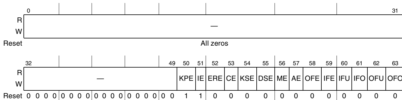
Figure 14-23. DEU Interrupt Control Register (DEUICR)
