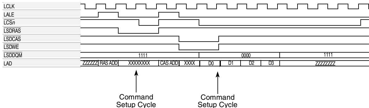
Figure 10-40. BUFCMD = 1, LCRR[BUFCMDC] = 2
