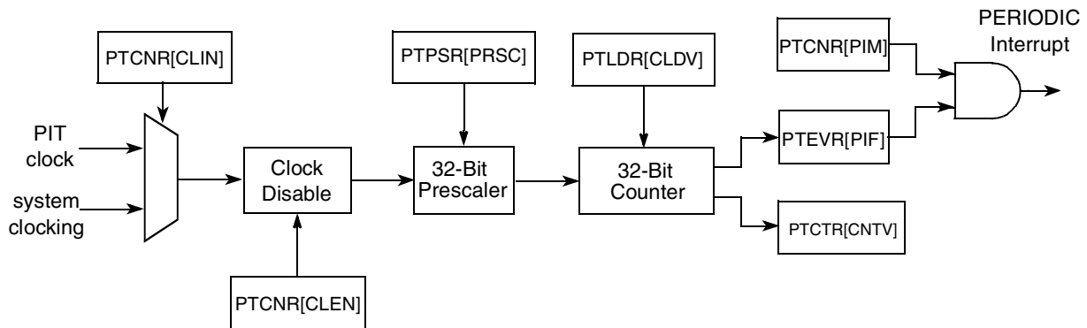
Figure 5-38. Periodic Interval Timer Functional Block Diagram
