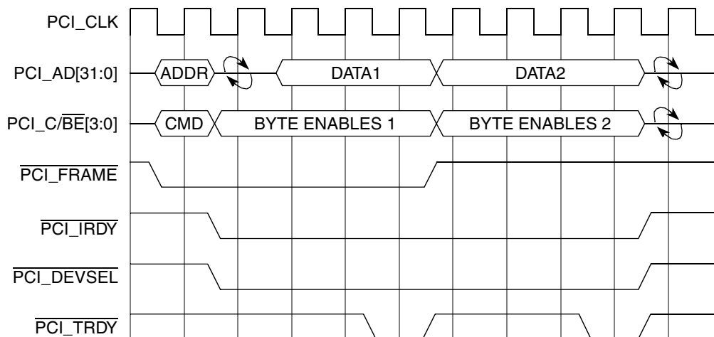
Figure 13-48. Burst Read Example
