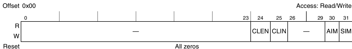
Figure 5-25. Real Time Counter Control Register (RTCNR)
