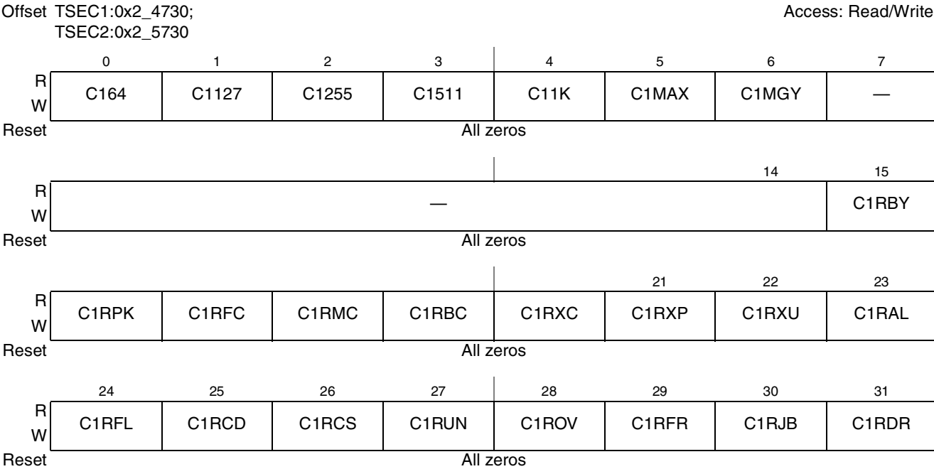
Figure 15-92. Carry Register 1 (CAR1) Register Definition
