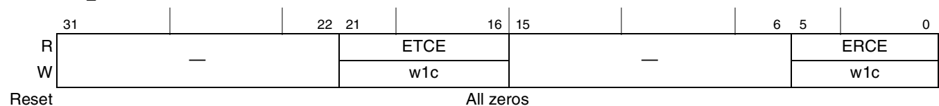
Figure 16-29. Endpoint Complete (ENDPTCOMPLETE)—DR-Only
