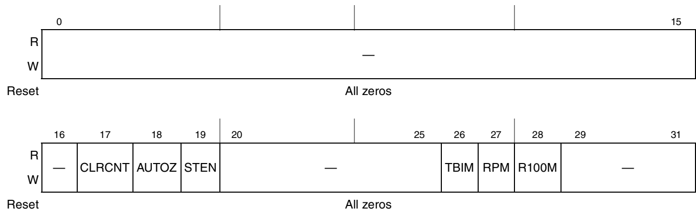
Figure 15-9. ECNTRL Register Definition
