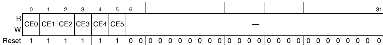
Figure 4-18. MCK Clock Register (MCKENR)
