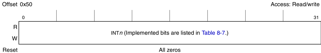
Figure 8-19. System Internal Interrupt Force Register (SIFCR_H)
