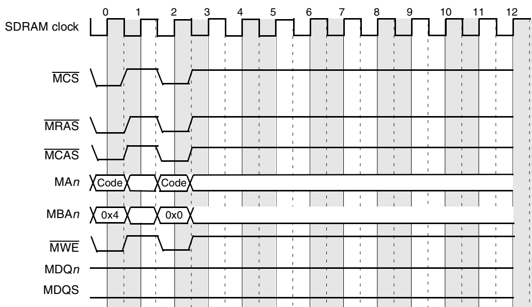
Figure 9-39. DDR SDRAM Mode-Set Command Timing
