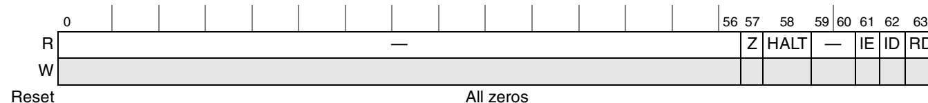
Figure 14-13. PKEU Status Register (PKEUSR)
