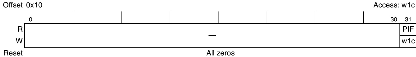
Figure 5-37. Periodic Interval Timer Event Register (PTEVR)
