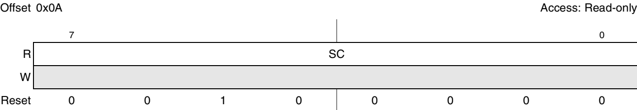
Figure 13-26. Subclass Code Configuration Register
