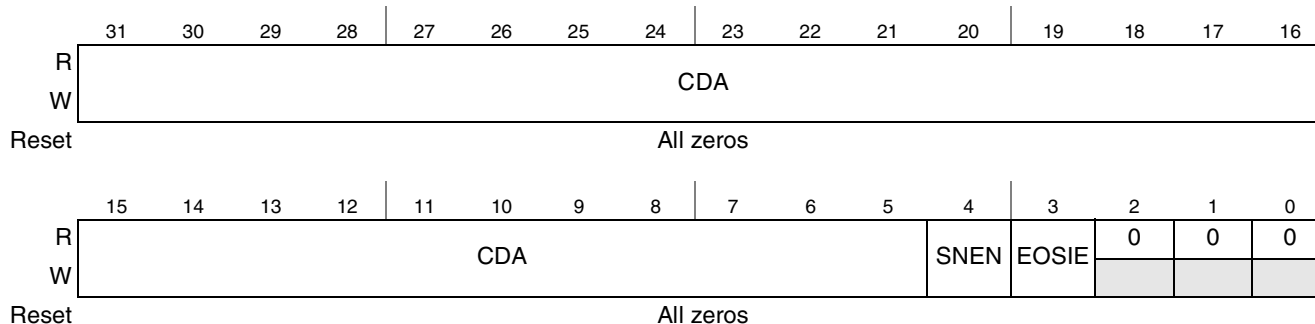
Figure 12-12. DMA Current Descriptor Address Register (DMACDAR n )
