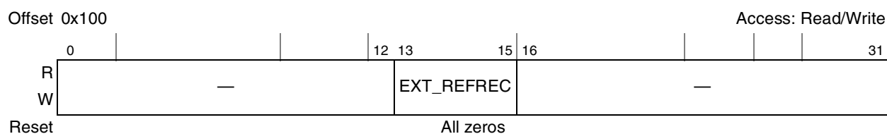
Figure 9-4. DDR SDRAM Timing Configuration 3 (TIMING_CFG_3)
