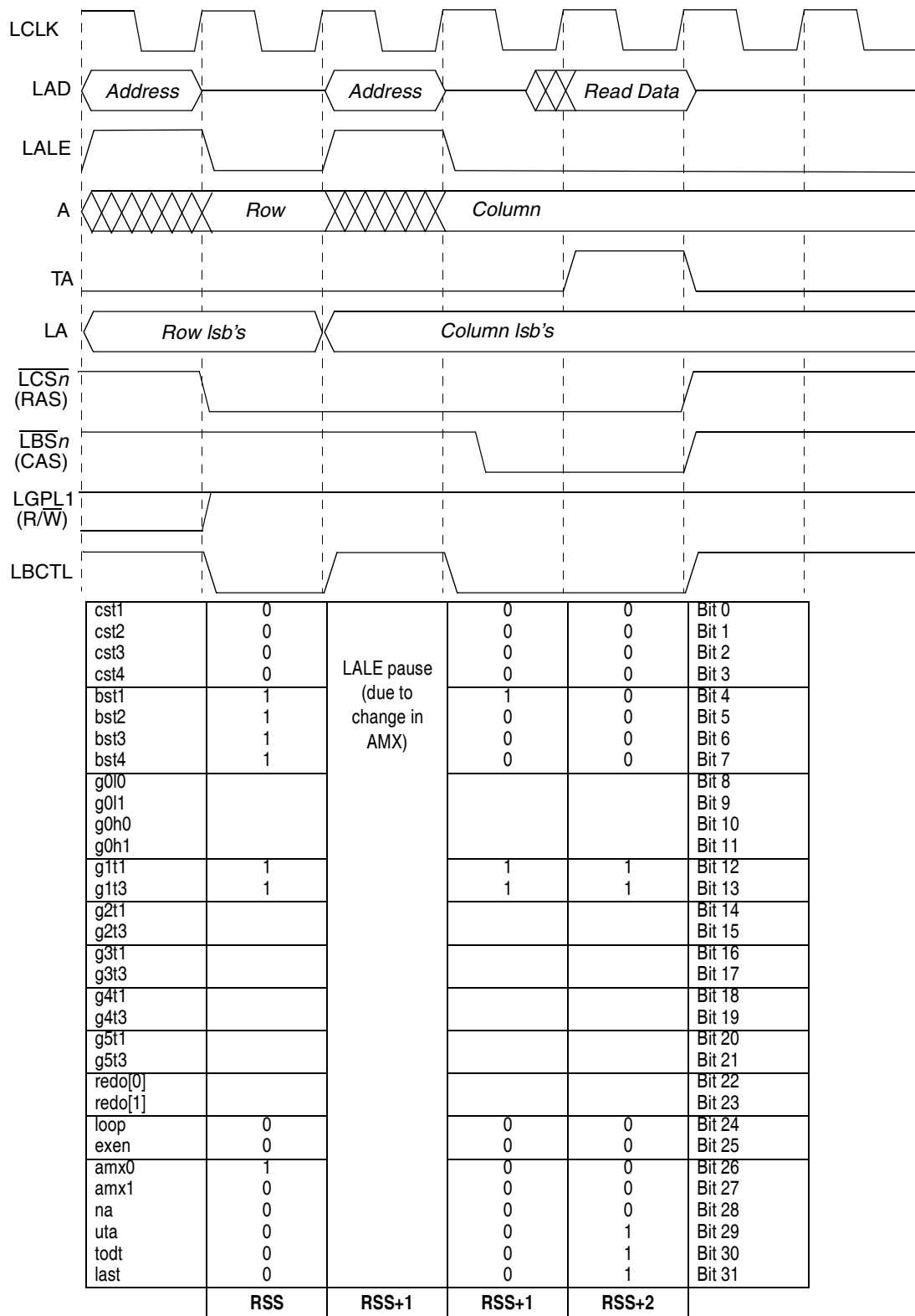
Figure 10-63. Single-Beat Read Access to FPM DRAM
