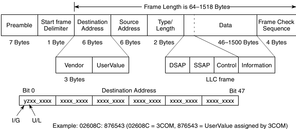
Figure 15-4. Ethernet/IEEE 802.3 Frame Structure with More Details
