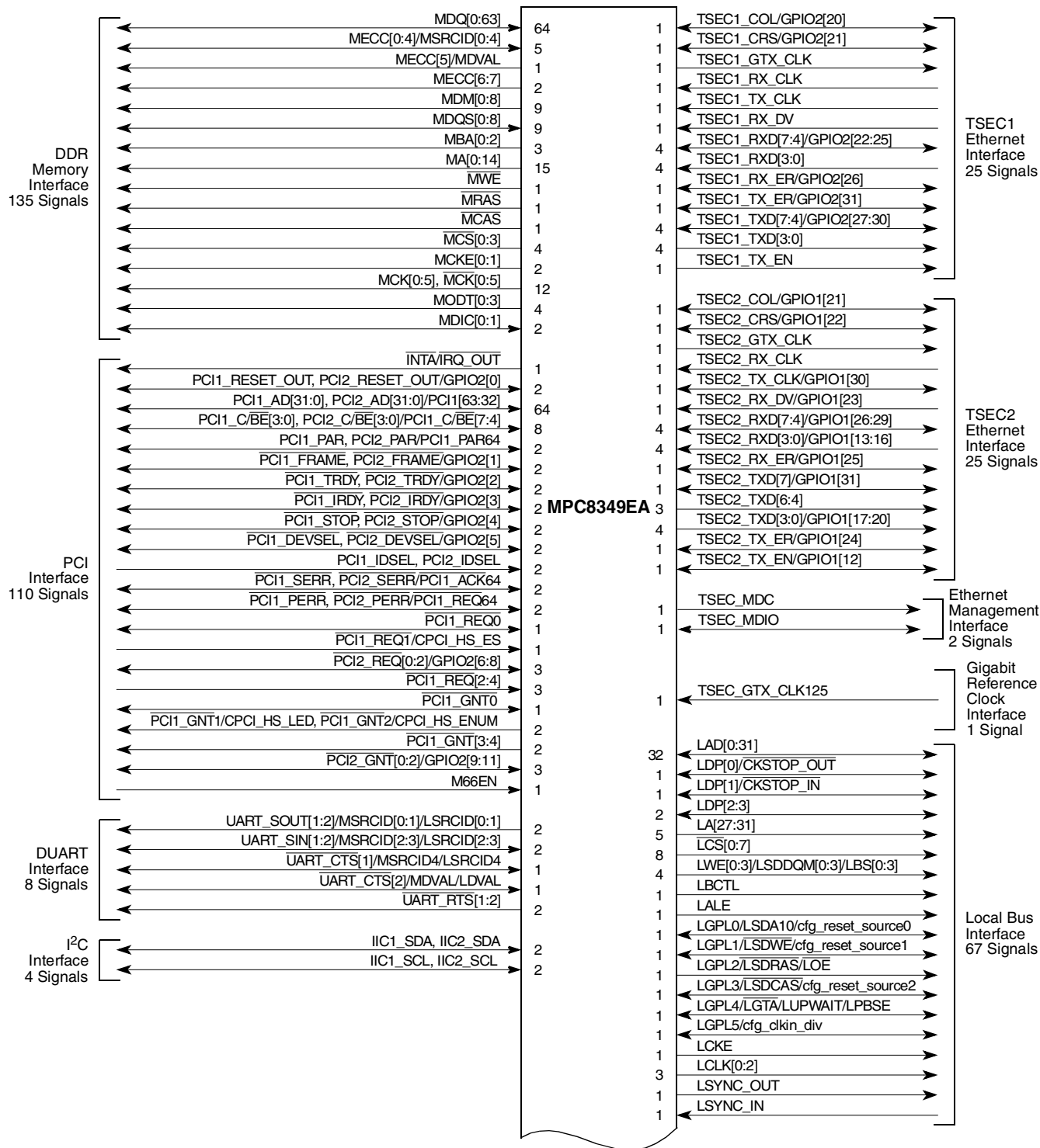
Figure 3-1. MPC8349EA Signal Groupings (1 of 2)
