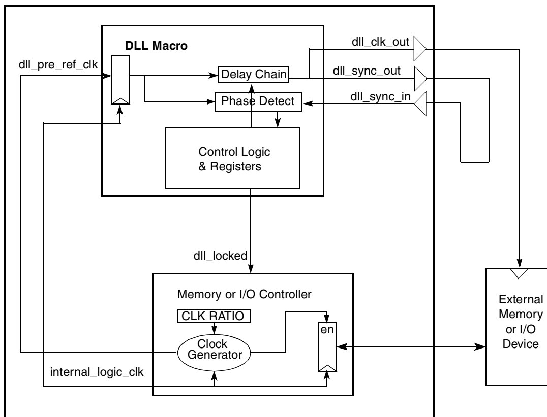
Figure 22-2. DLL Application Example
