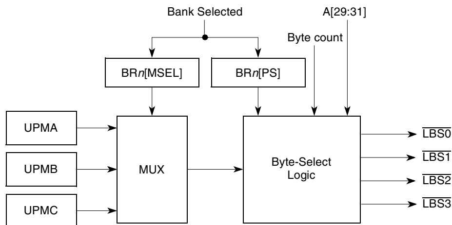
Figure 10-60. \overline{\text{LBS}} Signal Selection
