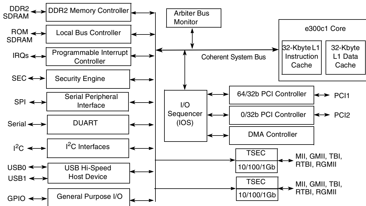
Figure 1-1. MPC8349EA Block Diagram
