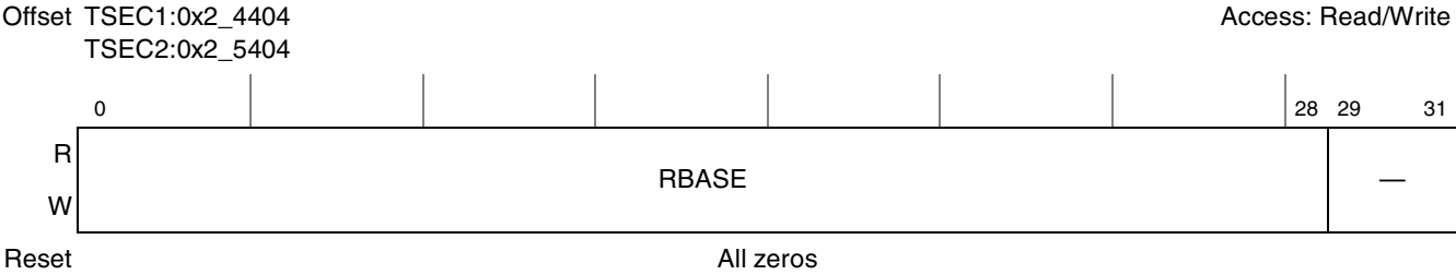
Figure 15-34. RBASE Register Definition
