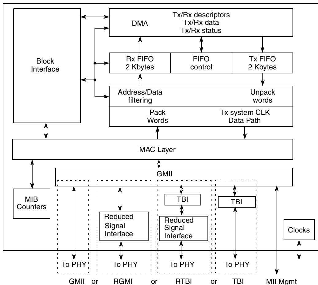
Figure 15-5. TSEC Block Diagram
