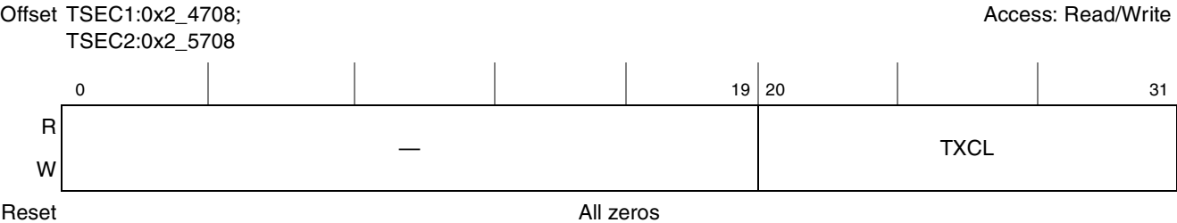
Figure 15-83. Transmit Excessive Collision Packet Counter Register Definition
