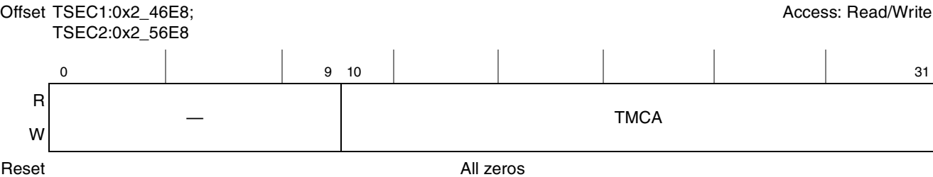
Figure 15-75. Transmit Multicast Packet Counter Register Definition
