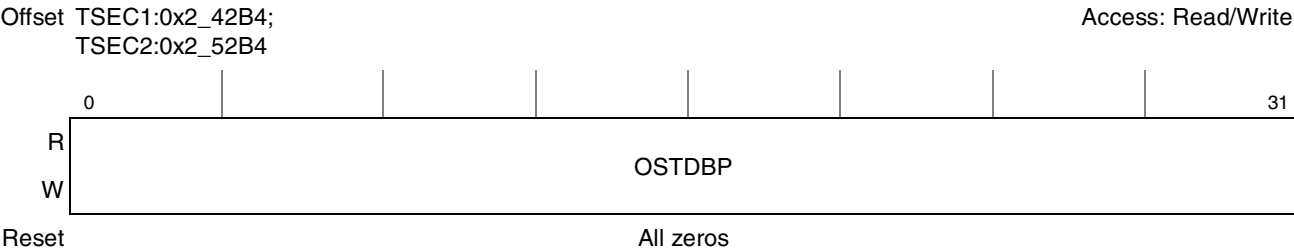
Figure 15-26. OSTDBP Register Definition
