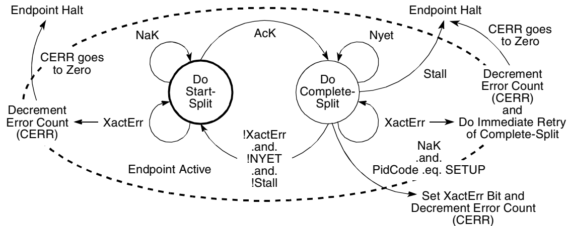
Figure 16-54. Host Controller Asynchronous Schedule Split-Transaction State Machine
