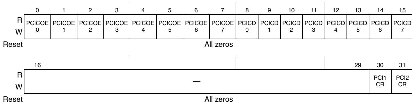
Figure 4-16. Output Clock Control Register (OCCR)
