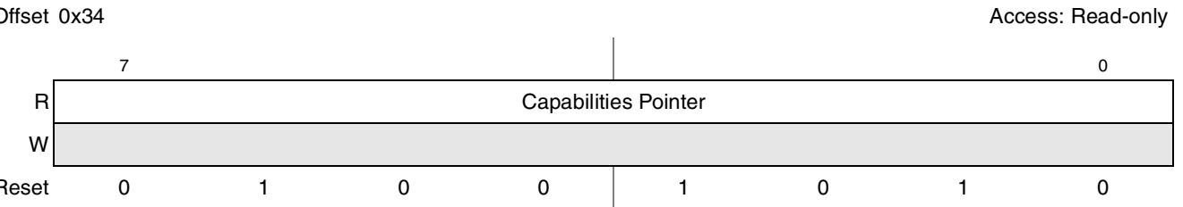
Figure 13-38. Capabilities Pointer Configuration Register
