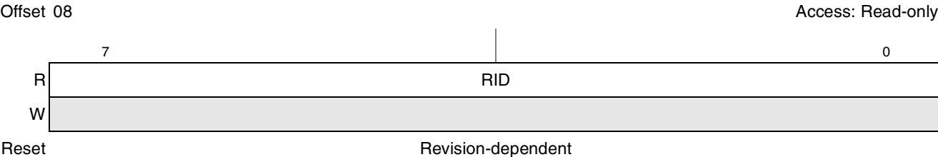
Figure 13-24. Revision ID Configuration Register
