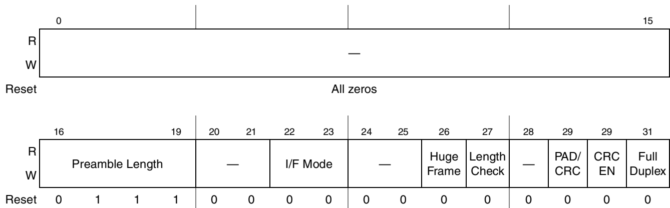
Figure 15-36. MACCFG2 Register Definition
