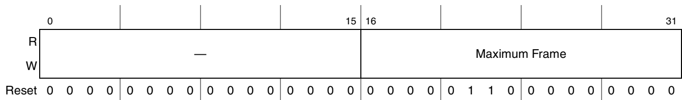
Figure 15-39. Maximum Frame Length Register Definition
