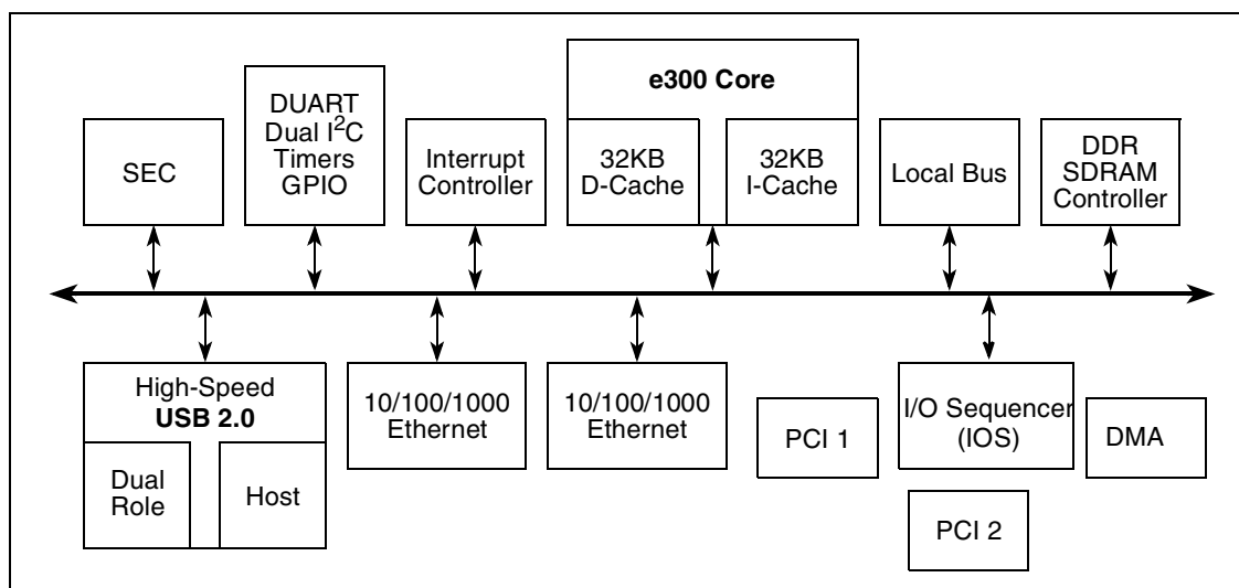
Figure 14-1. SEC Connected to MPC8349EA Internal Bus
