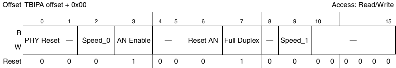
Figure 15-99. Control Register Definition
