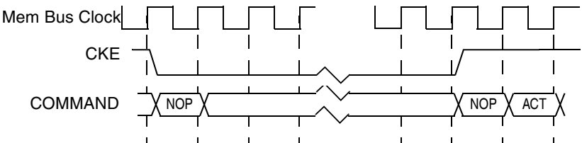
Figure 9-43. DDR SDRAM Power-Down Mode
