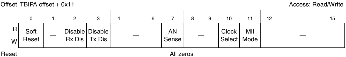
Figure 15-108. TBI Control Register Definition
