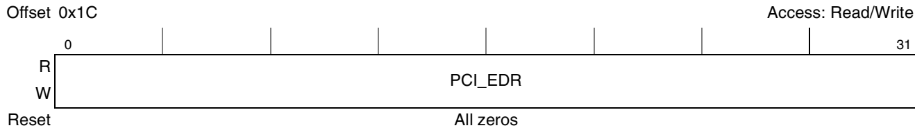
Figure 13-12. PCI Error Data High Capture Register (PCI_EDHCR)
