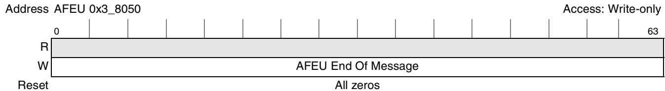
Figure 14-32. AFEU End of Message Register (AFEUEMR)
