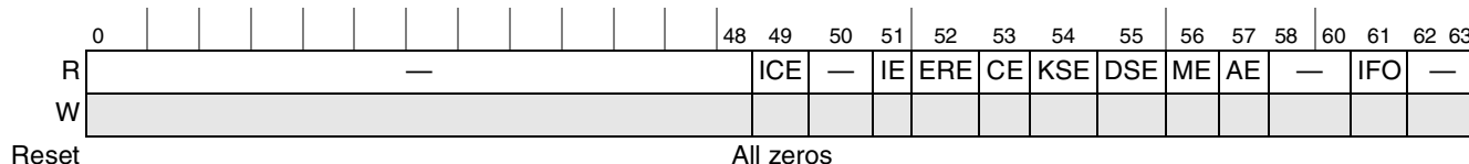
Figure 14-39. MDEU Interrupt Status Register (MDEUIR)
