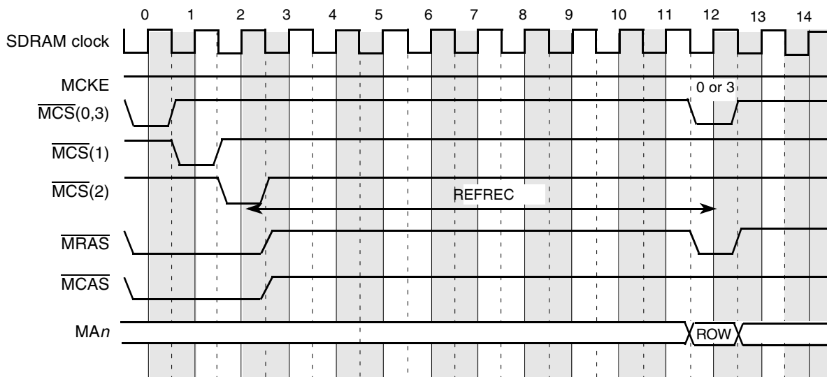
Figure 9-42. DDR SDRAM Bank Staggered Auto Refresh Timing
