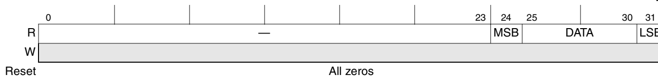
Figure 19-13. Example SPMODE[REV] = 1 SPMODE[LEN] = 7 MSB Sent First
