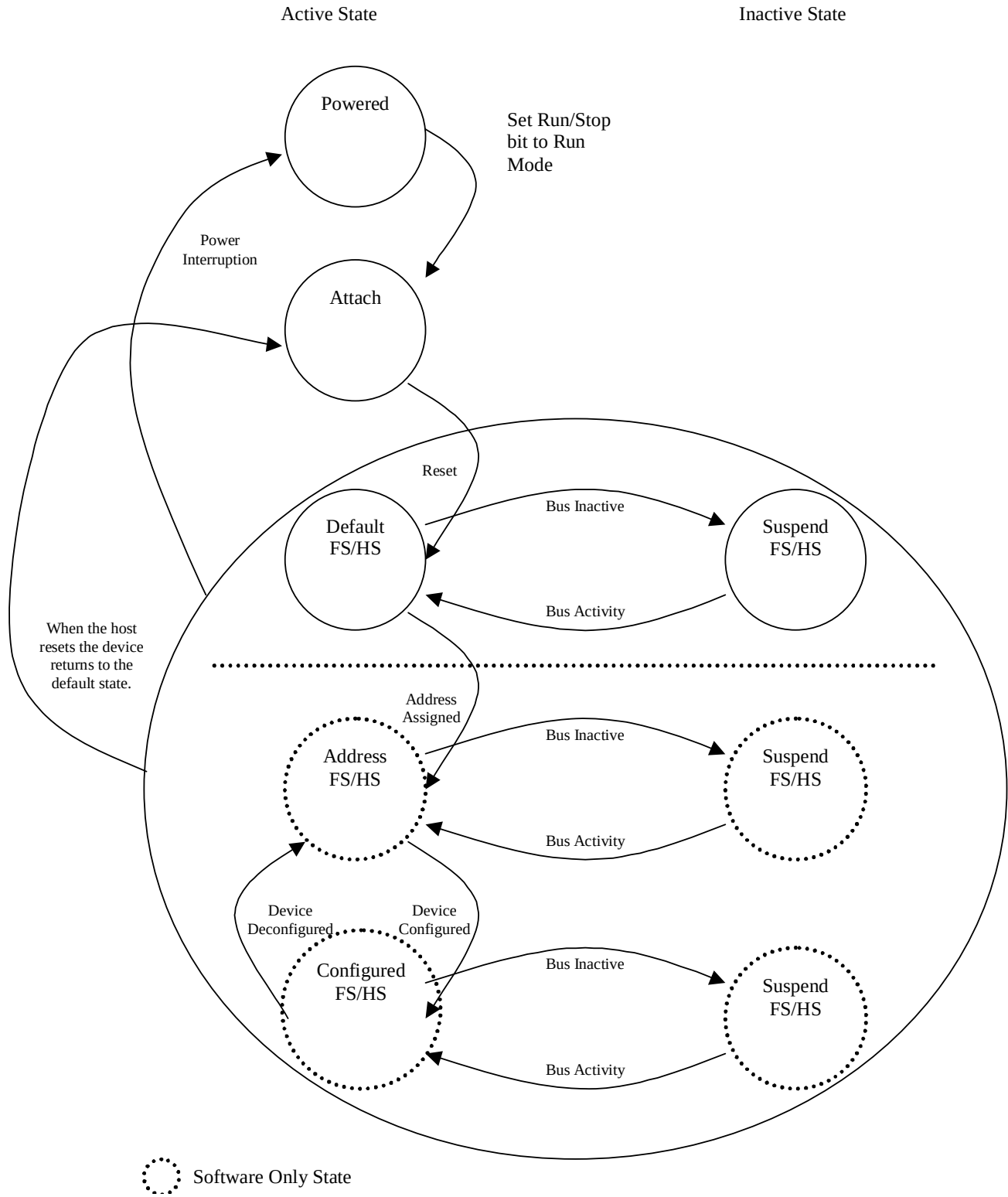
Figure 16-65. USB 2.0 Device States
