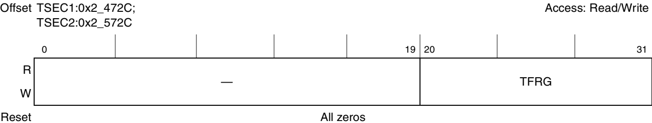
Figure 15-91. Transmit Fragment Counter Register Definition
