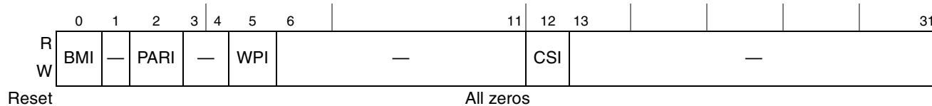
Figure 10-15. Transfer Error Interrupt Enable Register (LTEIR)
