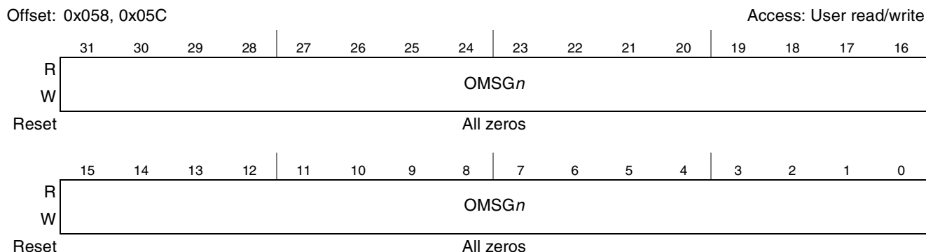
Figure 12-5. Outbound Message Registers (OMR0–OMR1)
