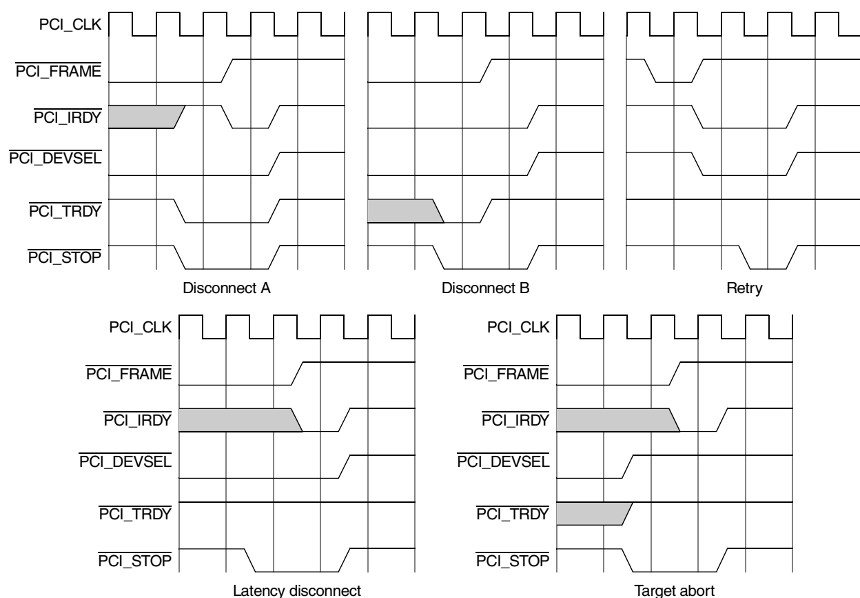
Figure 13-51. Target-Initiated Terminations
