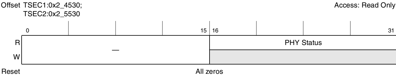
Figure 15-44. MIIMSTAT Register Definition
