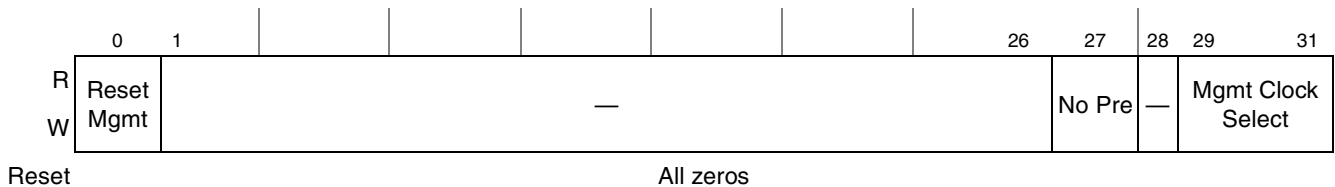
Figure 15-40. MII Management Configuration Register Definition
