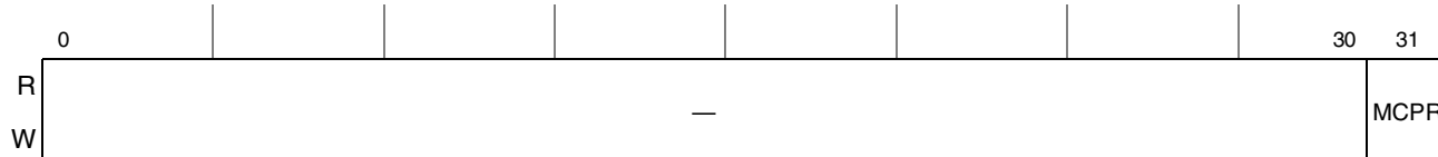
Figure 8-18. System Error Control Register (SERCER)
