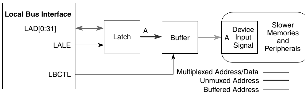
Figure 10-71. GPCM Address Timings
