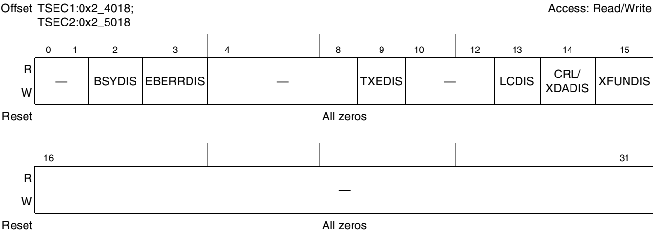
Figure 15-8. Error Disabled Register (EDIS)
