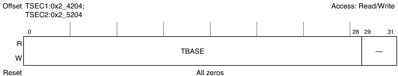
Figure 15-24. TBASE Register Definition
