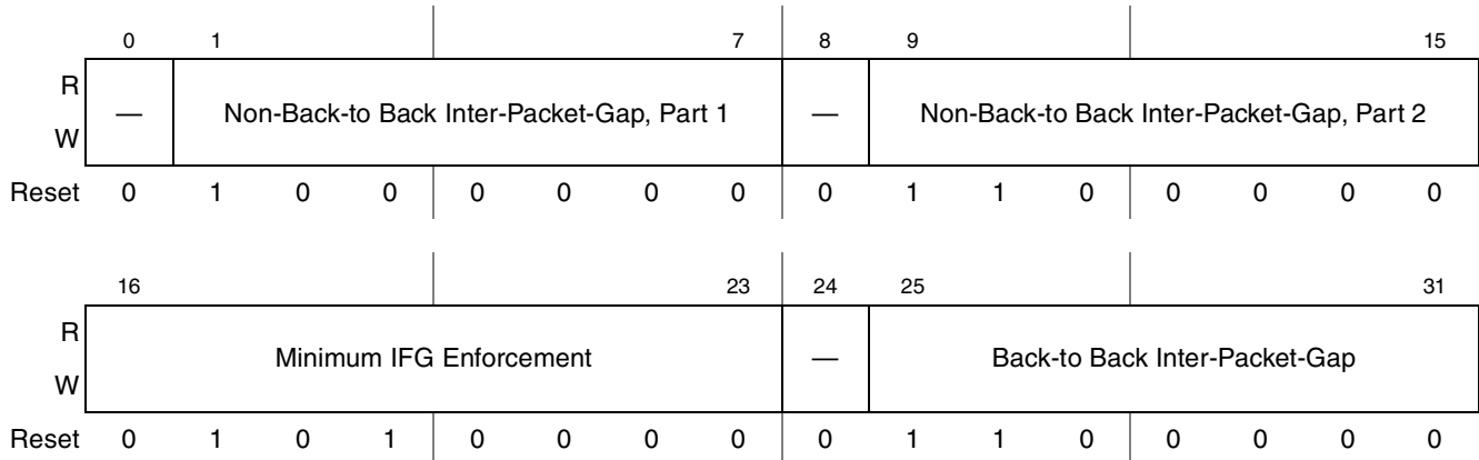
Figure 15-37. IPGIFG Register Definition
