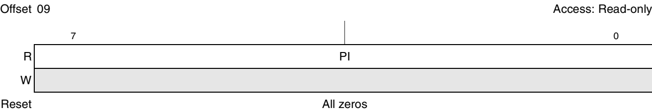
Figure 13-25. Standard Programming Interface Configuration Register
