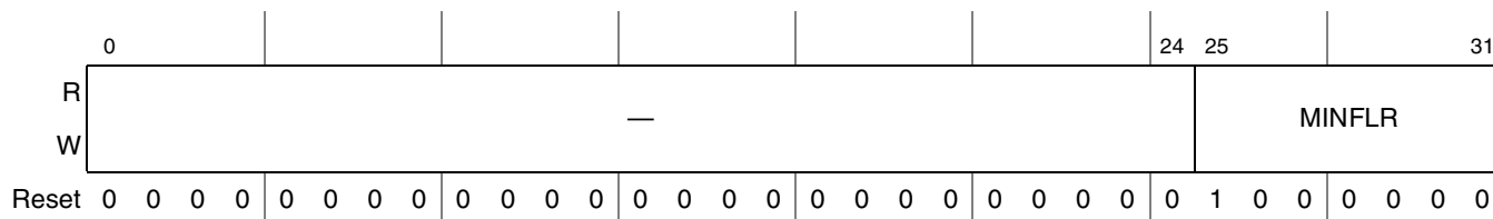
Figure 15-10. MINFLR Register Definition
