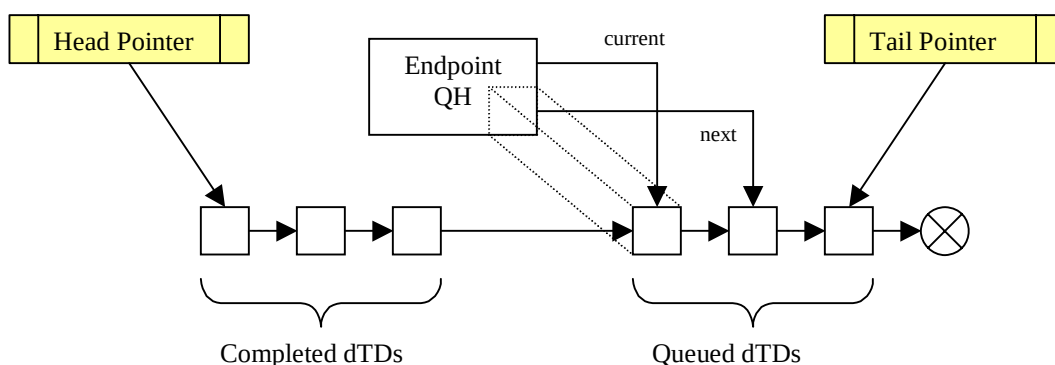
Figure 16-67. Software Link Pointers
