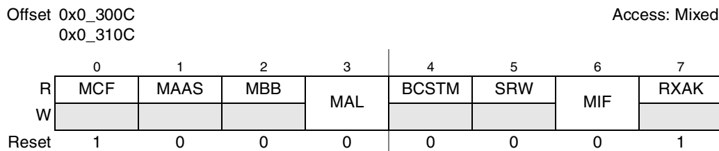
Figure 17-5. I 2 C n Status Register (I2C n SR)
