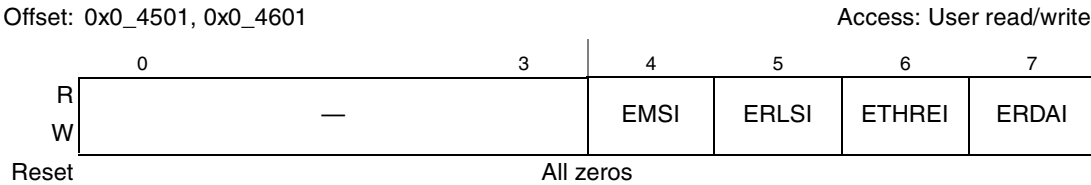
Figure 18-6. Interrupt Enable Registers (UIER1 and UIER2)
