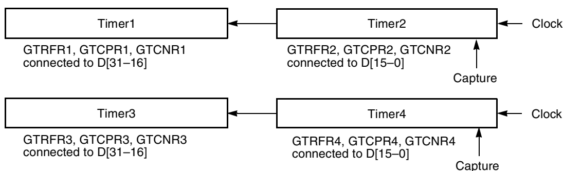
Figure 5-49. Timer Pair-Cascaded Mode Block Diagram
