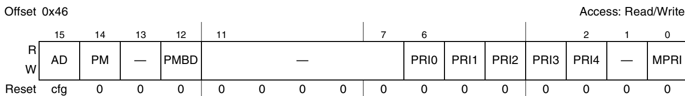
Figure 13-44. PCI Arbiter Control Register (PCIACR)
