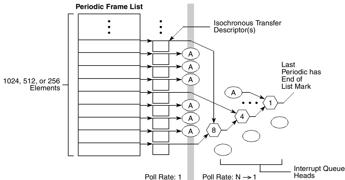
Figure 16-49. Example Periodic Schedule
