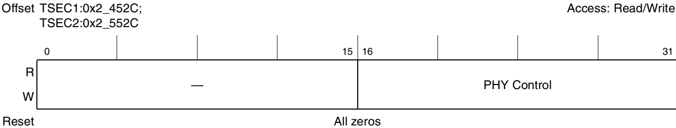
Figure 15-43. MII Management Control Register Definition
