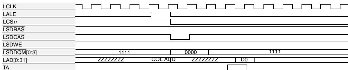
Figure 10-42. SDRAM Single-Beat Read, Page Hit, CL = 3
