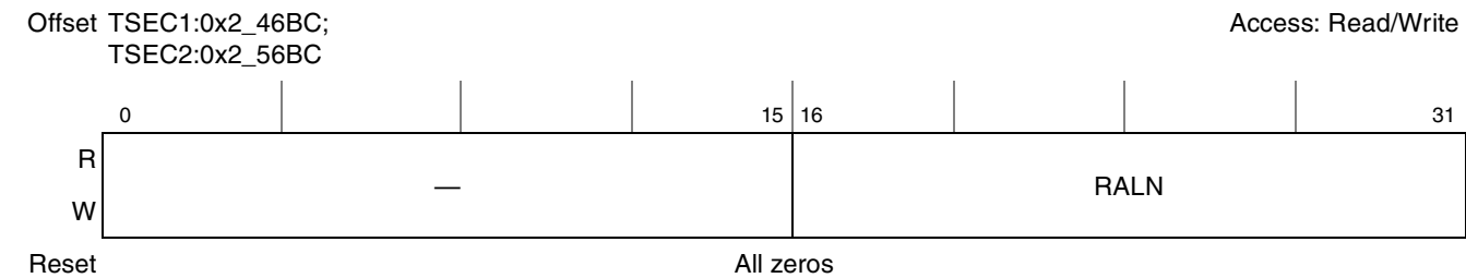
Figure 15-64. Receive Alignment Error Counter Register Definition
