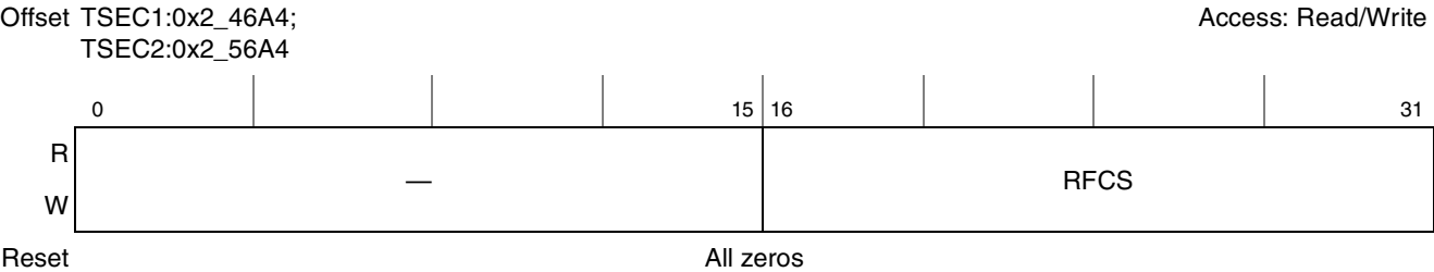
Figure 15-58. Receive FCS Error Counter Register Definition
