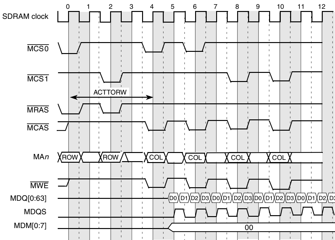
Figure 9-37. DDR SDRAM 4-Beat Burst Write Timing—ACTTORW = 4
