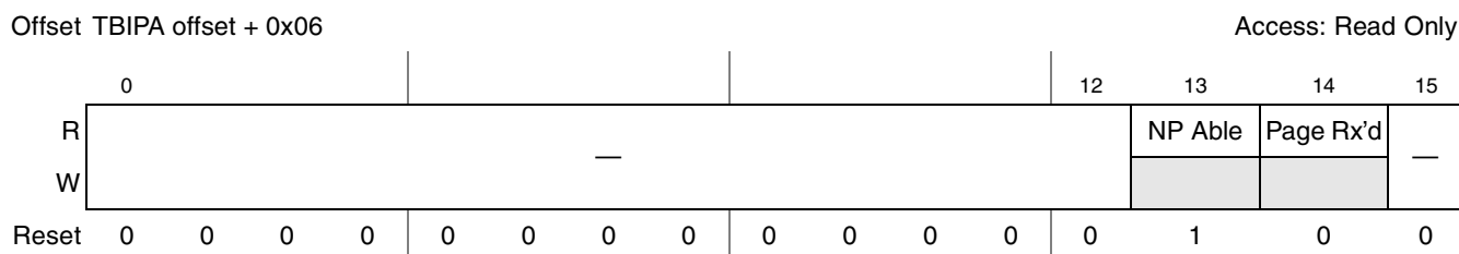
Figure 15-103. AN Expansion Register Definition
