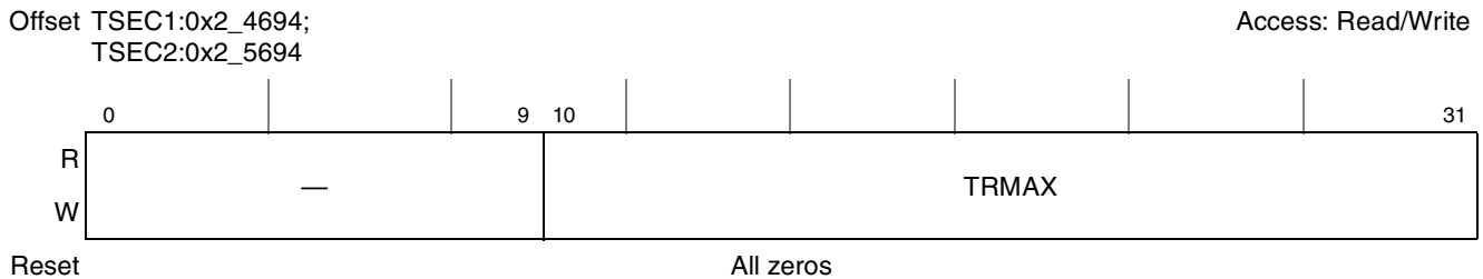
Figure 15-54. Transmit and Received 1024- to 1518-Byte Frame Register Definition
