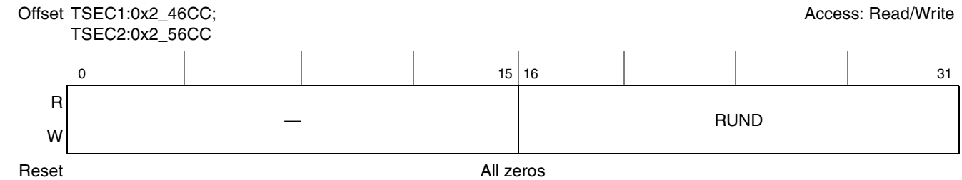
Figure 15-68. Receive Undersize Packet Counter Register Definition
