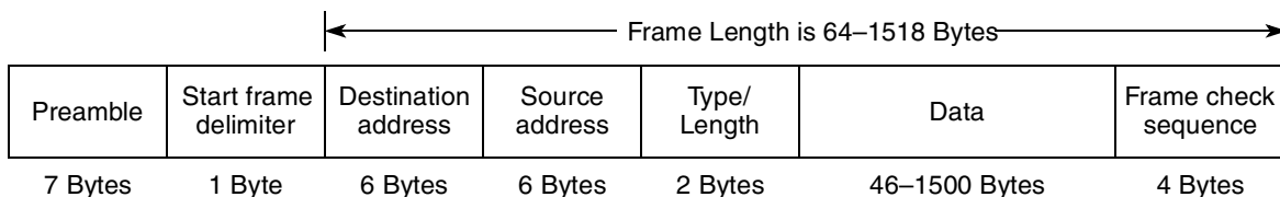
Figure 15-3. Ethernet/IEEE 802.3 Frame Structure
