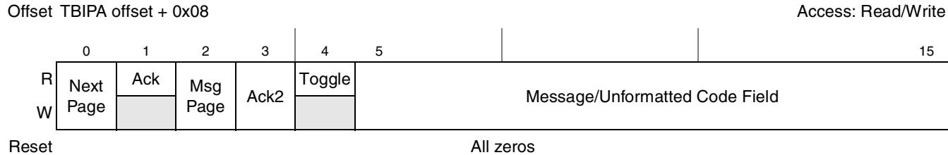
Figure 15-105. AN Link Partner Ability Next Page Register Definition
