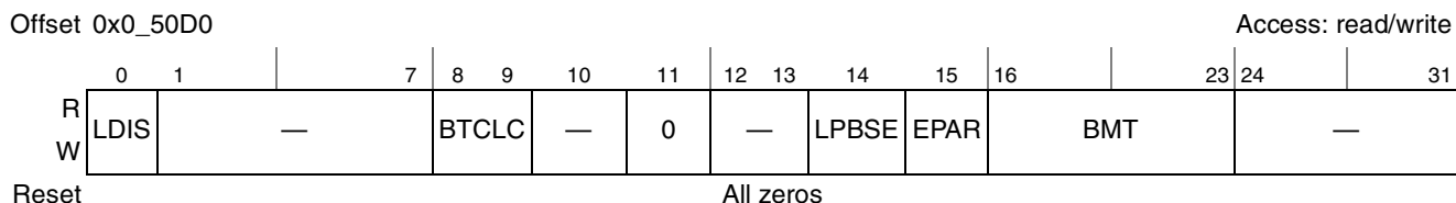
Figure 10-18. Local Bus Configuration Register
