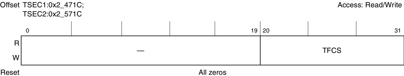
Figure 15-87. Transmit FCS Error Counter Register Definition
