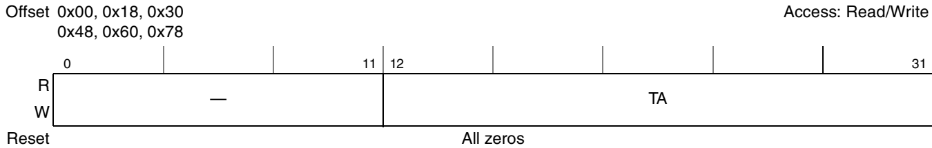
Figure 11-2. PCI Outbound Translation Address Registers (POTAR n )
