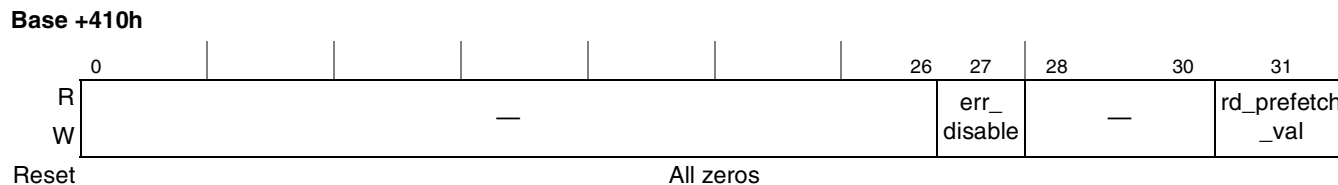
Figure 16-34. System Interface Control Register (SI_CTRL)
