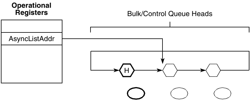
Figure 16-39. Asynchronous Schedule Organization
