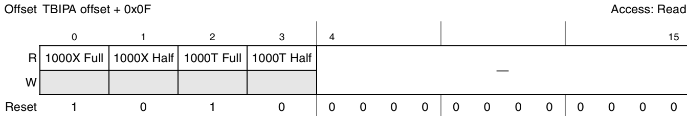
Figure 15-106. Extended Status Register Definition
