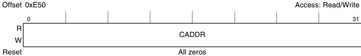
Figure 9-29. Memory Error Address Capture Register (CAPTURE_ADDRESS)
