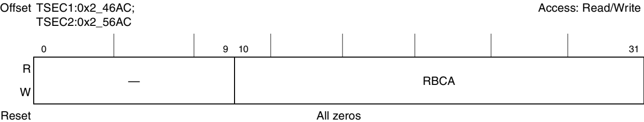
Figure 15-60. Receive Broadcast Packet Counter Register Definition
