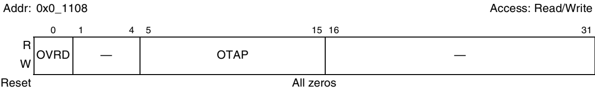
Figure 22-3. DLL Override Register
