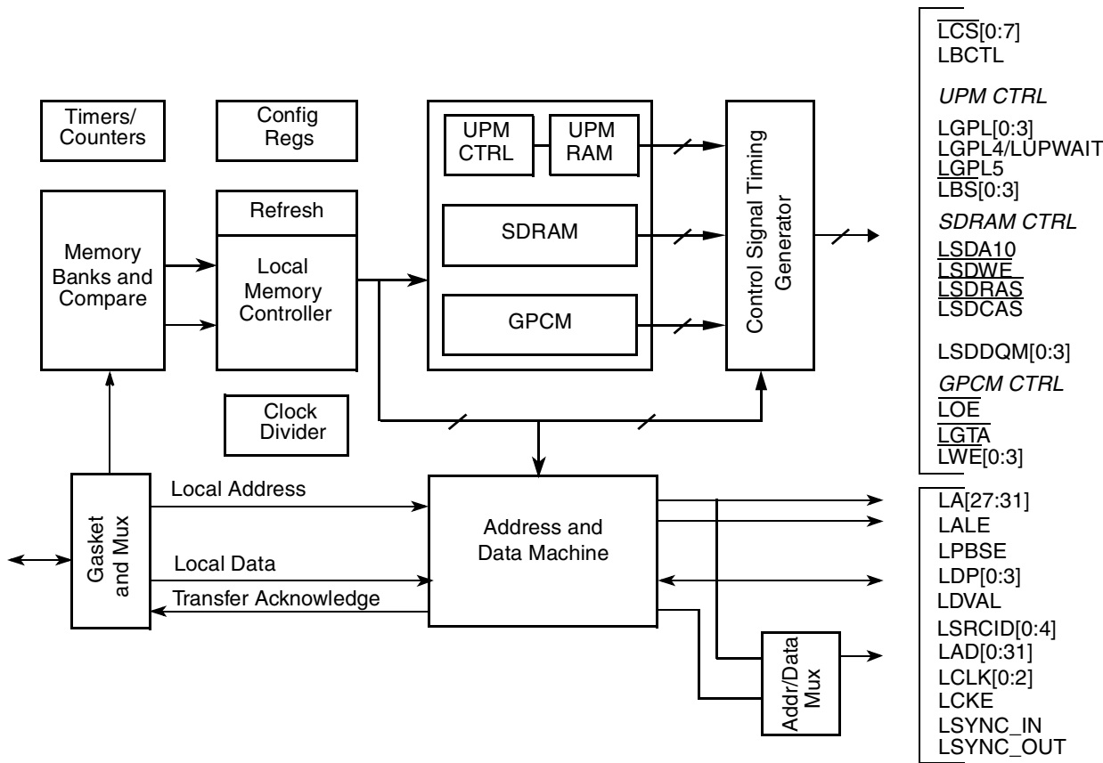
Figure 10-1. Local Bus Controller Block Diagram
