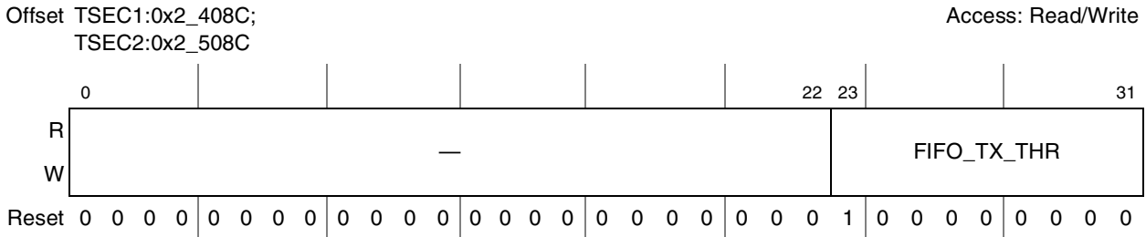
Figure 15-14. FIFO_TX_THR Register Definition
