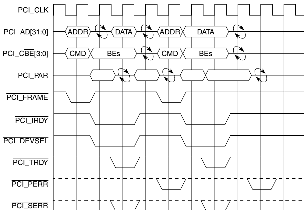
Figure 13-52. PCI Parity Operation
