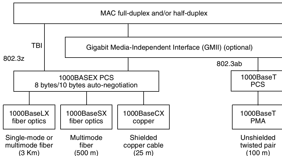
Figure 15-2. 802.3z and 802.3ab Physical Standards
