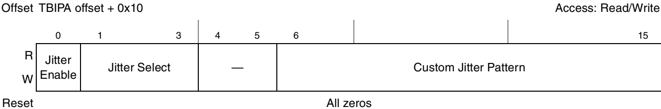
Figure 15-107. Jitter Diagnostics Register Definition
