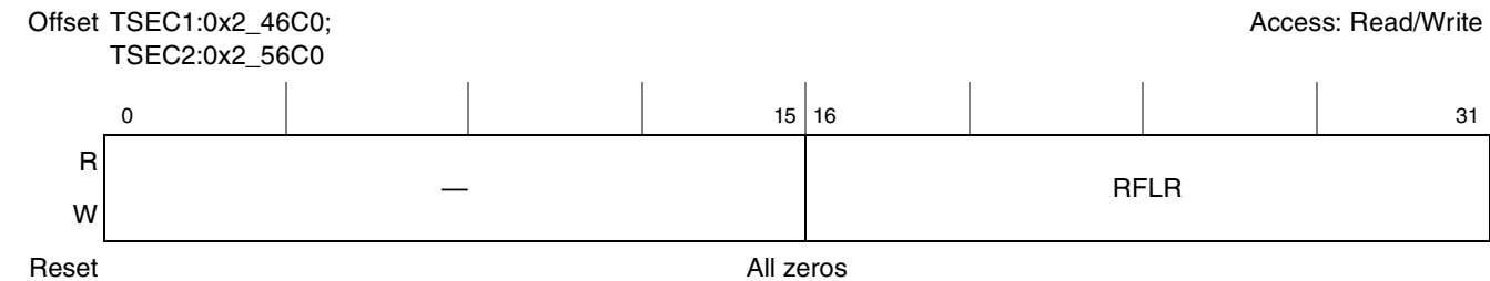
Figure 15-65. Receive Frame Length Error Counter Register Definition
