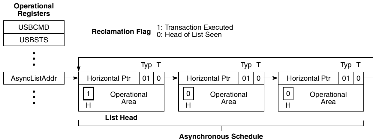
Figure 16-52. Asynchronous Schedule List with Annotation to Mark Head of List
