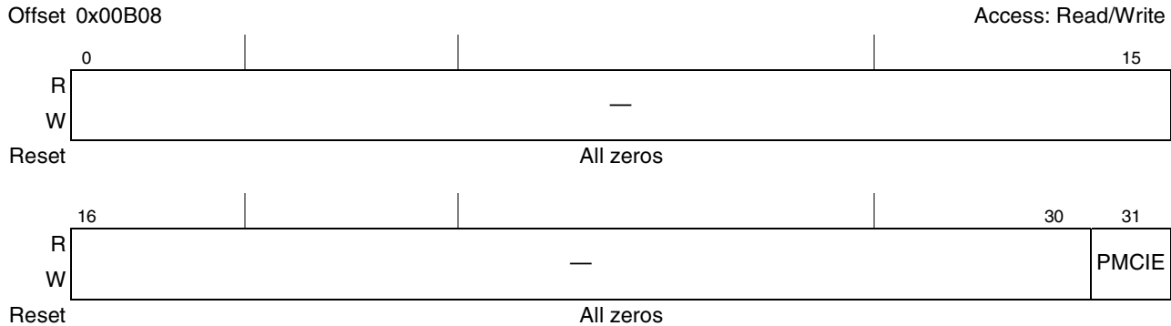
Figure 5-53. Power Management Controller Mask Register
