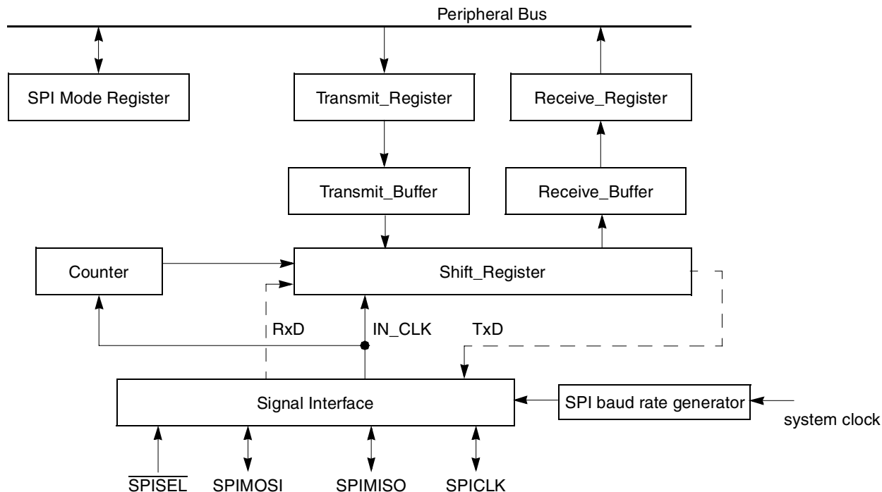
Figure 19-1. SPI Block Diagram
