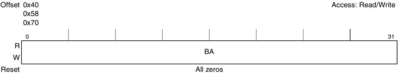
Figure 13-17. PCI Inbound Base Address Registers (PIBAR n )
