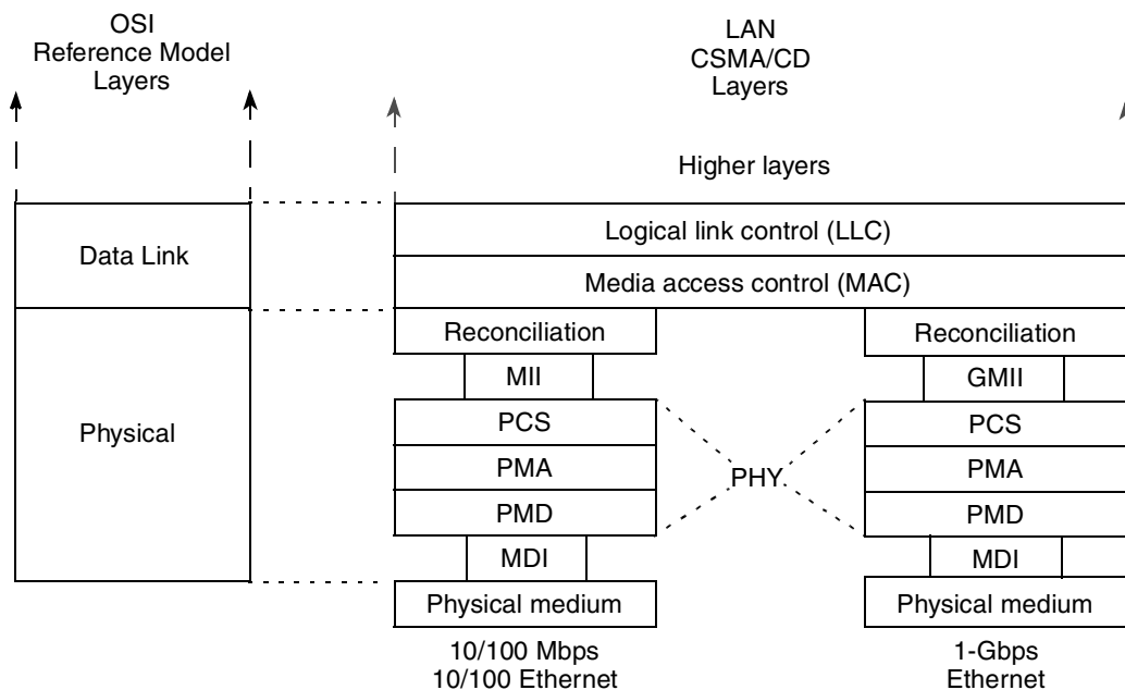
Figure 15-1. Ethernet Protocol in Relation to the OSI Protocol Stack
