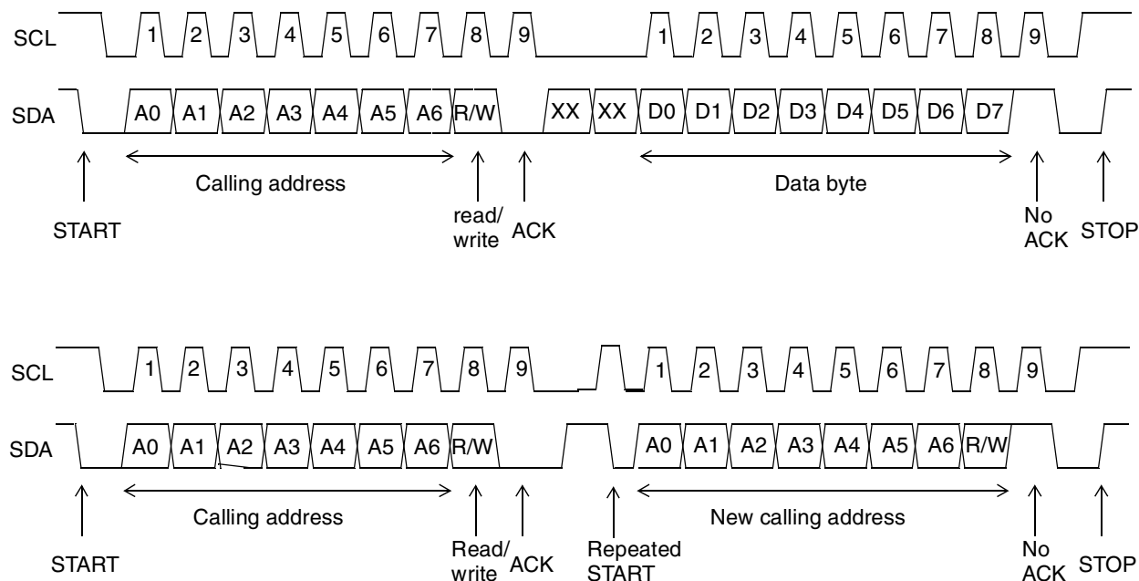
Figure 17-8. I 2 C Interface Transaction Protocol
