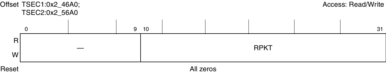
Figure 15-57. Receive Packet Counter Register Definition
