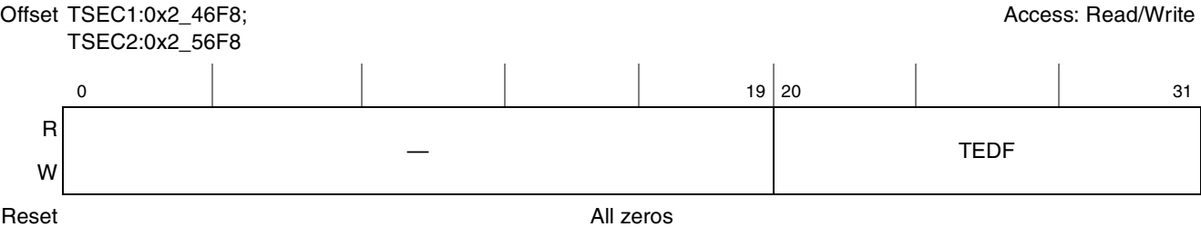
Figure 15-79. Transmit Excessive Deferral Packet Counter Register Definition
