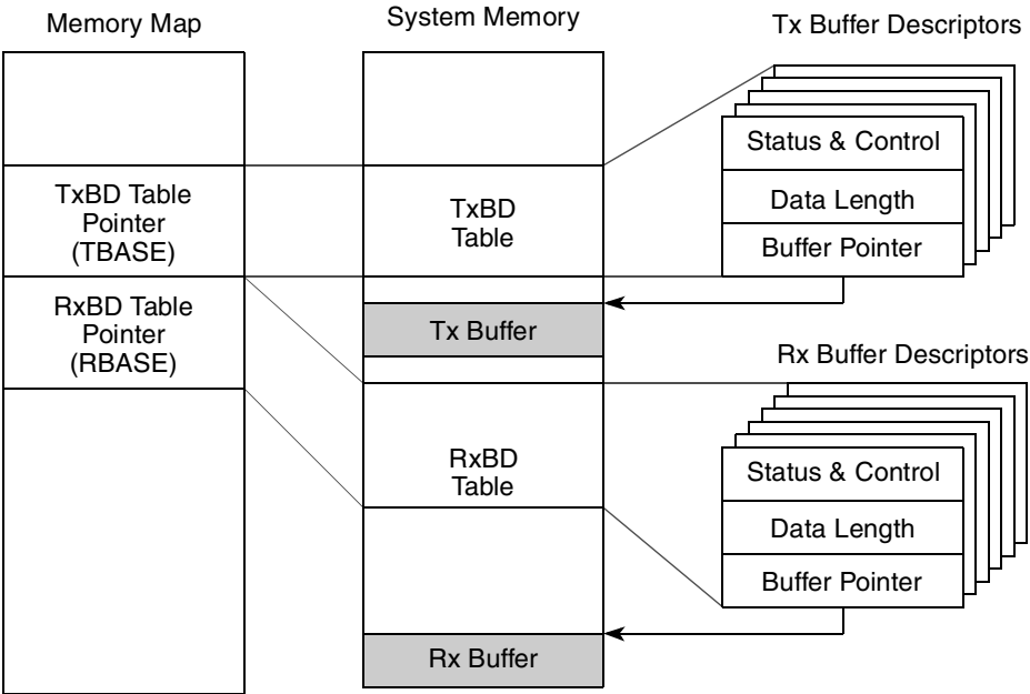
Figure 15-115. Example of TSEC Memory Structure for BD
