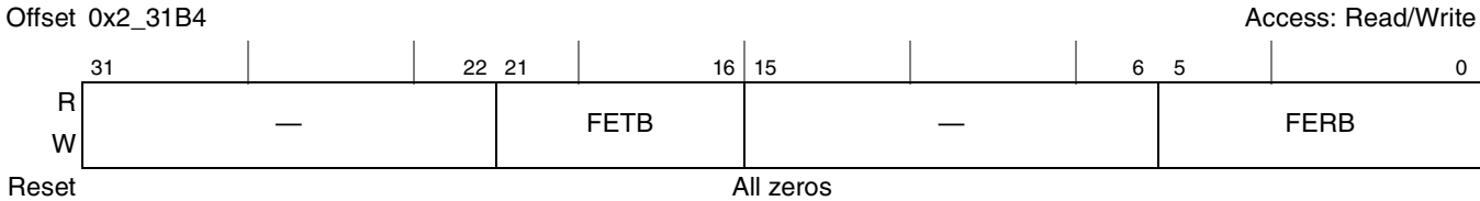
Figure 16-27. Endpoint Flush (ENDPTFLUSH)—DR-Only
