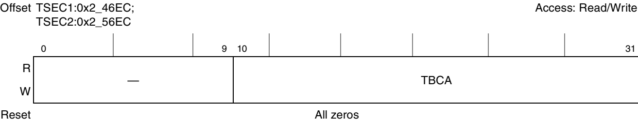
Figure 15-76. Transmit Broadcast Packet Counter Register Definition
