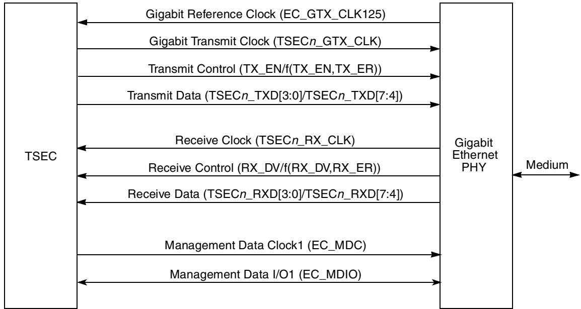
Figure 15-111. TSEC-RGMII Connection
