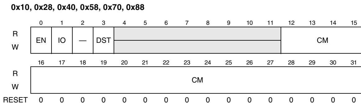
Figure 11-4. PCI Outbound Comparison Mask Registers (POCMR n )
