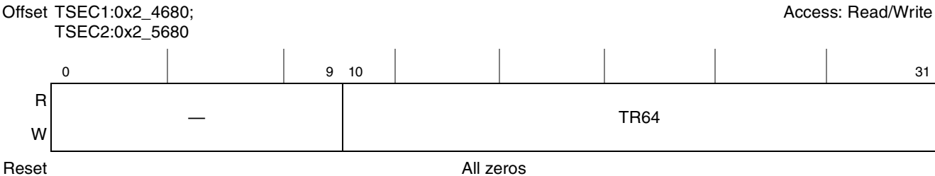
Figure 15-49. Transmit and Receive 64-Byte Frame Register Definition
