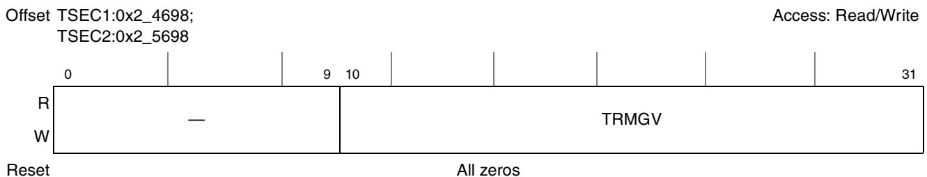
Figure 15-55. Transmit and Received 1519- to 1522-Byte VLAN Frame Register Definition
