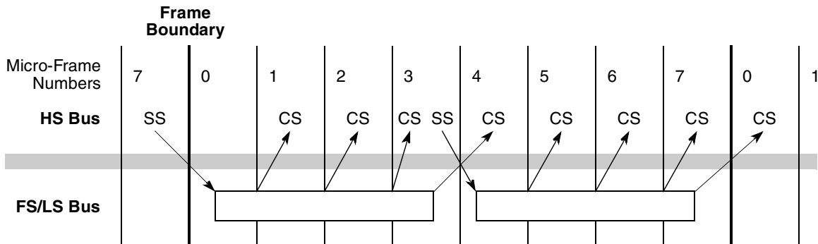
Figure 16-47. Frame Boundary Relationship between HS Bus and FS/LS Bus
