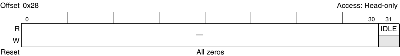
Figure 13-15. PCI General Status Register (PCI_GSR)
