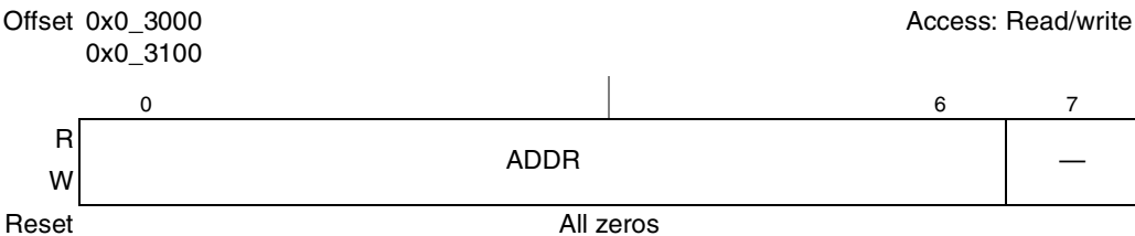
Figure 17-2. I 2 Cn Address Register (I2CnADR)
