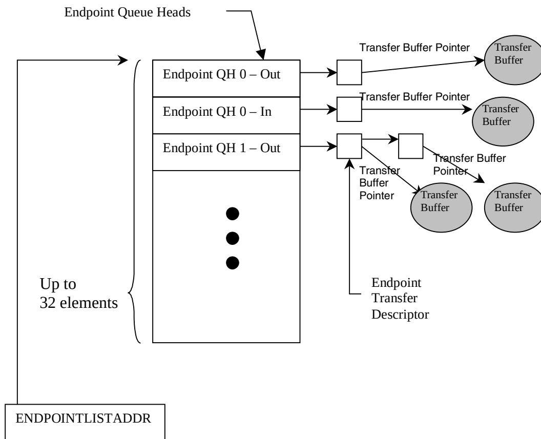
Figure 16-66. Endpoint Queue Head Diagram
