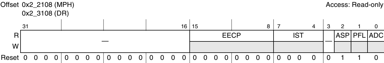
Figure 16-5. Host Control Capability Parameters (HCCPARAMS)
