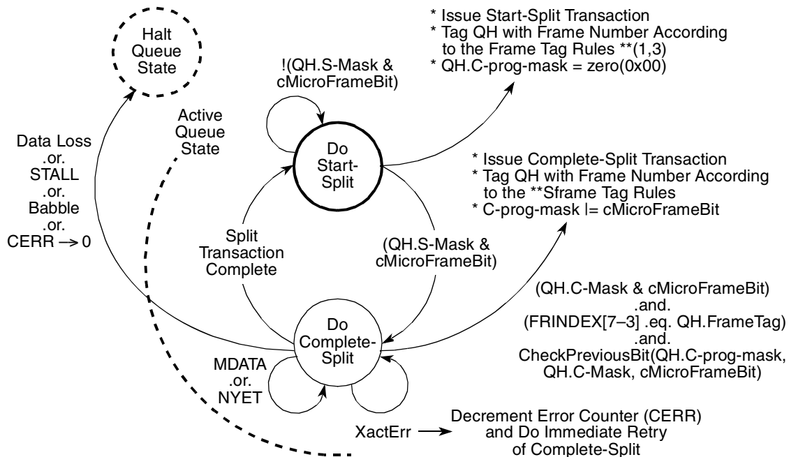
Figure 16-58. Split Transaction State Machine for Interrupt
