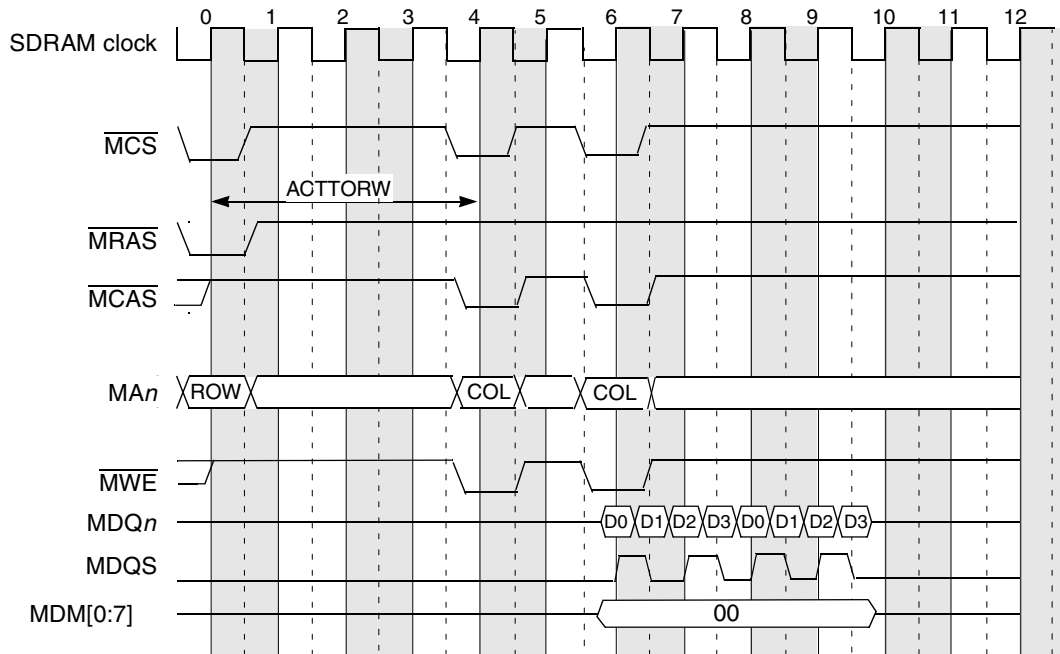
Figure 9-40. Registered DDR1 SDRAM DIMM Burst Write Timing
