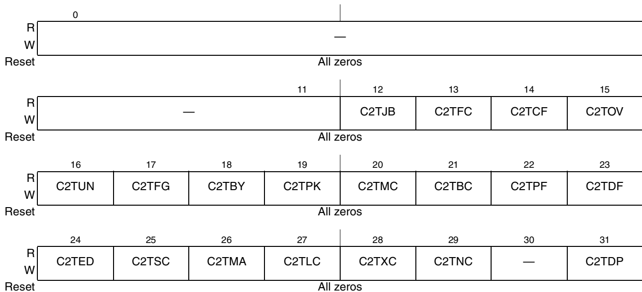
Figure 15-93. Carry Register 2 (CAR2) Register Definition
