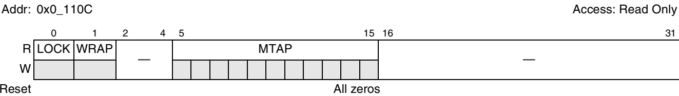
Figure 22-4. DLL Status Register
