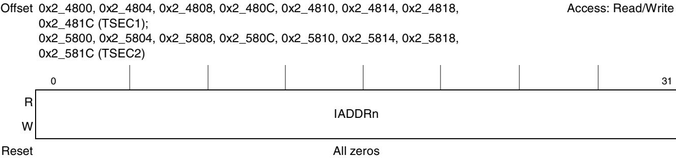
Figure 15-96. IADDRn Register Definition
