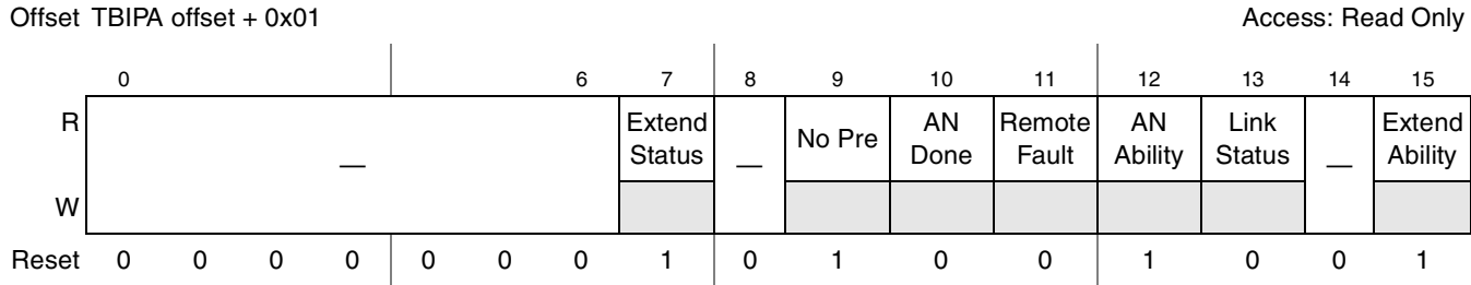
Figure 15-100. Status Register Definition
