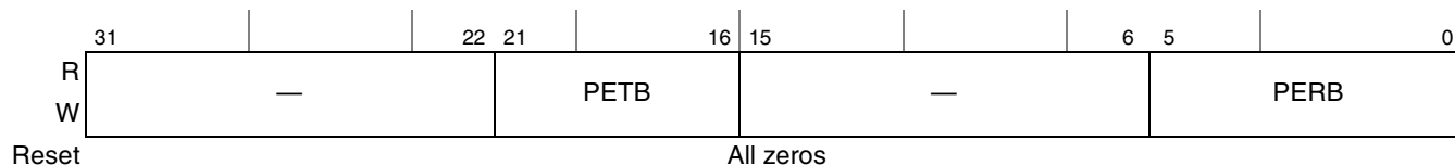
Figure 16-26. Endpoint Initialization (ENDPTPRIME)—DR-Only
