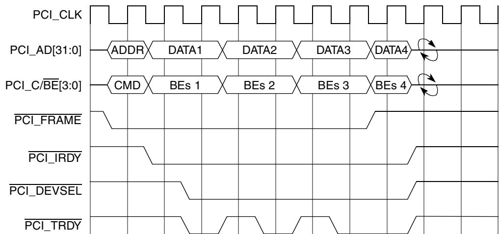
Figure 13-50. Burst Write Example
