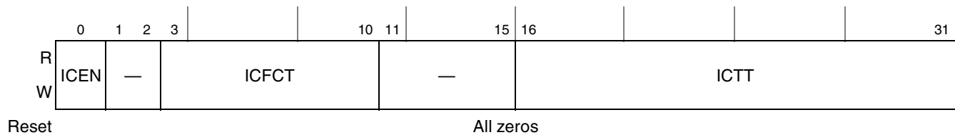
Figure 15-30. RXIC Register Definition
