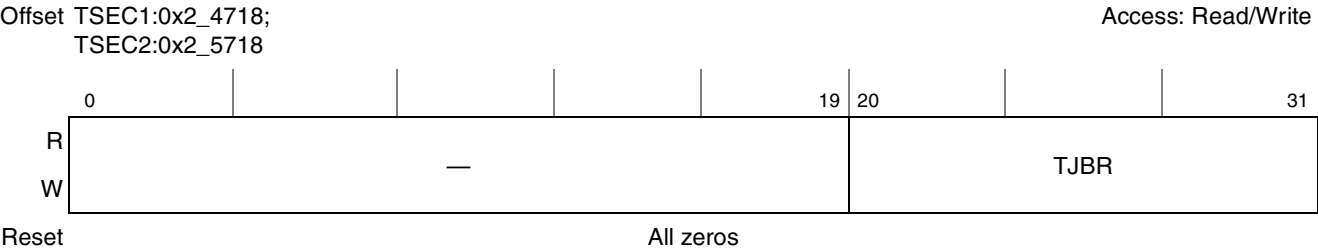
Figure 15-86. Transmit Jabber Frame Counter Register Definition
