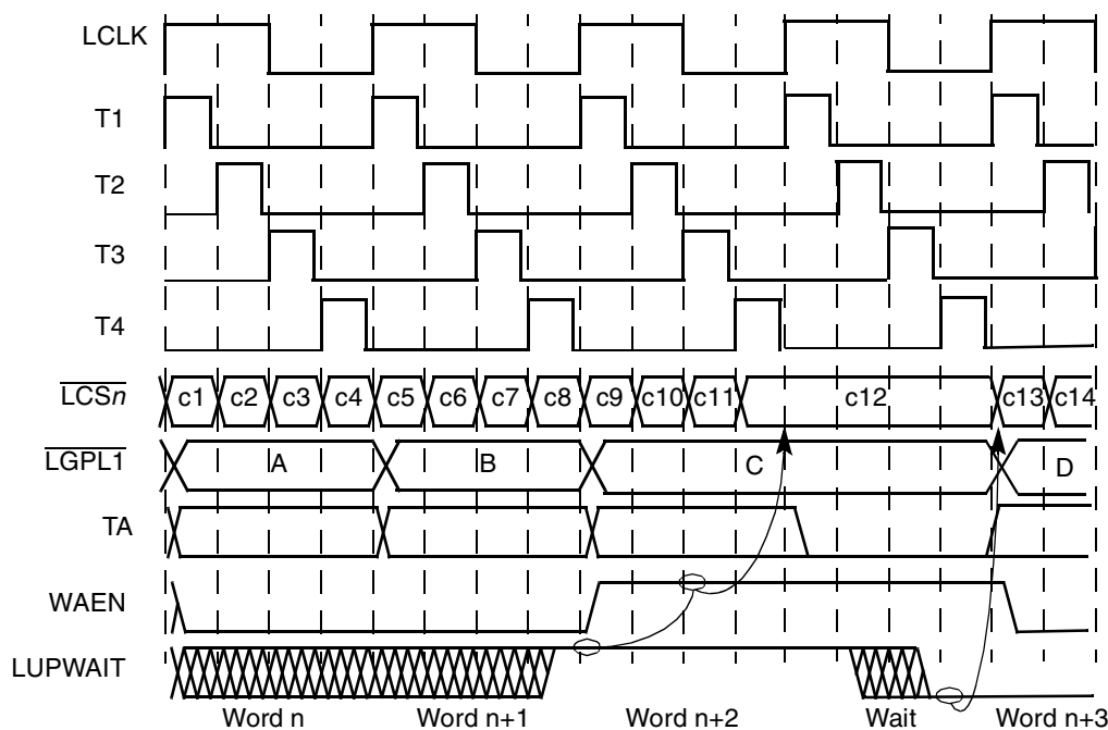
Figure 10-62. Effect of LUPWAIT Signal
