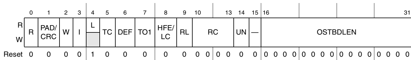
Figure 15-25. OSTBD Register Definition
