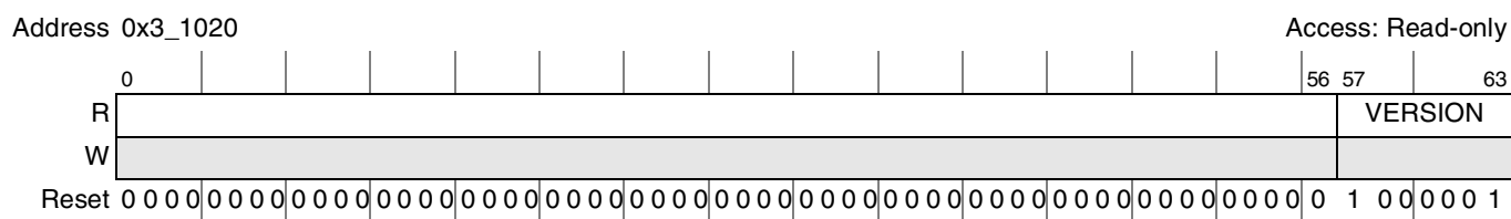
Figure 14-70. ID Register
