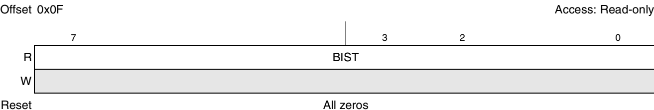
Figure 13-31. BIST Control Configuration Register
