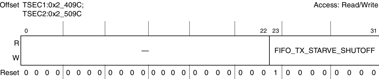
Figure 15-17. FIFO_TX_STARVE_SHUTOFF Register Definition
