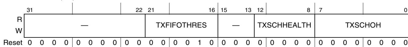
Figure 16-18. Transmit FIFO Tuning Controls (TXFILLTUNING)
