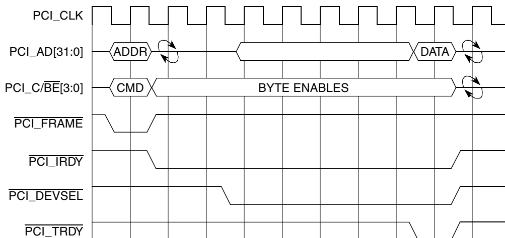
Figure 13-47. Single Beat Read Example
