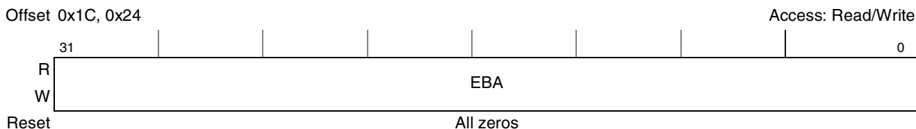
Figure 13-35. GPL Extended Base Address Registers 1–2
