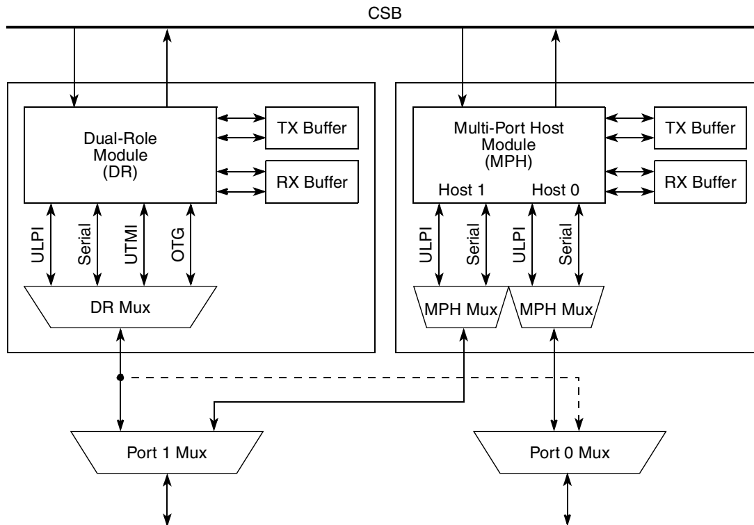
Figure 16-1. USB Interface Block Diagram
