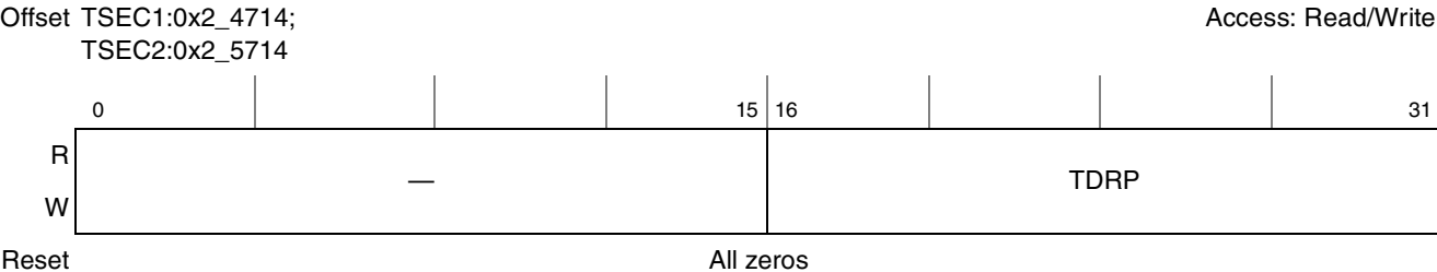
Figure 15-85. Transmit Drop Frame Counter Register Definition
