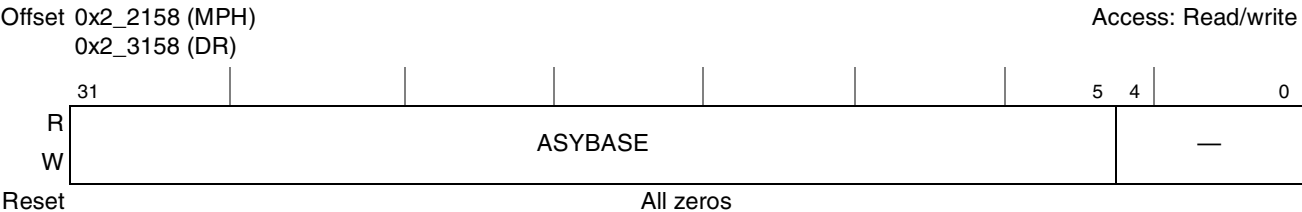
Figure 16-14. Current Asynchronous List Address (ASYNCLISTADDR)
