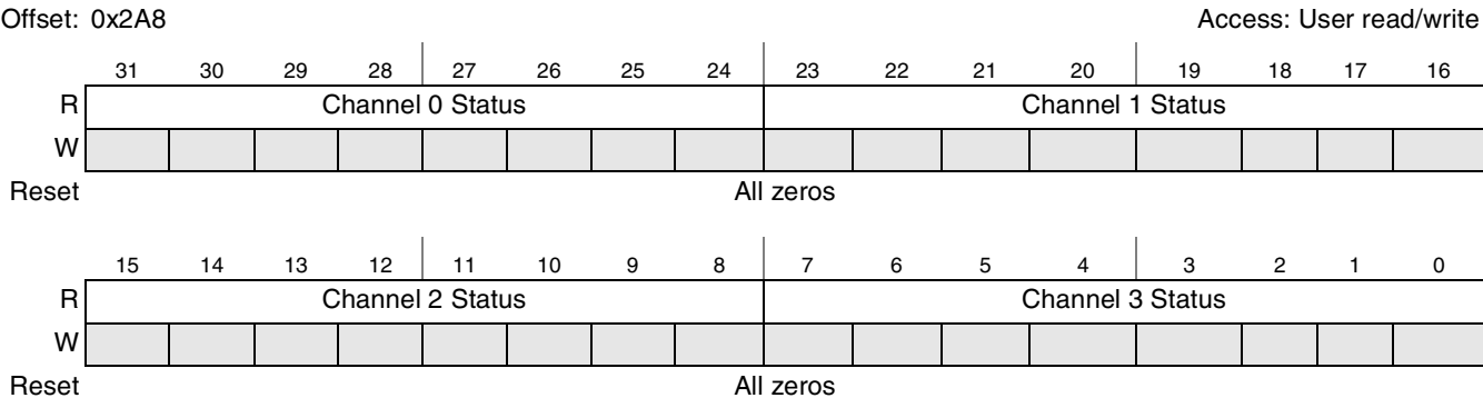
Figure 12-17. DMA General Status Register (DMAGSR)
