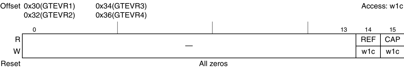
Figure 5-46. Global Timers Event Registers (GTEVR1—GTEVR4)
