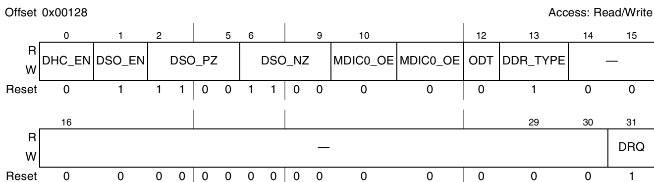
Figure 5-16. DDR Control Driver Register (DDRCDDR)
