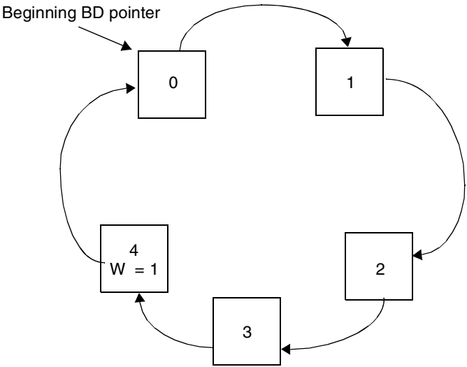
Figure 15-116. Buffer Descriptor Ring
