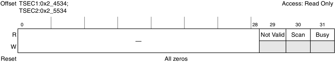
Figure 15-45. MII Management Indicator Register Definition
