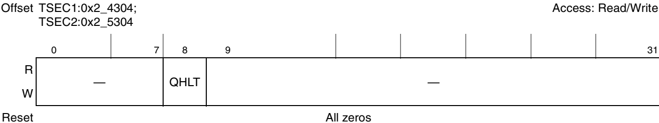
Figure 15-28. RSTAT Register Definition
