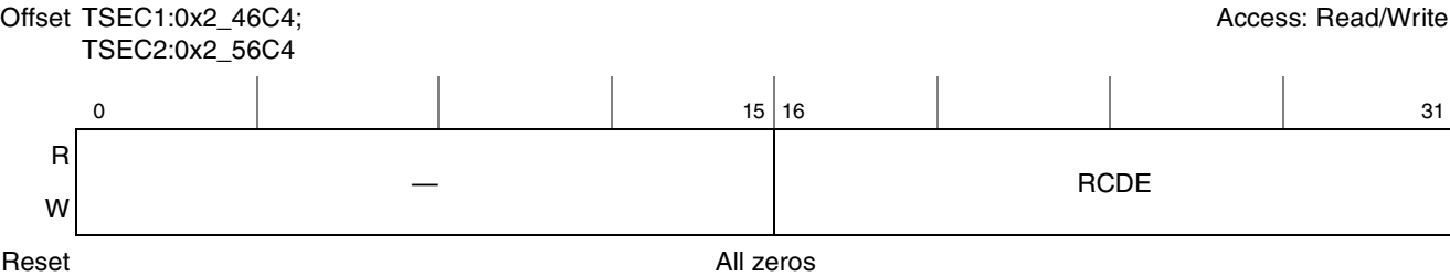
Figure 15-66. Receive Code Error Counter Register Definition
