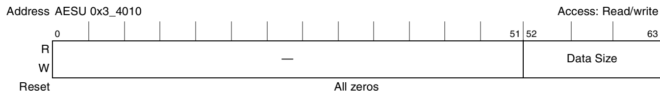
Figure 14-53. AESU Data Size Register
