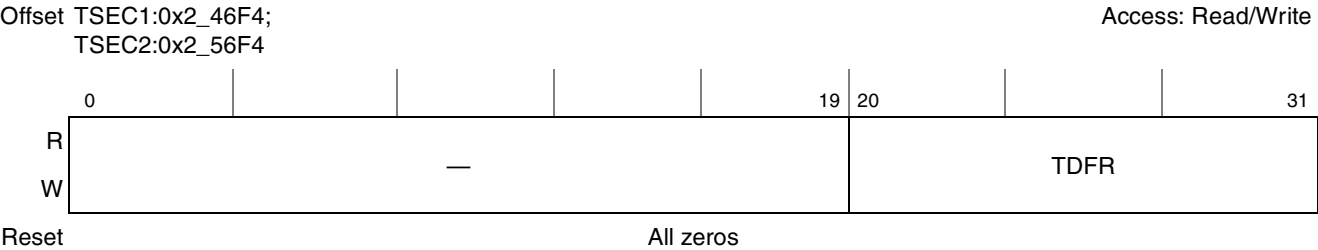
Figure 15-78. Transmit Deferral Packet Counter Register Definition
