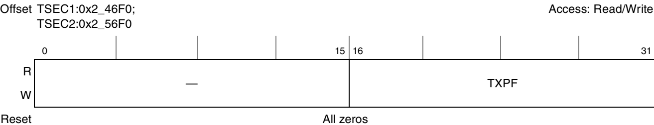
Figure 15-77. Transmit Pause Control Frame Counter Register Definition
