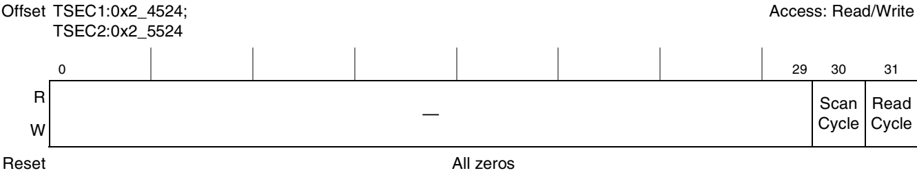
Figure 15-41. MIIMCOM Register Definition
