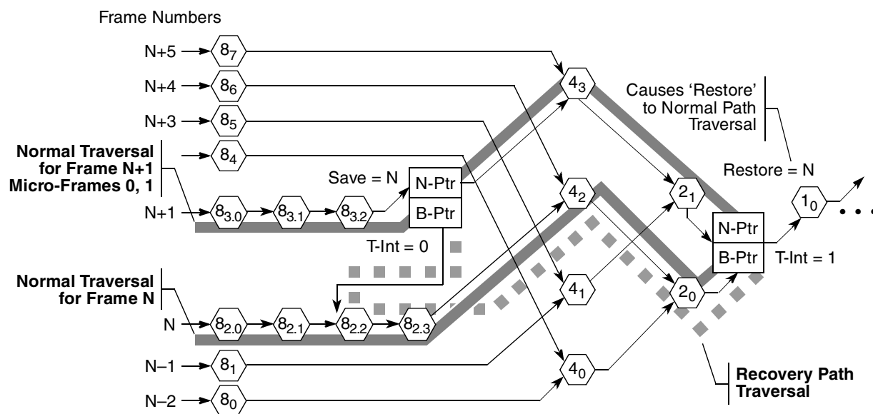
Figure 16-57. Example Host Controller Traversal of Recovery Path via FSTNs
