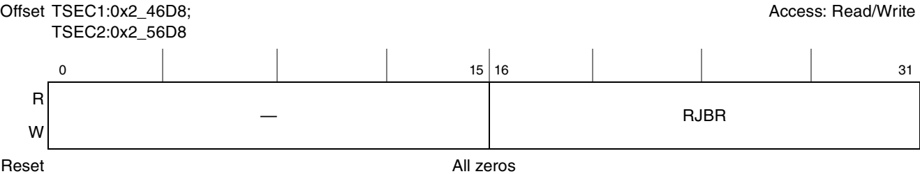
Figure 15-71. Receive Jabber Counter Register Definition
