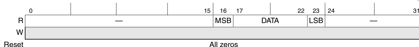
Figure 19-12. Example SPMODE[REV] = 0 SPMODE[LEN] = 7 LSB Sent First
