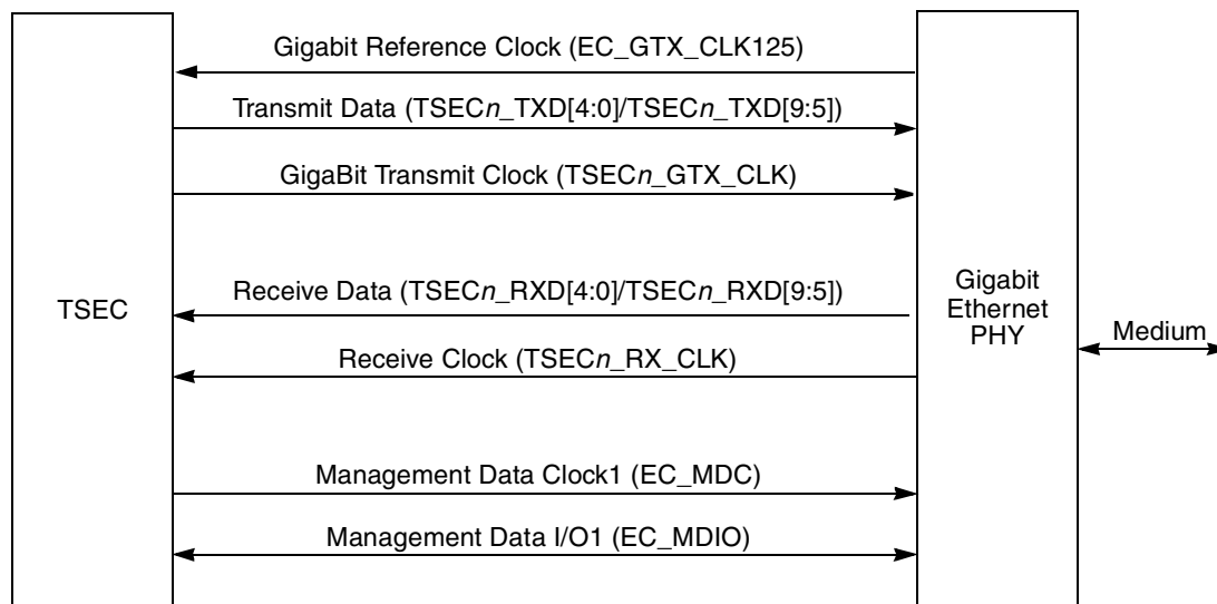
Figure 15-113. TSEC-RTBI Connection
