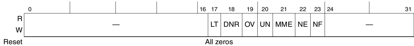
Figure 19-8. SPIM—SPI Mask Register
