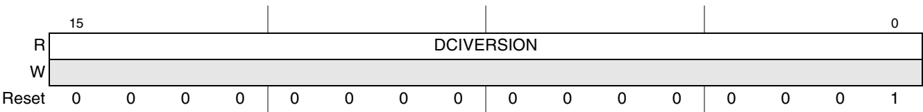
Figure 16-6. Device Interface Version (DCIVERSION)—DR-Only
