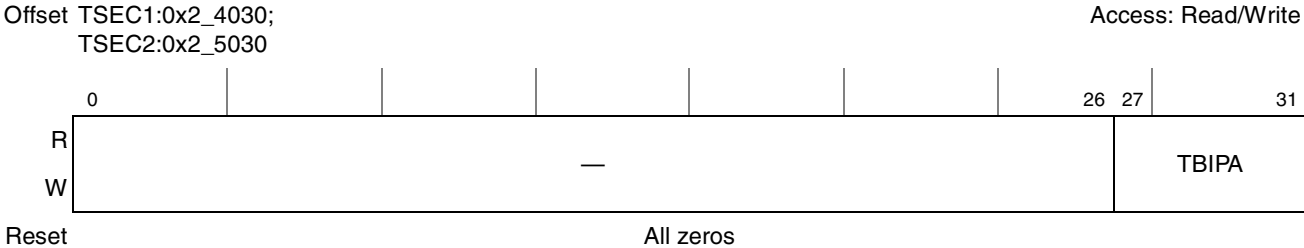
Figure 15-13. TBIPA Register Definition
