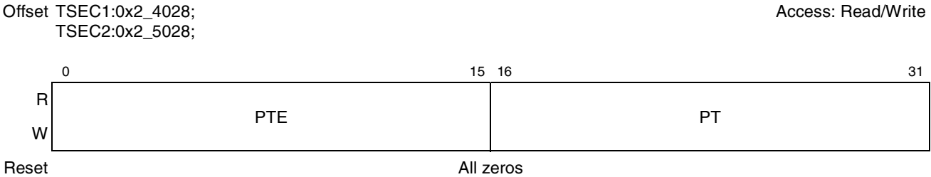
Figure 15-11. PTV Register Definition
