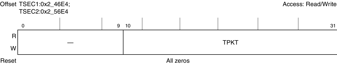
Figure 15-74. Transmit Packet Counter Register Definition
