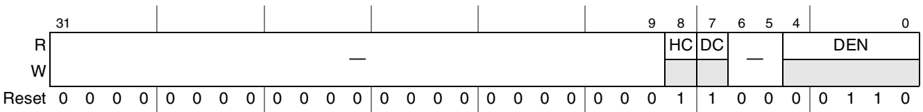
Figure 16-7. Device Control Capability Parameters (DCCPARAMS)—DR-Only
