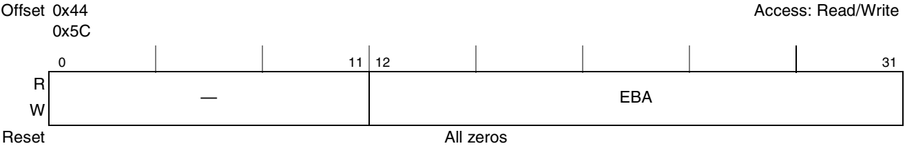
Figure 13-18. PCI Inbound Extended Base Address Registers (PIEBAR n )
