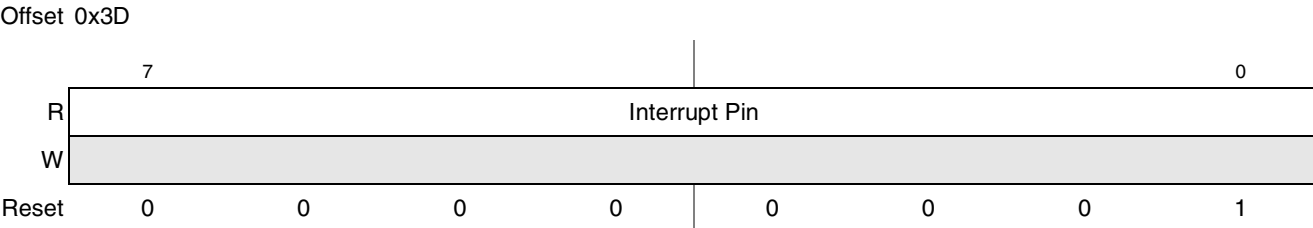
Figure 13-40. Interrupt Pin Register
