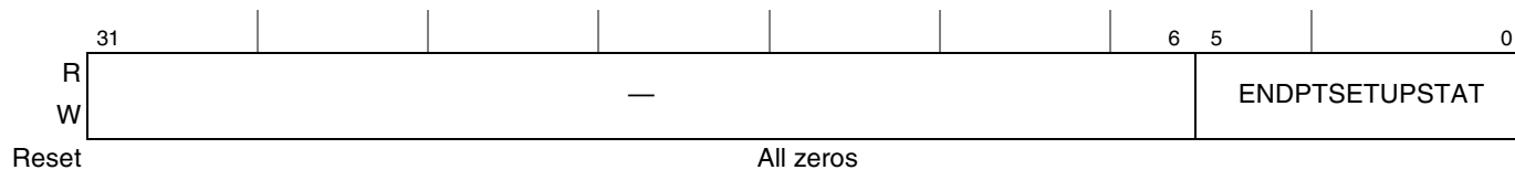
Figure 16-25. Endpoint Setup Status (ENDPTSETUPSTAT)—DR-Only
