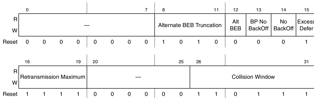
Figure 15-38. Half-Duplex Register Definition
