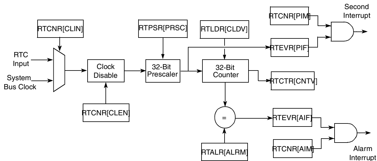
Figure 5-31. Real Time Clock Module Functional Block Diagram
