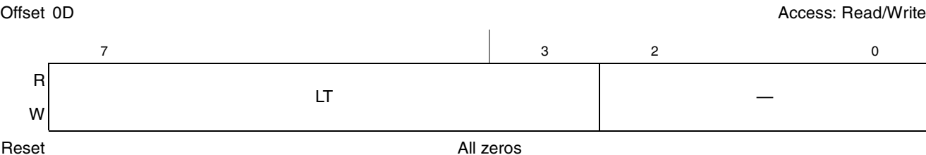
Figure 13-29. Latency Timer Configuration Register
