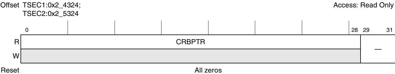
Figure 15-31. CRBPTR Register Definition
