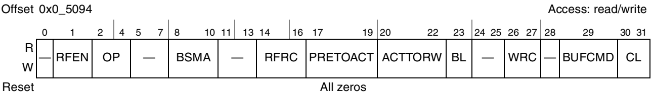
Figure 10-10. Local Bus SDRAM Machine Mode Register (LSDMR)
