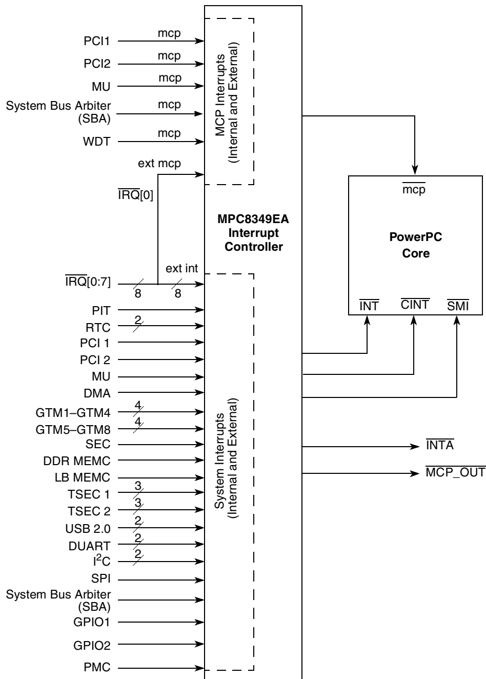
Figure 8-25. Interrupt Structure
