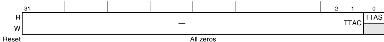
Figure 16-16. TT Asynchronous Buffer Status (ASYNCTTSTS)—MPH-Only
