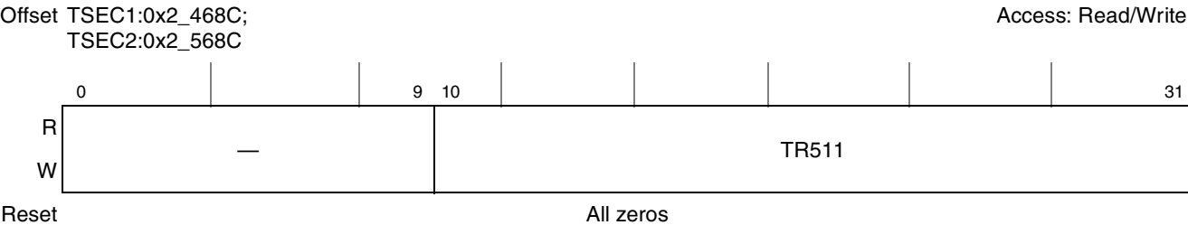
Figure 15-52. Transmit and Received 256- to 511-Byte Frame Register Definition
