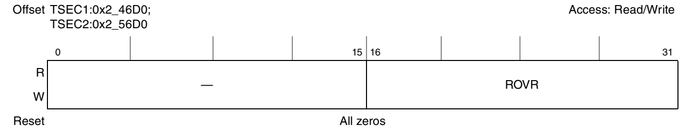
Figure 15-69. Receive Oversize Packet Counter Register Definition
