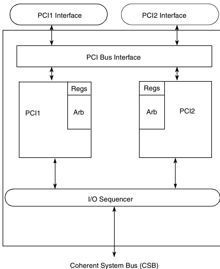
Figure 13-1. PCI Controller Block Diagram
