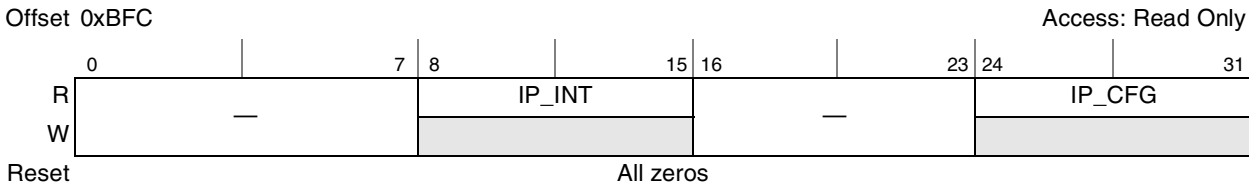
Figure 9-18. DDR IP Block Revision 2 (DDR_IP_REV2)
