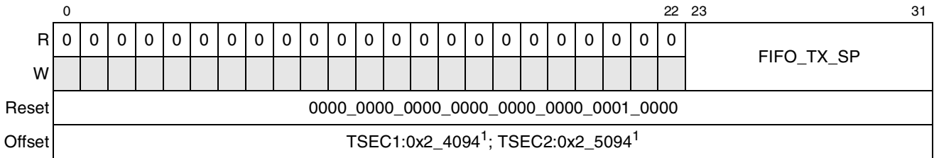
Figure 15-15. FIFO_TX_SP Register Definition
