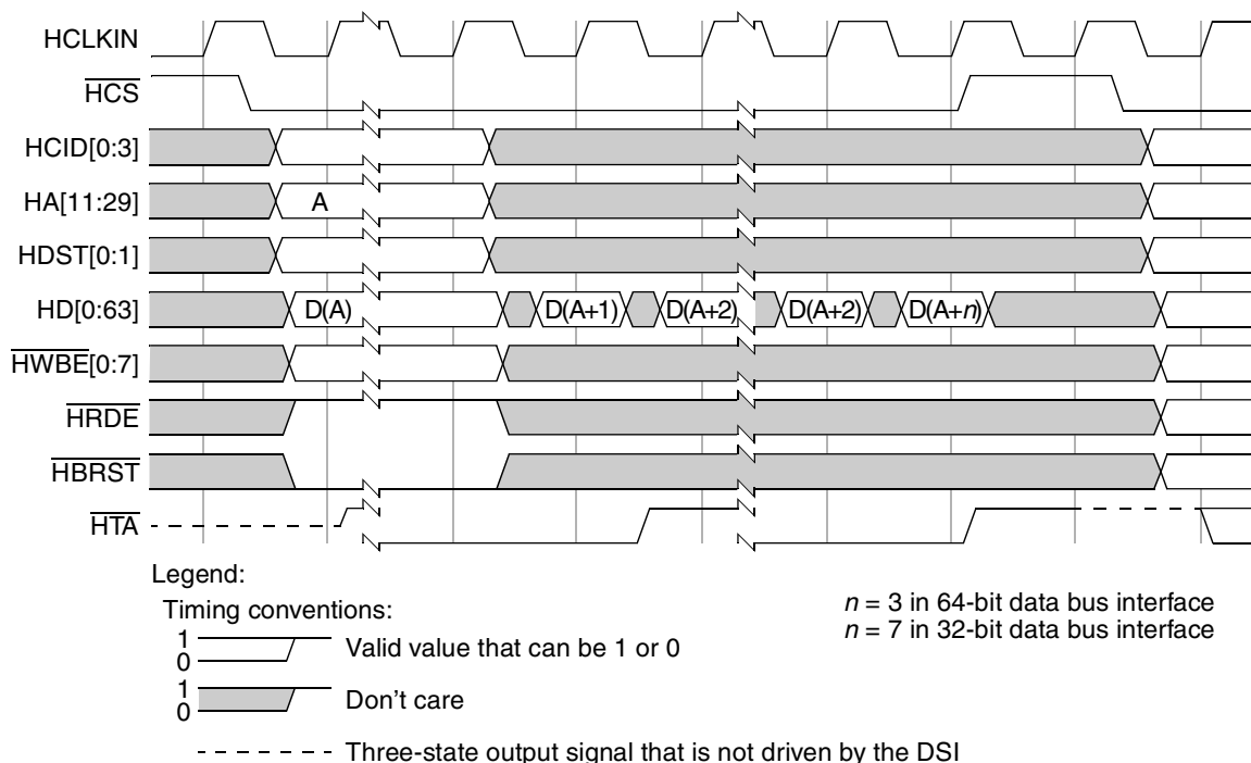
Figure 10-84. Synchronous Burst Write to MSC8122 DSI
