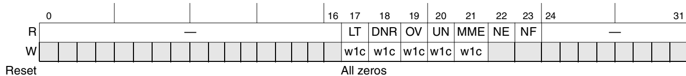
Figure 19-7. SPIE—SPI Event Register
