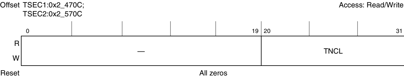
Figure 15-84. Transmit Total Collision Counter Register Definition
