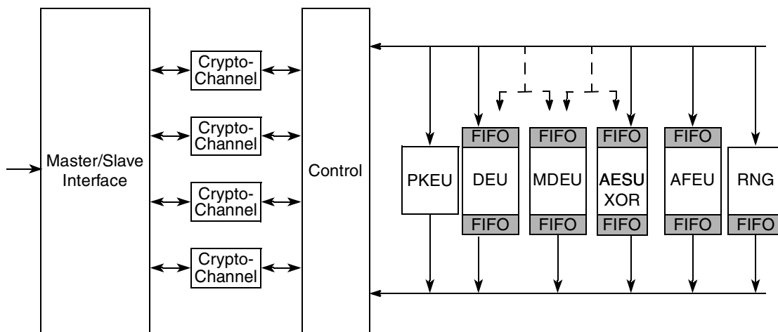
Figure 1-3. Integrated Security Engine Functional Blocks
