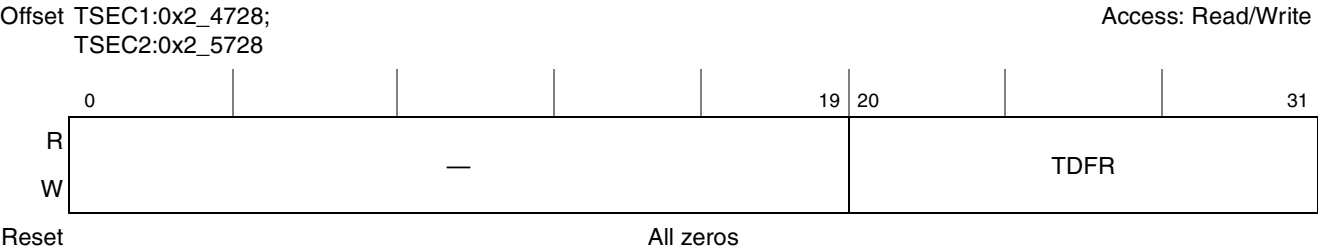
Figure 15-90. Transmit Undersize Frame Counter Register Definition
