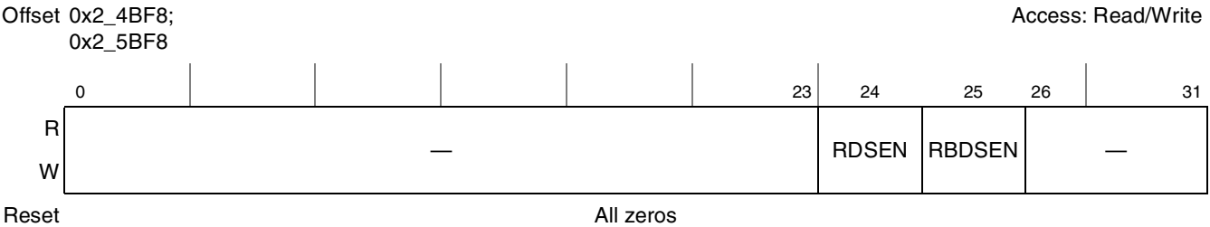
Figure 15-98. ATTR Register Definition
