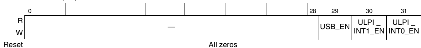
Figure 16-36. Control (CONTROL)
