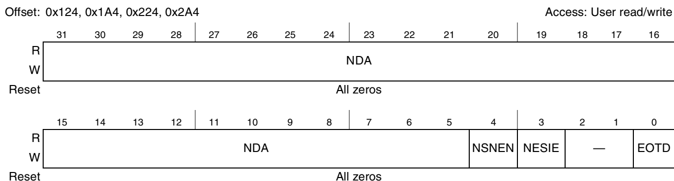
Figure 12-16. DMA Next Descriptor Address Register (DMANDAR n )
