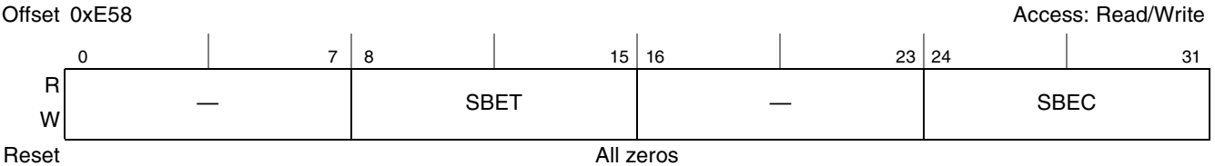
Figure 9-30. Single-Bit ECC Memory Error Management Register (ERR_SBE)
