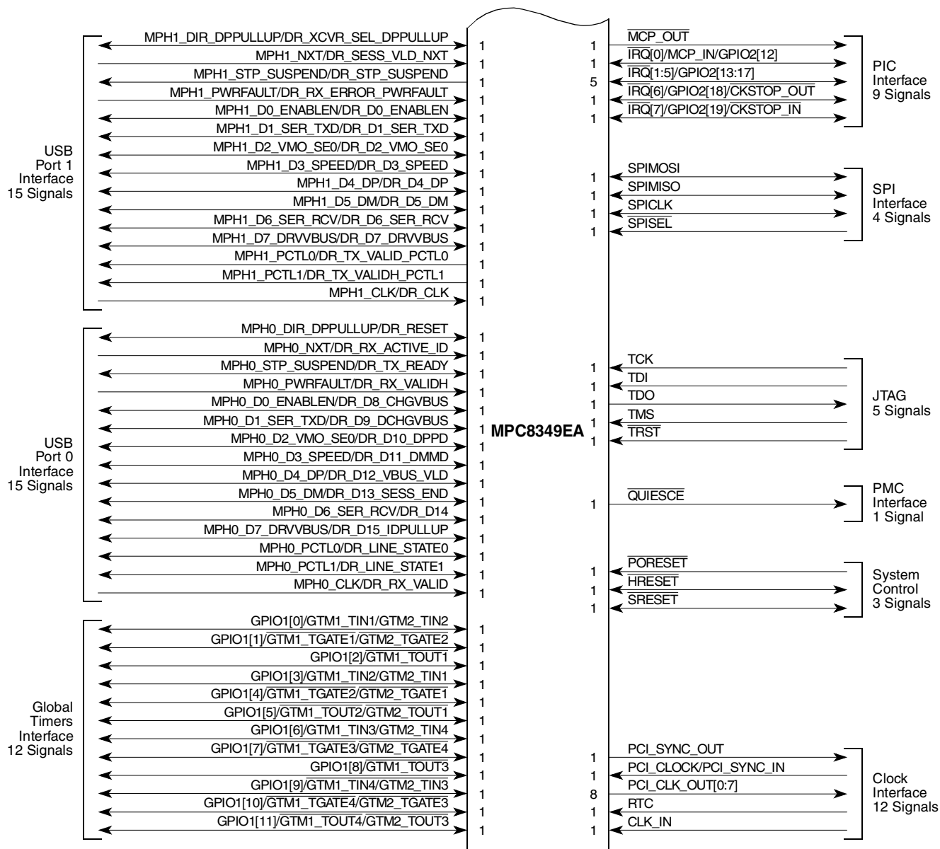
Figure 3-2. MPC8349EA Signal Groupings (2 of 2)
