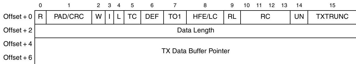
Figure 15-117. Transmit Buffer Descriptor
