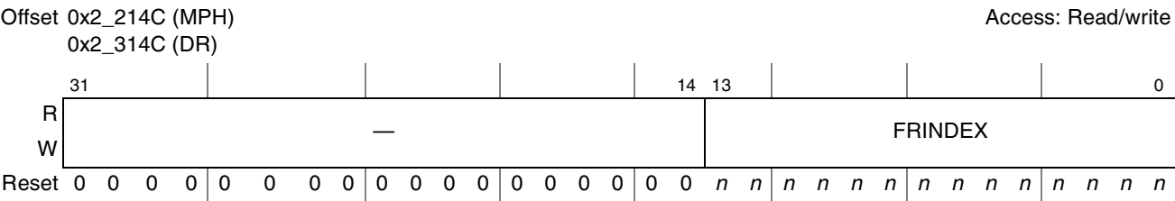
Figure 16-11. USB Frame Index (FRINDEX)
