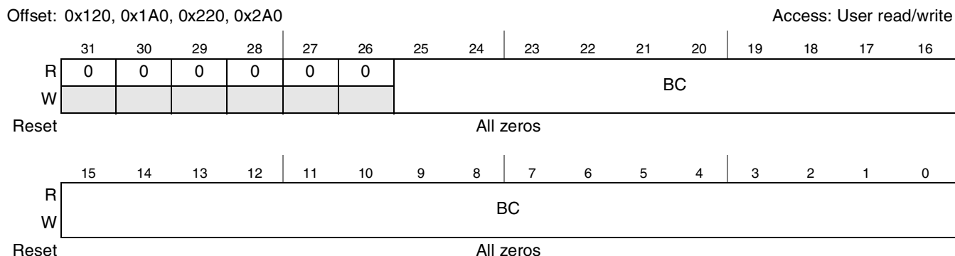
Figure 12-15. DMA Byte Count Register (DMABCR n )
