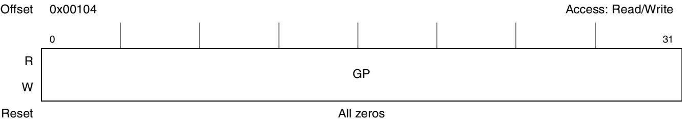
Figure 5-11. System General Purpose Register High (SGPRH)
