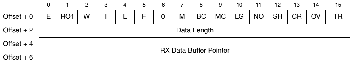
Figure 15-118. Receive Buffer Descriptor
