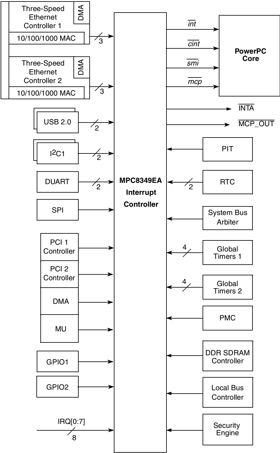
Figure 8-1. Interrupt Sources Block Diagram
