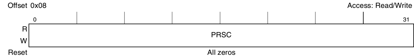
Figure 5-35. Periodic Interval Timer Prescale Register (PTPSR)
