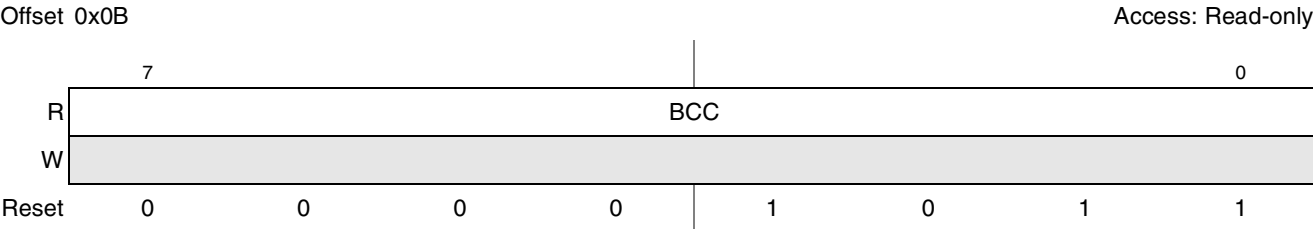
Figure 13-27. Base Class Code Configuration Register
