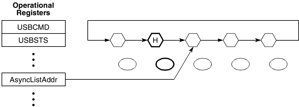
Figure 16-46. General Format of Asynchronous Schedule List
