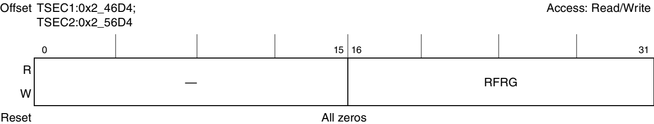
Figure 15-70. Receive Fragments Counter Register Definition
