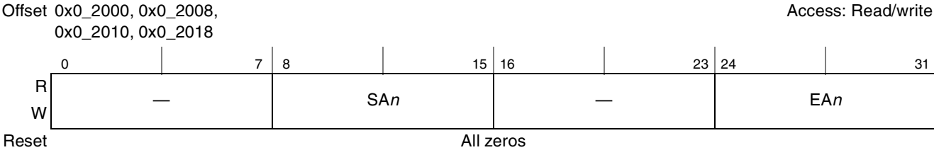
Figure 9-2. Chip Select Bounds Registers (CS n _BNDS)
