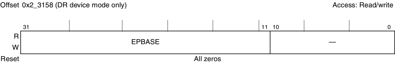
Figure 16-15. Endpoint List Address (ENDPOINTLISTADDR)—DR-Only
