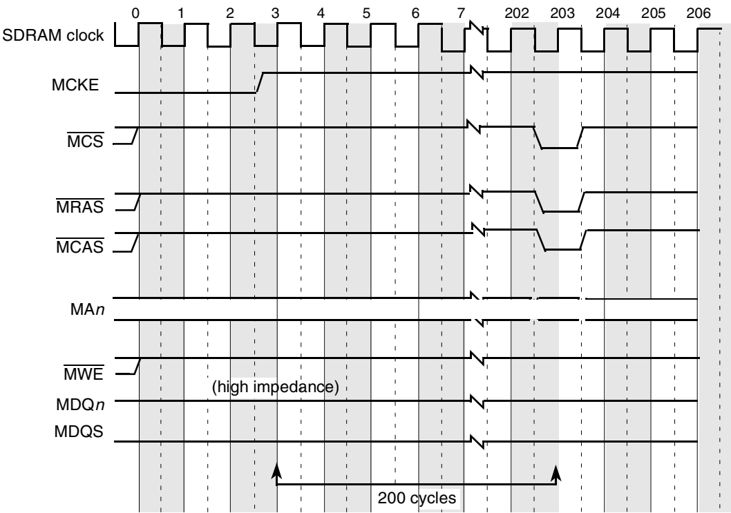
Figure 9-45. DDR SDRAM Self-Refresh Exit Timing
