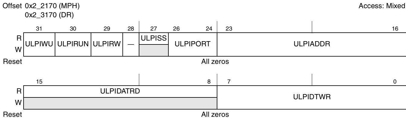
Figure 16-20. ULPI Register Access (ULPI VIEWPORT)
