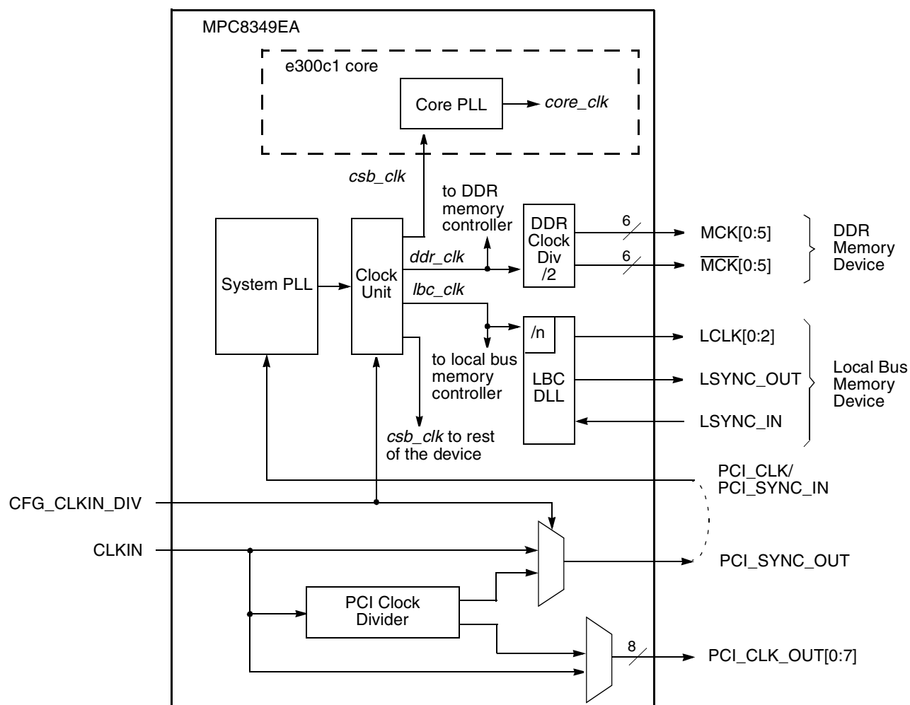
Figure 4-9. Clock Subsystem Block Diagram
