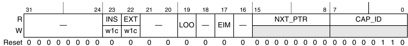
Figure 13-45. Hot Swap Register Block
