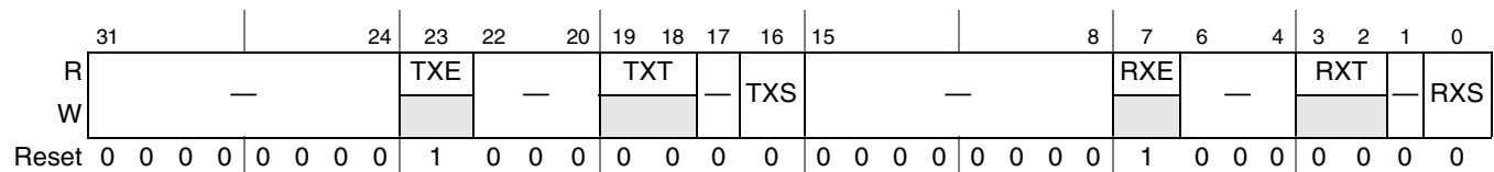
Figure 16-30. Endpoint Control 0 (ENDPTCTRL0)—DR-Only
