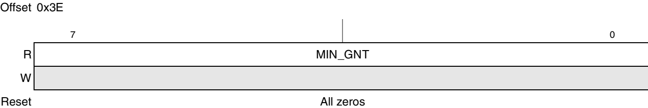
Figure 13-41. Minimum Grant Configuration Register
