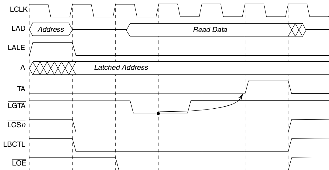
Figure 10-32. External Termination of GPCM Access
