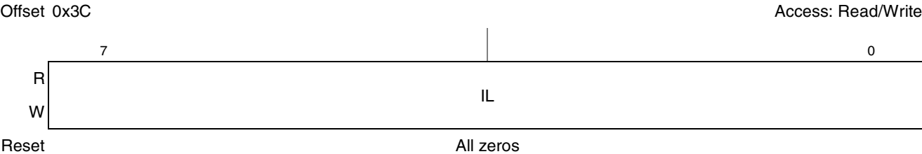
Figure 13-39. Interrupt Line Configuration Register
