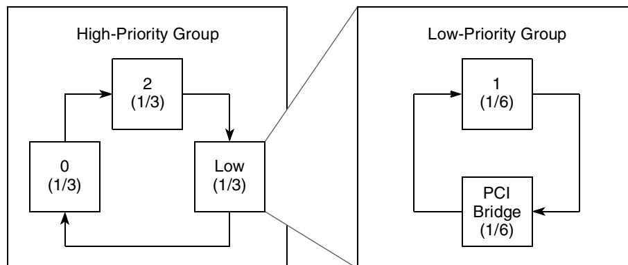
Figure 13-46. PCI Arbitration Example
