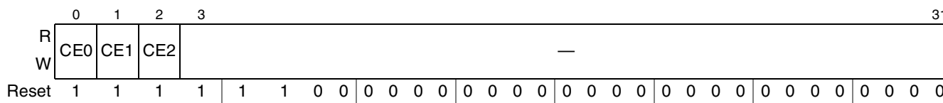
Figure 22-5. DLL Clock Register
