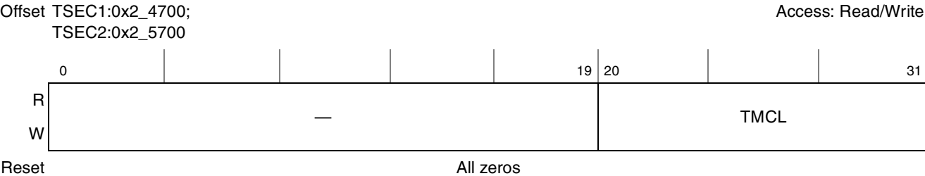
Figure 15-81. Transmit Multiple Collision Packet Counter Register Definition
