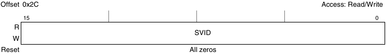
Figure 13-36. Subsystem Vendor ID Configuration Register
