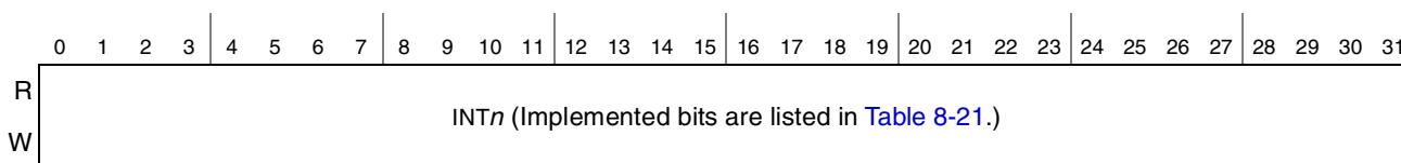
Figure 8-17. System Error Mask Register (SERMR)
