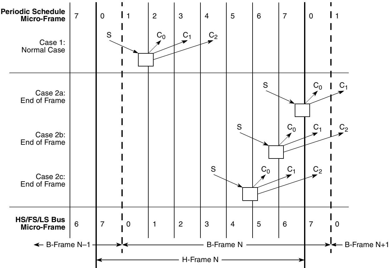
Figure 16-55. Split Transaction, Interrupt Scheduling Boundary Conditions
