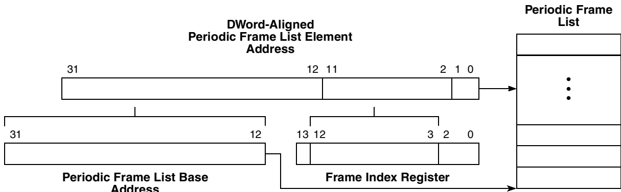
Figure 16-45. Derivation of Pointer into Frame List Array
