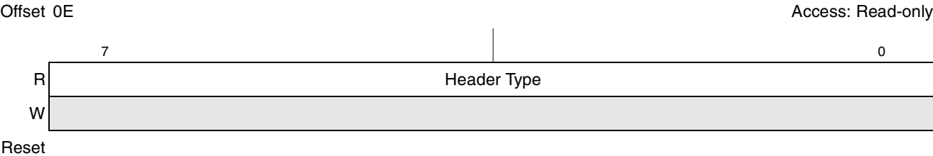
Figure 13-30. Header Type Configuration Register
