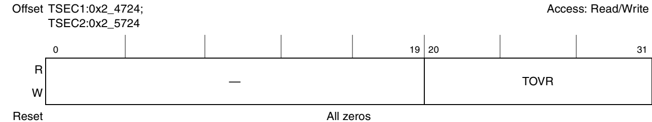
Figure 15-89. Transmit Oversized Frame Counter Register Definition
