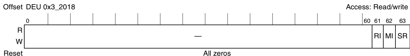
Figure 14-20. DEU Reset Control Register (DEURCR)
