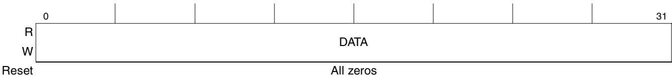
Figure 19-10. SPI Transmit Data Hold Register
