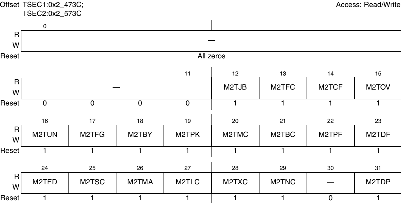
Figure 15-95. Carry Mask Register 2 (CAM2) Register Definition
