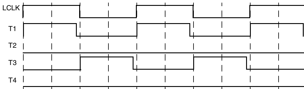
Figure 10-55. UPM Clock Scheme for LCRR[CLKDIV] = 2
