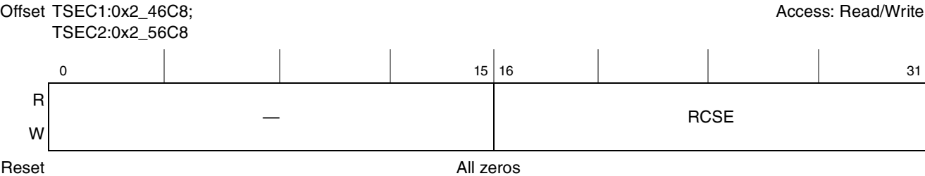
Figure 15-67. Receive Carrier Sense Error Counter Register Definition
