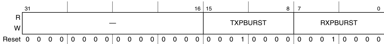
Figure 16-17. Master Interface Data Burst Size (BURSTSIZE)
