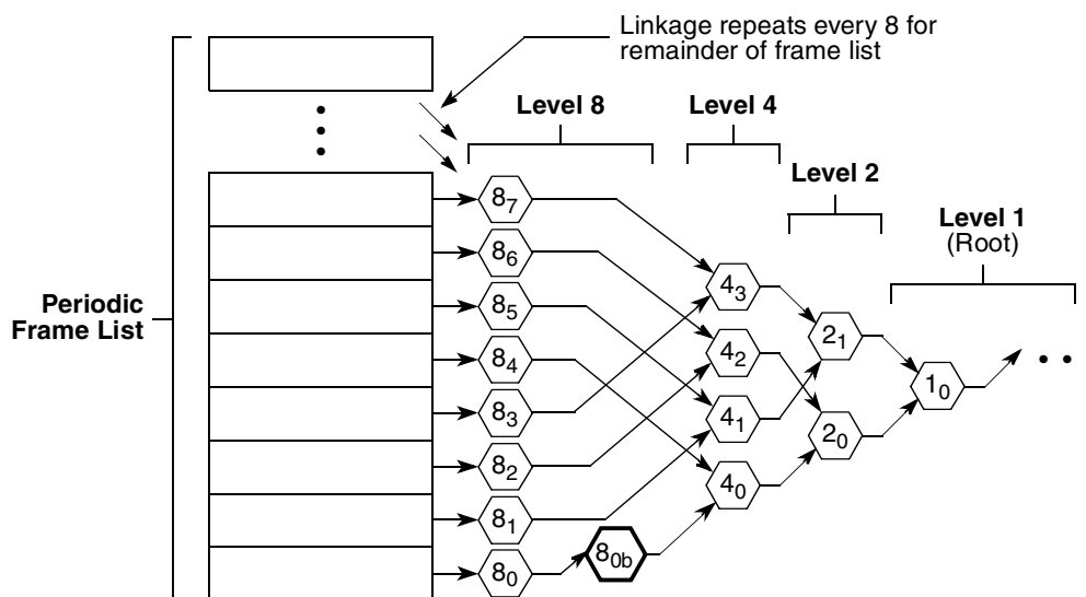
Figure 16-56. General Structure of EHCI Periodic Schedule Utilizing Interrupt Spreading
