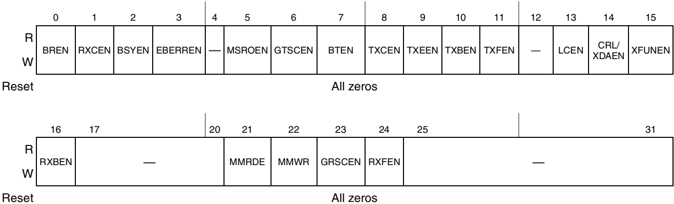
Figure 15-7. IMASK Register Definition
