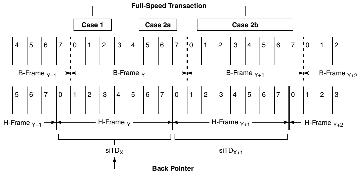
Figure 16-60. siTD Scheduling Boundary Examples
