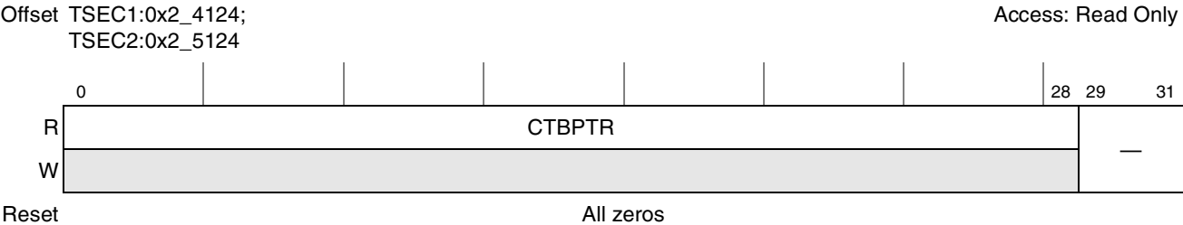
Figure 15-22. CTBPTR Register Definition
