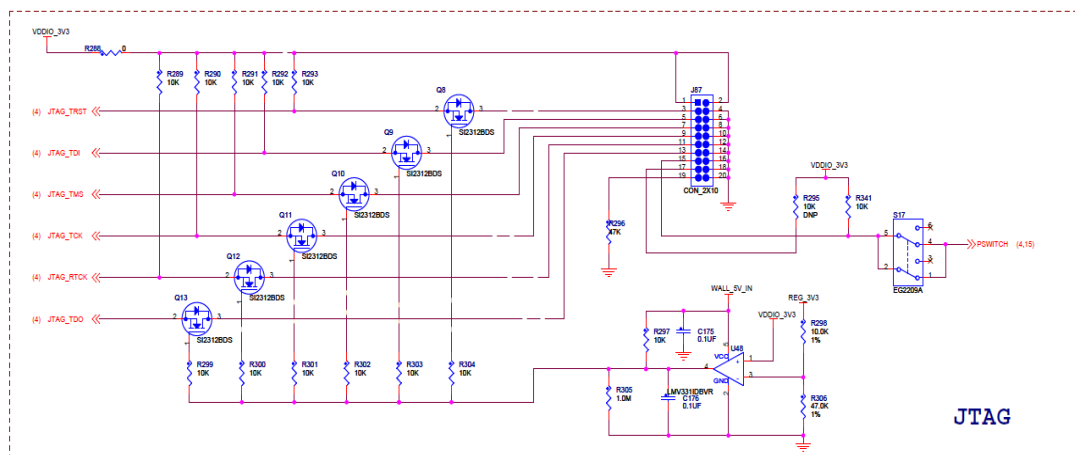
Figure 2-18 JTAG Schematic Drawing
