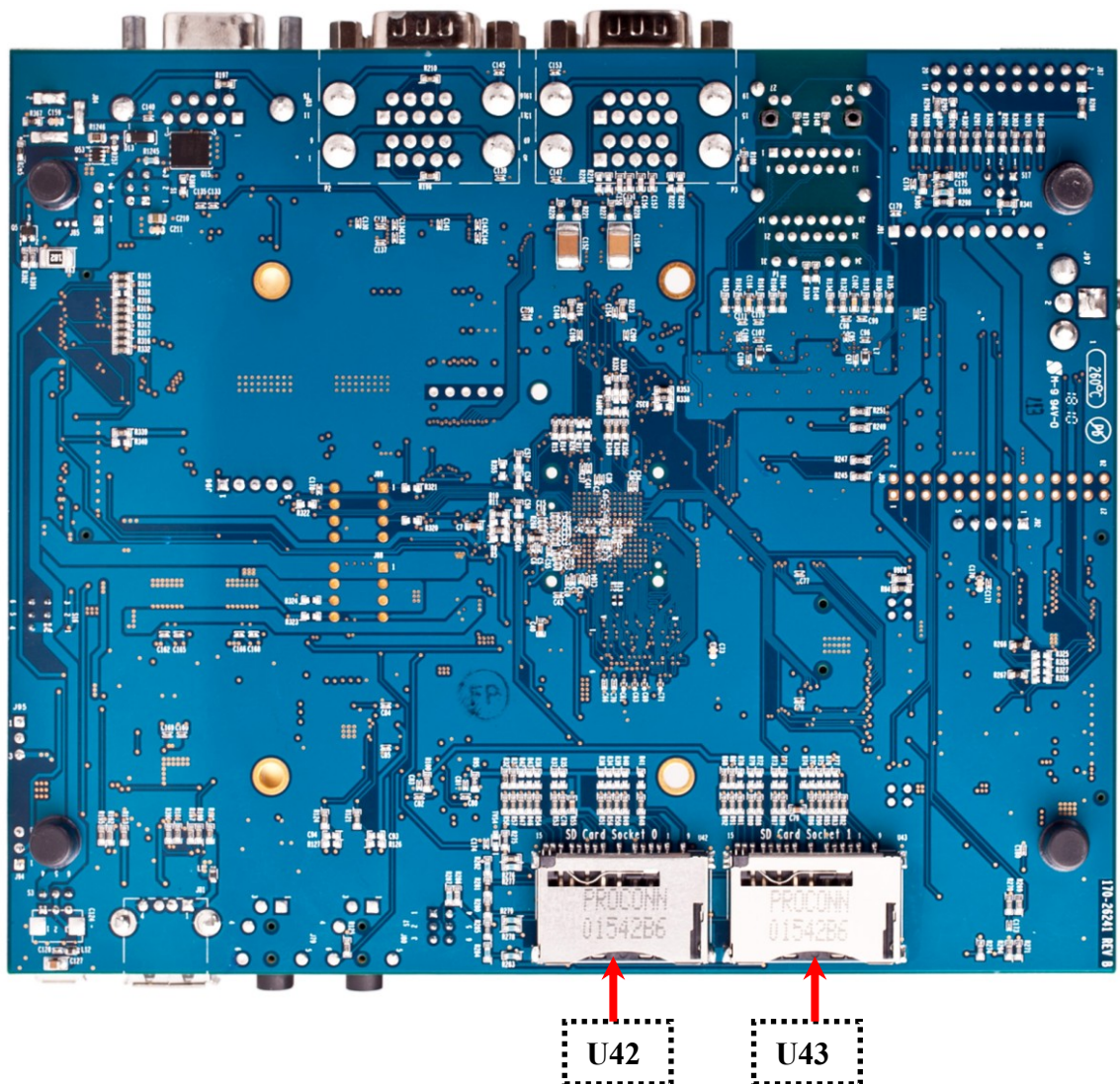
Figure 2-20 Interface Connectors
