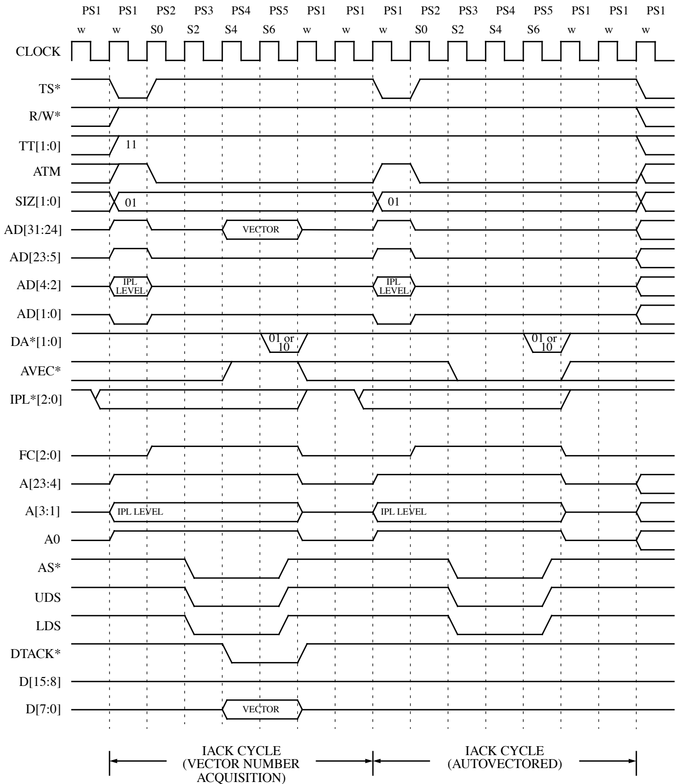
Figure 3: Interrupt-Acknowledge Operation
